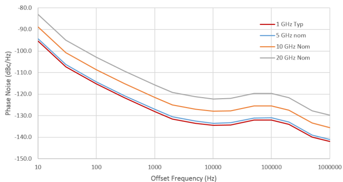
Phase Noise
