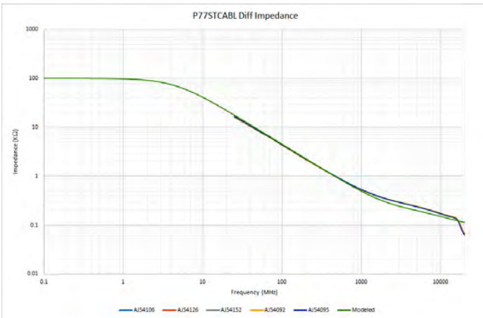
Figure 7: P77STCABL differential impedance
