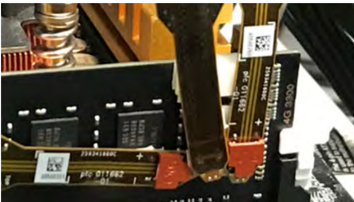
Figure 2: P77STFLXB solder down, flex-circuit accessory provides a probing solution for DDR4 and LPDDR4 electrical validation when used with Nexus XH Series Interposers.
