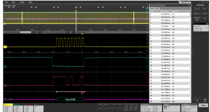
Performing bus decode analysis and generating results table
