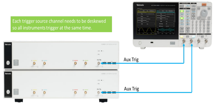
Figure 6: Setup diagram to quickly achieve moderate skew among channels
