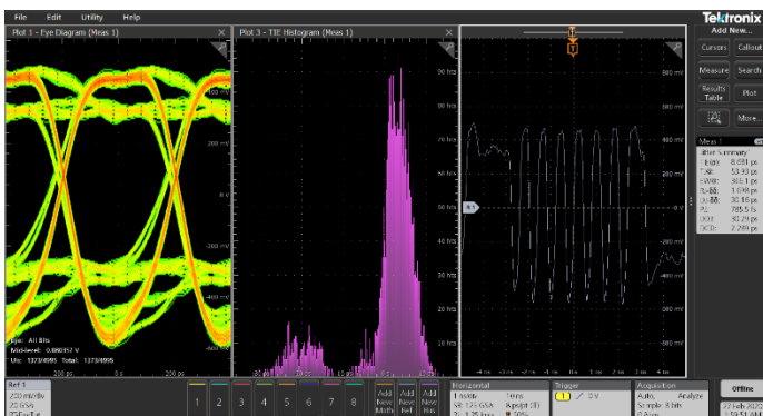
Figure 13: Side-by-side view of eye diagram, TIE histogram and waveform shown in individual views
