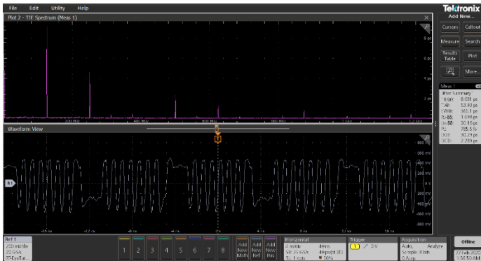
Figure 12: Stacked view of time domain waveform and jitter spectrum
