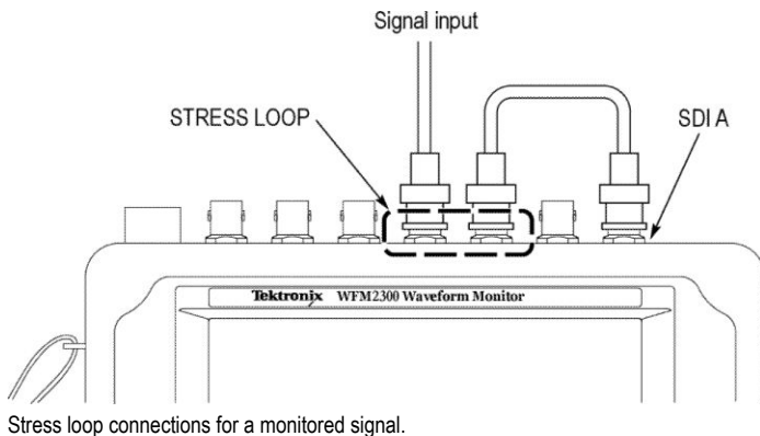
Stress loop connections for a monitored signal.
