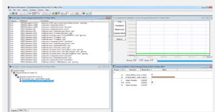
Offline multiplexer provides support for manipulating H.265 (HEVC) and H.264/AVC content into Transport Streams
