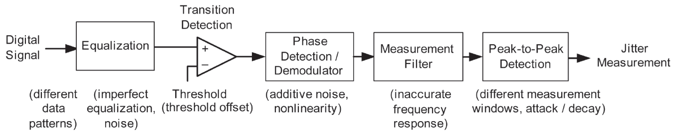
► Figure 16. The functions involved in jitter measurement (Causes of measurement discrepancies are indicated in parentheses).
