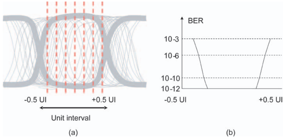
▶ Figure 11. Bathtub curve – BER vs. location in Eye Diagram.
