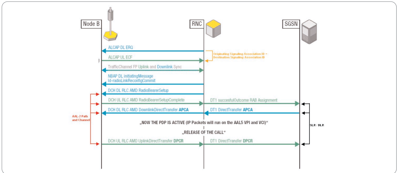
► Figure 13. Mobile Originating PDP-Context Activation and Deactivation.
