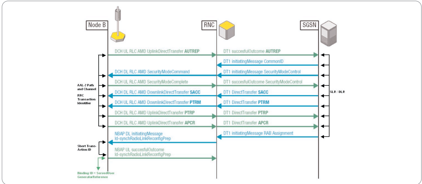
► Figure 12. Mobile Originating PDP-Context Activation and Deactivation.
