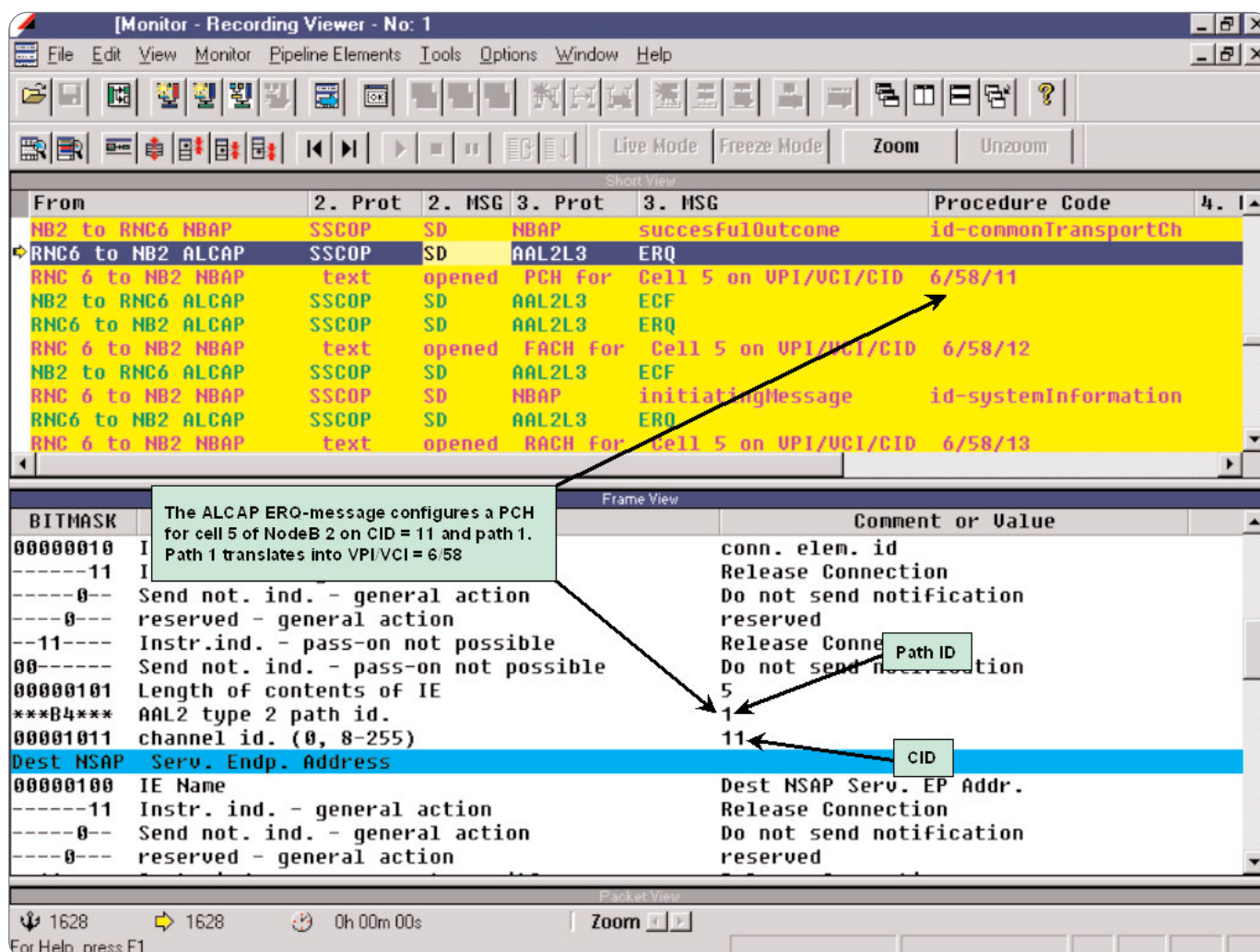
► Figure 2. Extract of a Cell Configuration, recorded by Tektronix Protocol tester on an Iub-interface.
