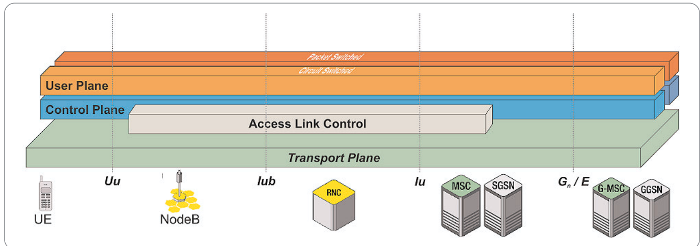
► Figure 1. An Abstract View at the UMTS Protocol Stack.
