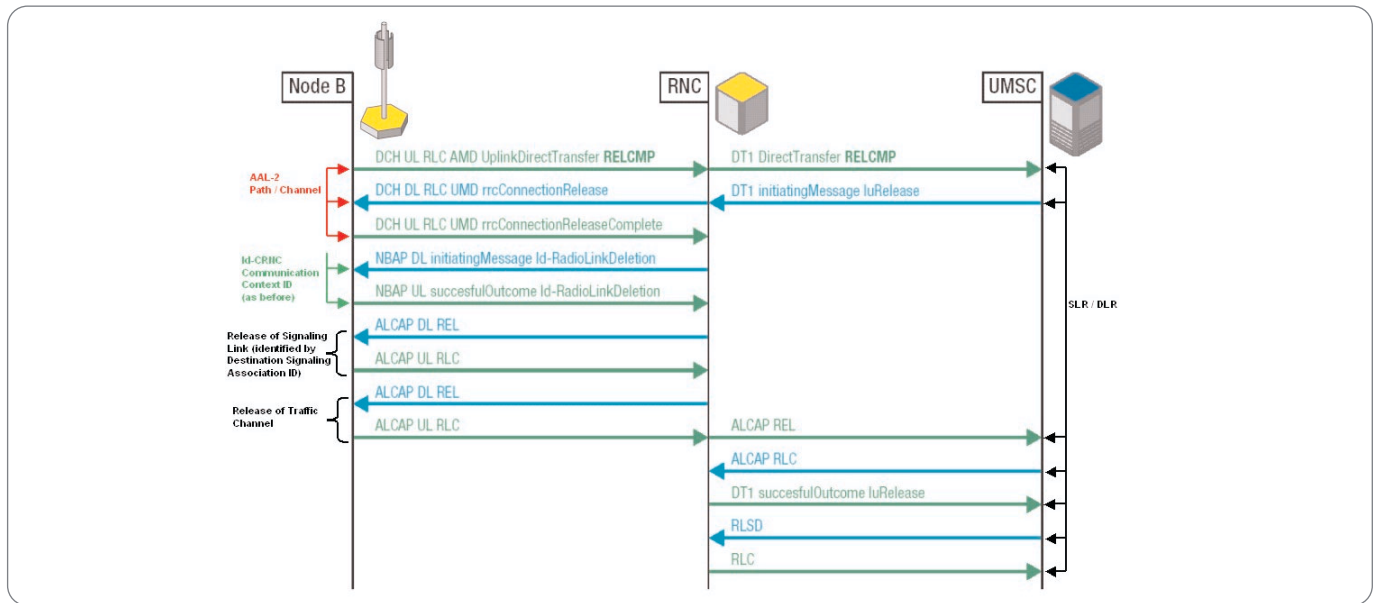
► Figure 10. Mobile Oriented Call.
