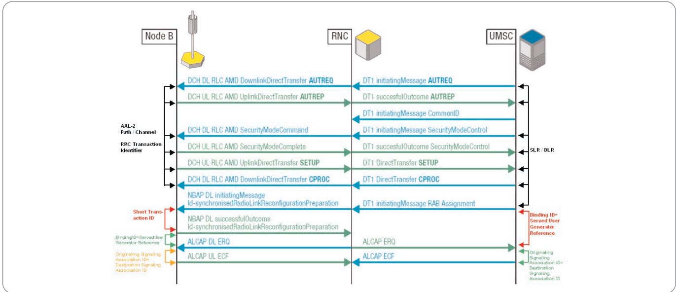
► Figure 8. Mobile Oriented Call.
