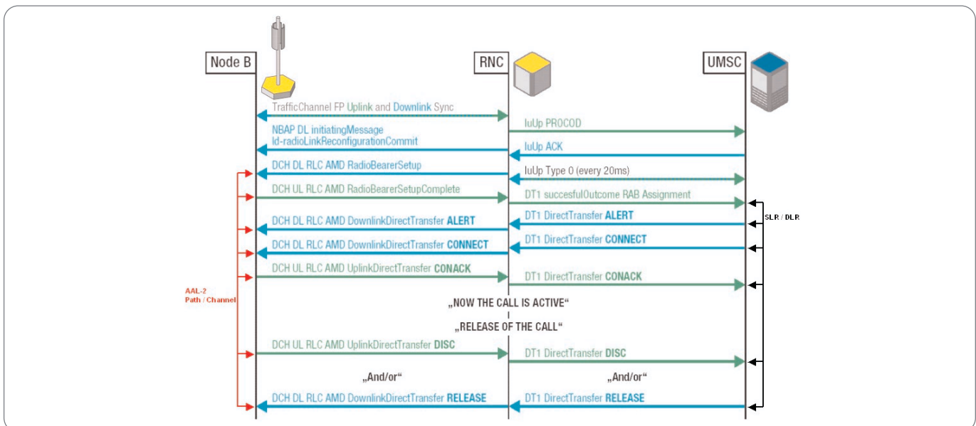
► Figure 9. Mobile Oriented Call.
