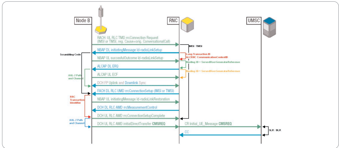
► Figure 7. Mobile Oriented Call.
