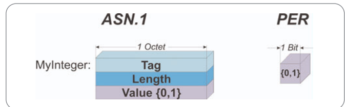
► Figure 4. The Impact of Applying PER on a Mandatory Parameter "MyInteger" ( \Leftrightarrow example).
