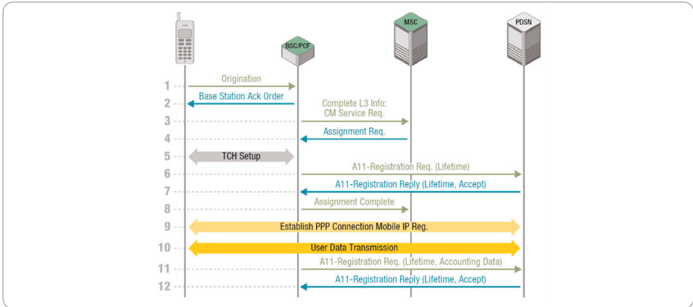
► Figure 2. Setting up a cdma2000 1X mobile data call.
