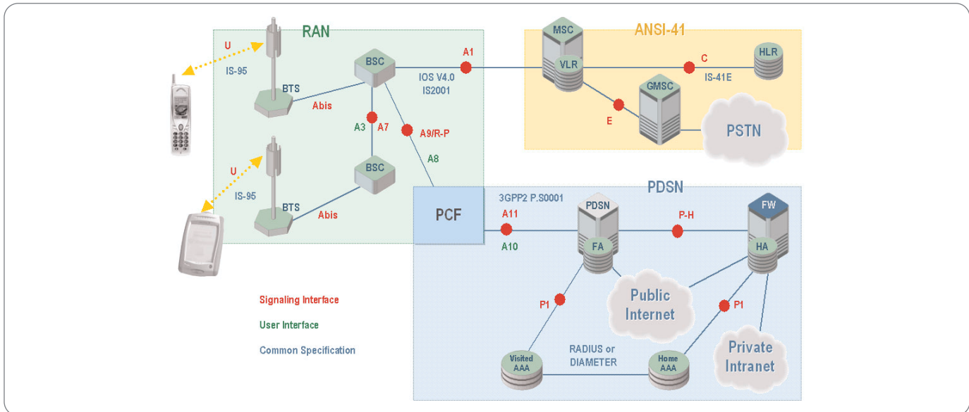
► Figure 1. The structure of a CDMA network.
