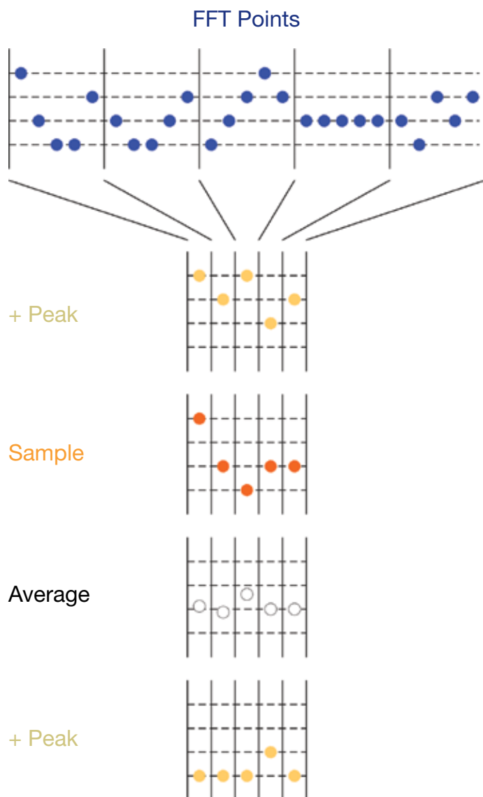
Figure 14. Detection Methods for creating spectrum traces.
