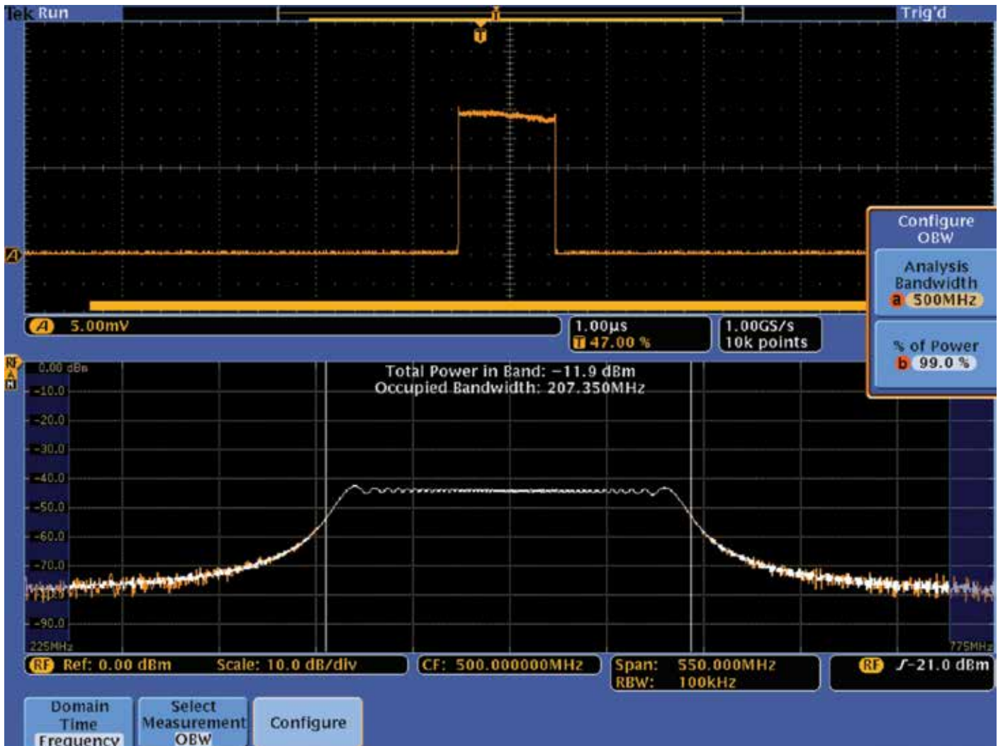
Figure 23. OBW Measurement.
