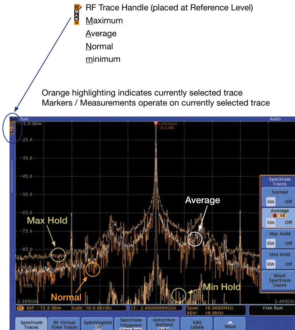
Figure 13. Spectrum Traces.
