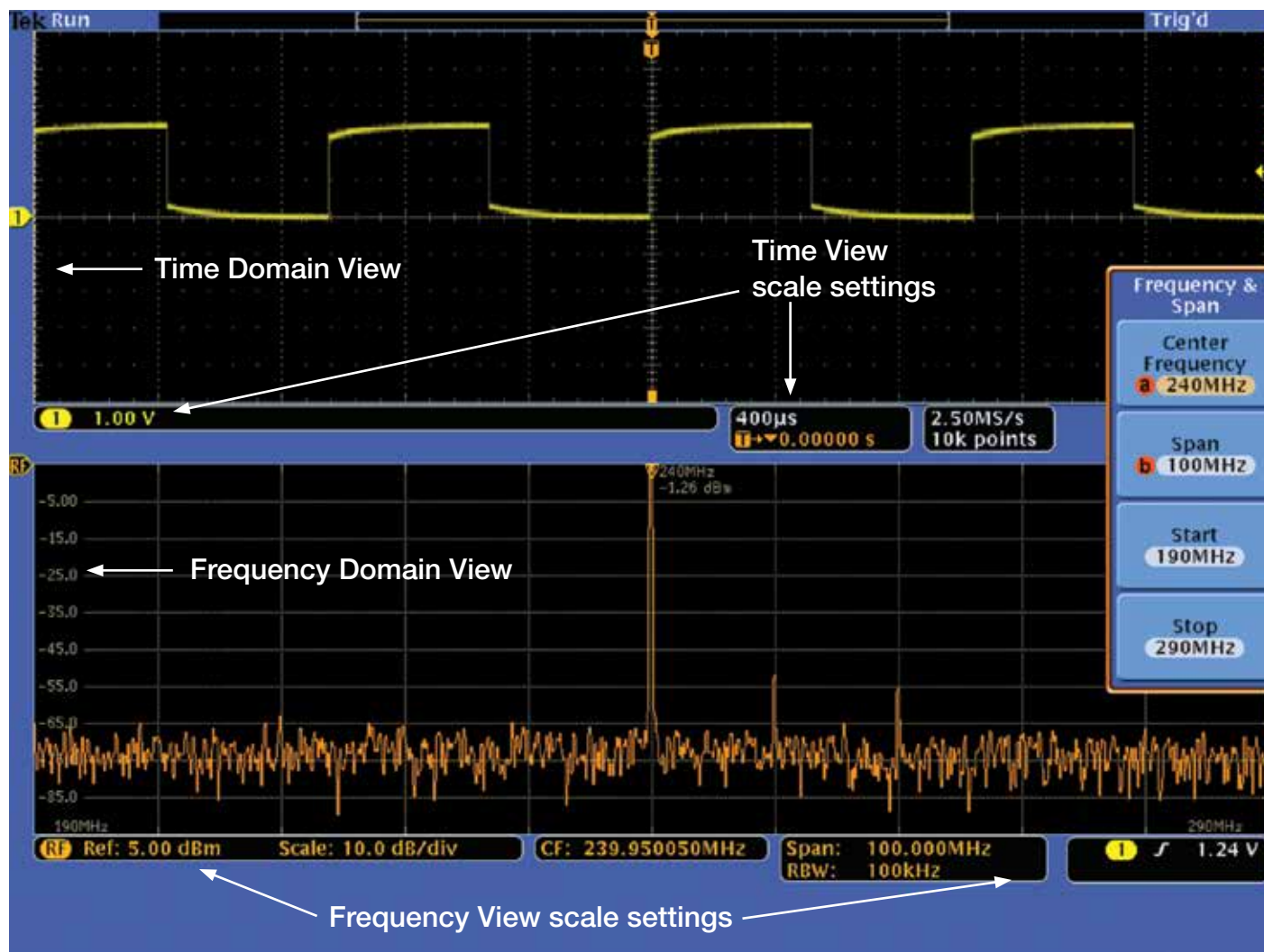
Figure 6. MDO4000B Display Overview for Time and Frequency Domain Views.
