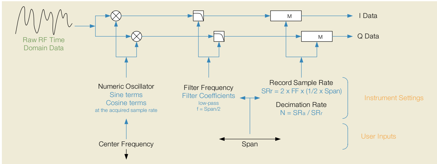
Figure 39. Generating IQ Data.
