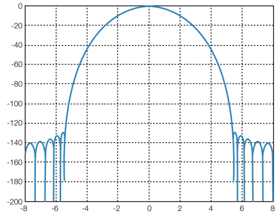
Figure A4. The spectrum of a Kaiser window. The horizontal scale unit is frequency bin ( F^\circ/N ). The Vertical scale is in dB.
