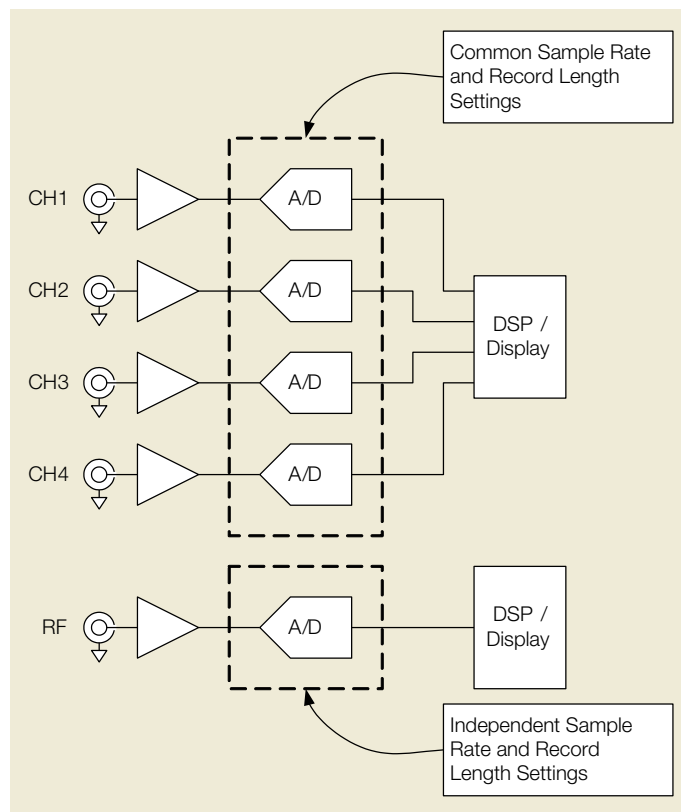
Figure 4. MDO4000B Simplified Acquisition system.
