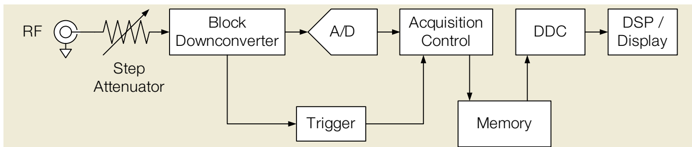
Figure 32. Simplified MDO4000B Block Diagram.
