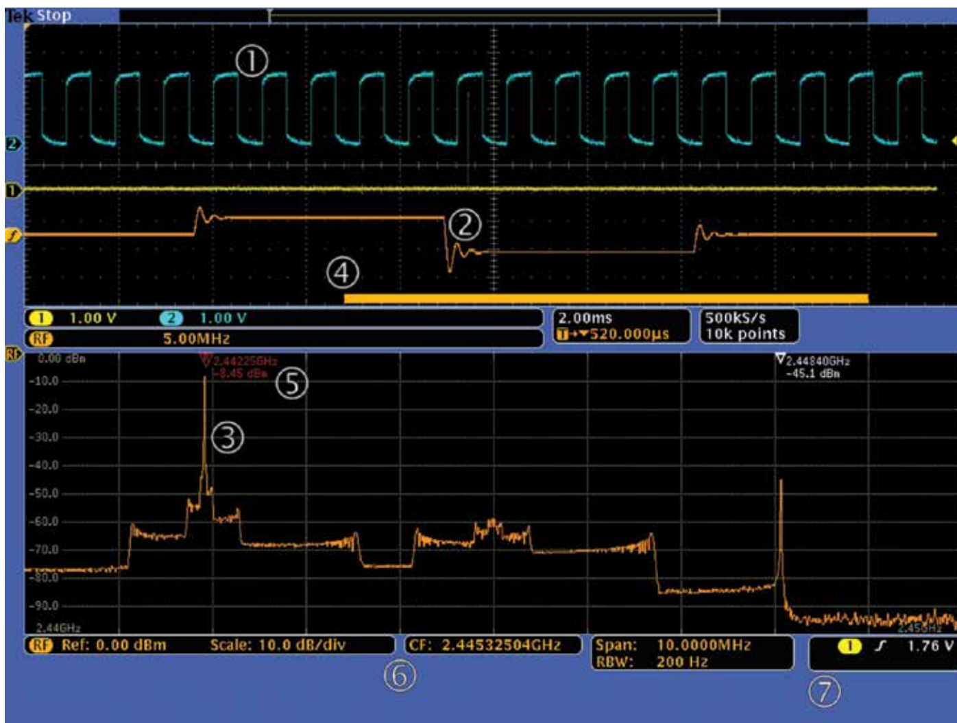
Figure 12. MDO4000B Display Elements.
