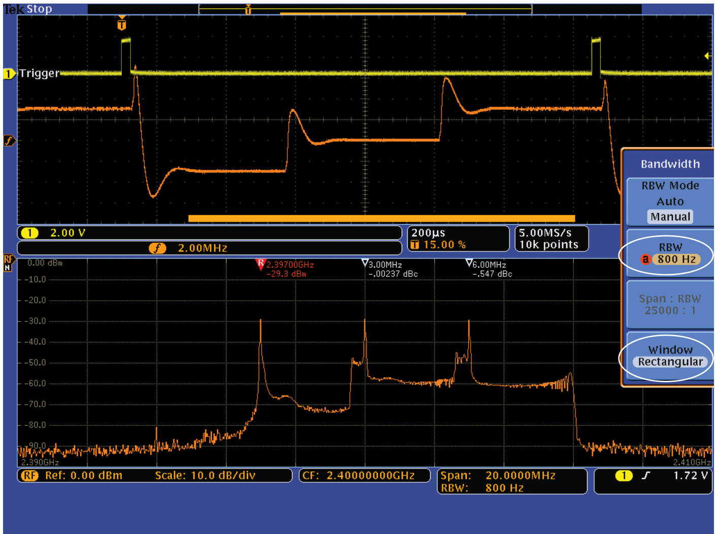
Figure A6. Rectangular Window with 750 Hz RBW.
