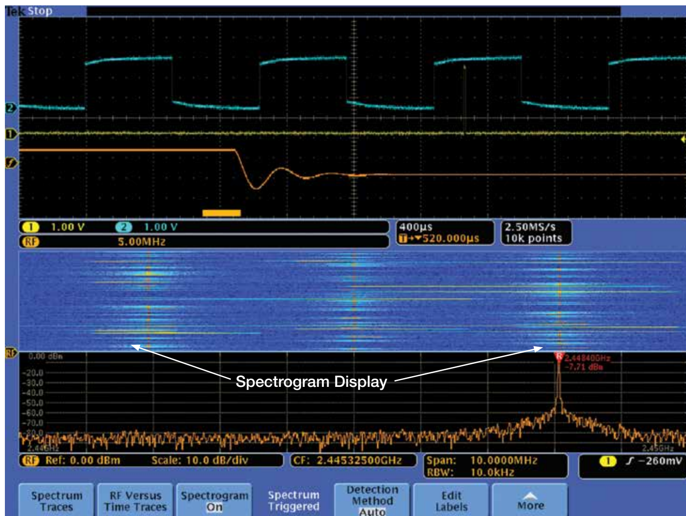
Figure 18. Spectrogram.
