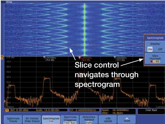
Figure 46. A "Slice" shows previously recorded signals.
