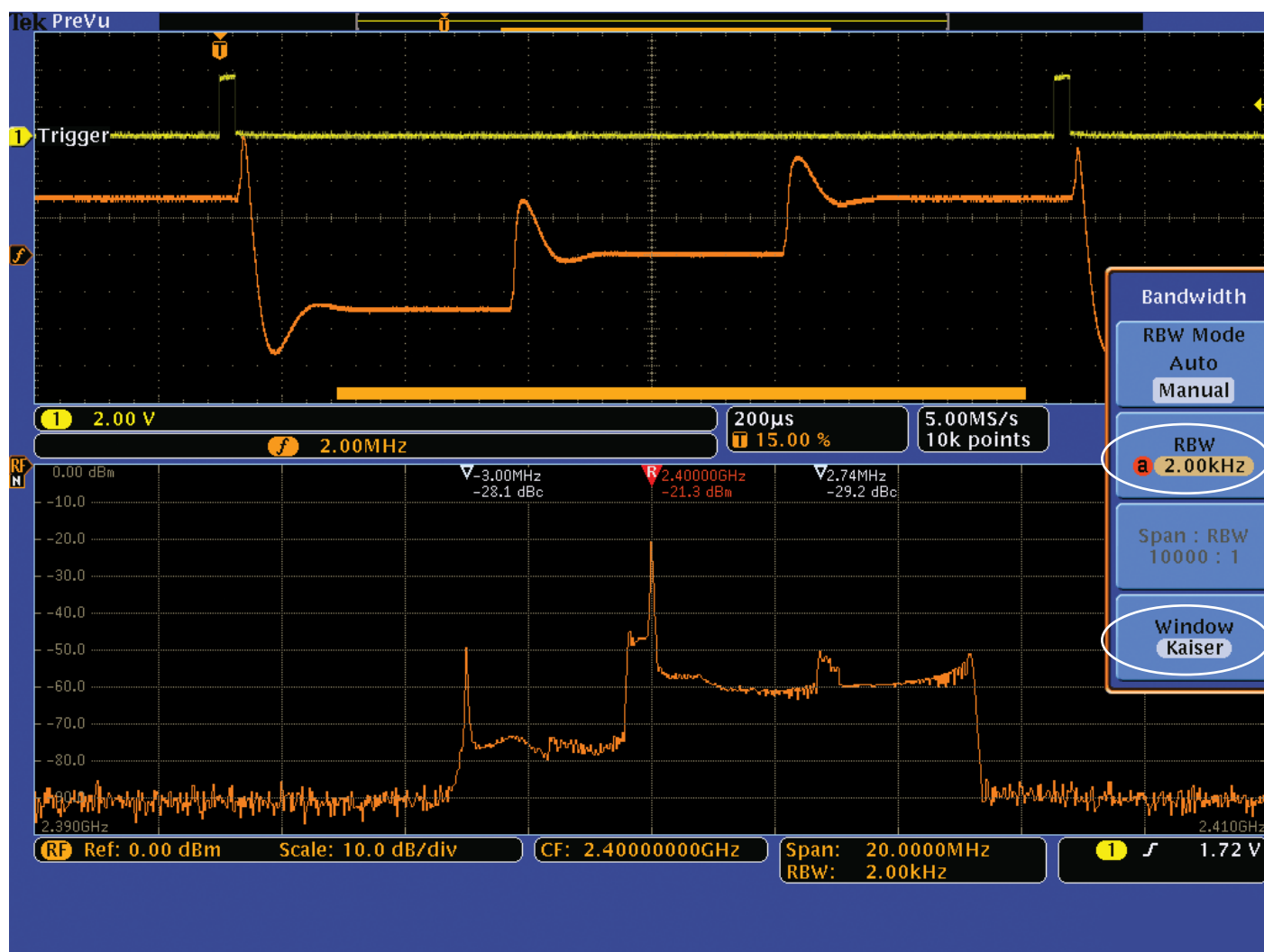
Figure A5. Kaiser Window with 2 kHz RBW.
