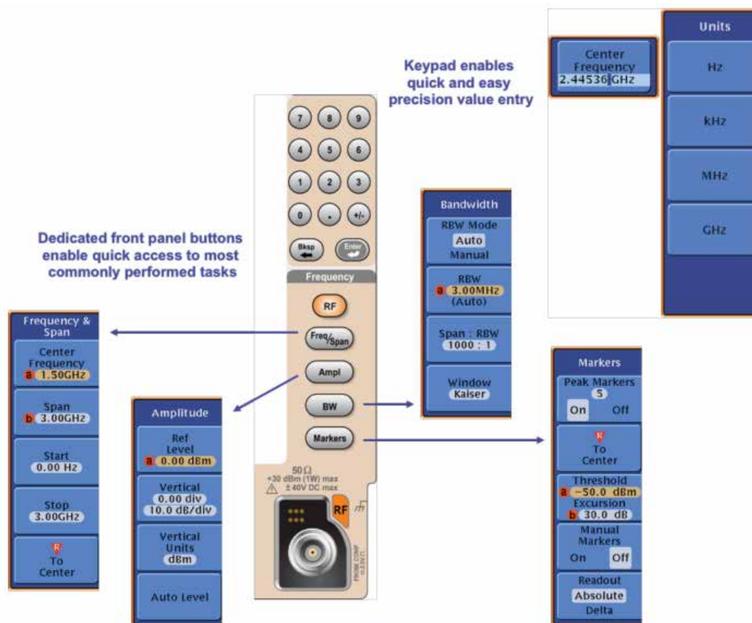
Figure 11. MDO4000B Front Panel.
