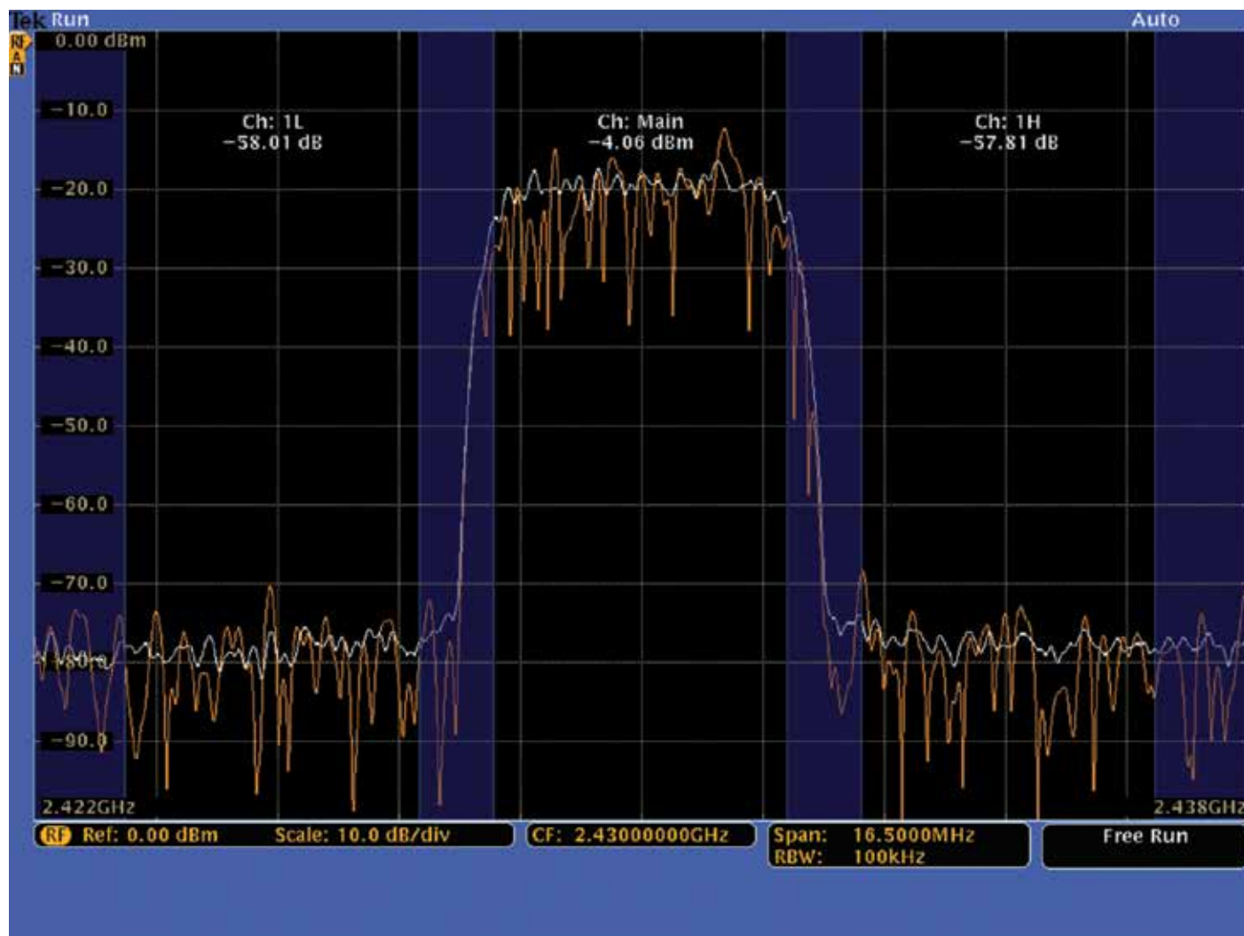
Figure 22. ACPR Measurement.
