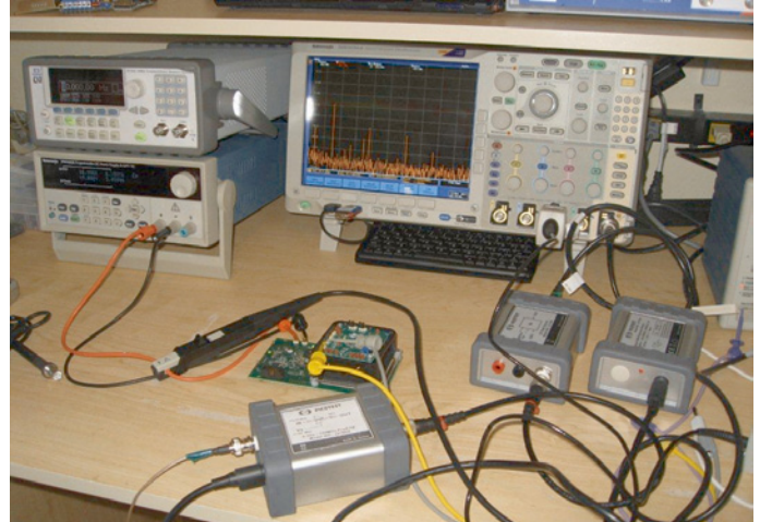
Figure 3. Test setup for measuring the charger including a Mixed Domain Oscilloscope, voltage and current probes, laboratory-grade power supply, and signal injectors.
