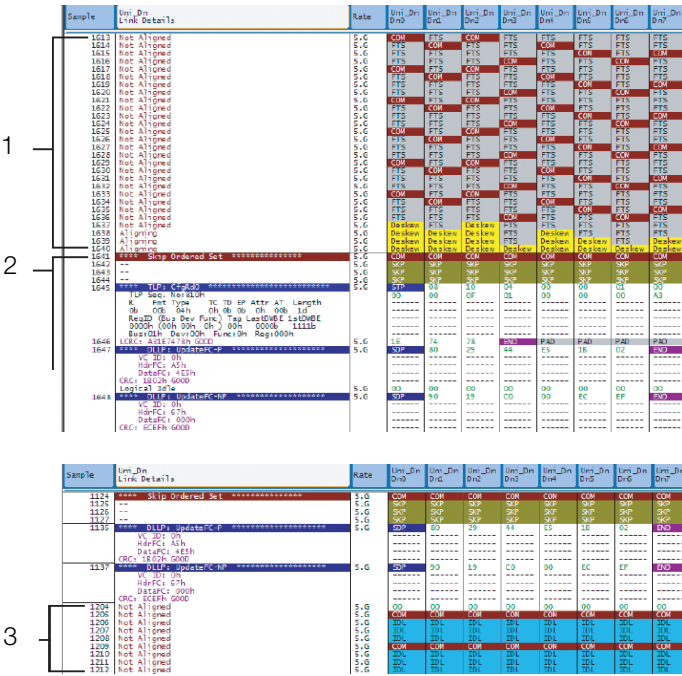
Figure 25. Tektronix TLA Series aligns data across all lanes of the bus. 1. TLA Displays the FTS Packets as the Link Exits Electrical Idle. 2. Data is aligned to the Skip Ordered Set. 3. Link Issues Electrical Idle Ordered Set and Enters L0s.
