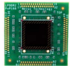
LPDDR 2 Pop Interposer
