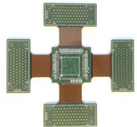
LPDDR3 Pop Interposer
