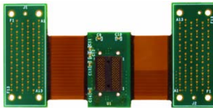
DDR3/4 Component Interposer
