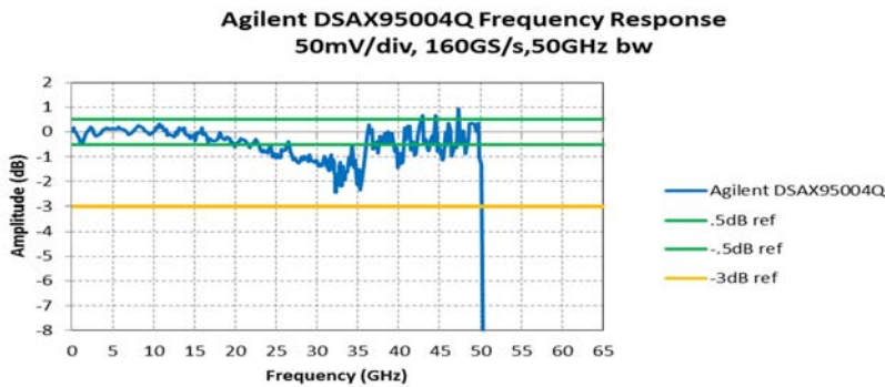
Figure 7. Agilent DSAX95004Q frequency response plot.
