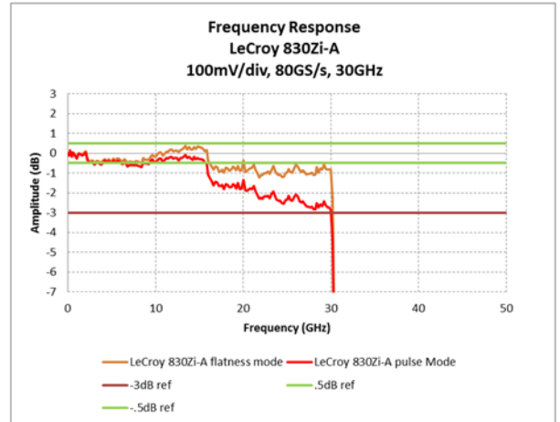
Figure 6. LeCroy 830Zi-A frequency response plot.
