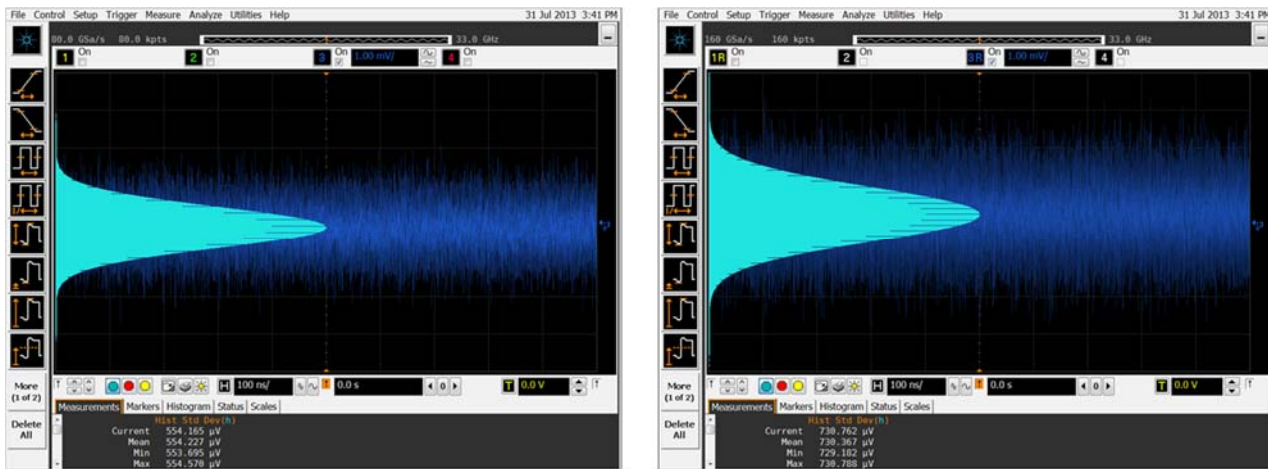
Figure 9. Noise performance comparison of Agilent DSAX95004Q oscilloscope channels (standard vs “RealEdge”).
