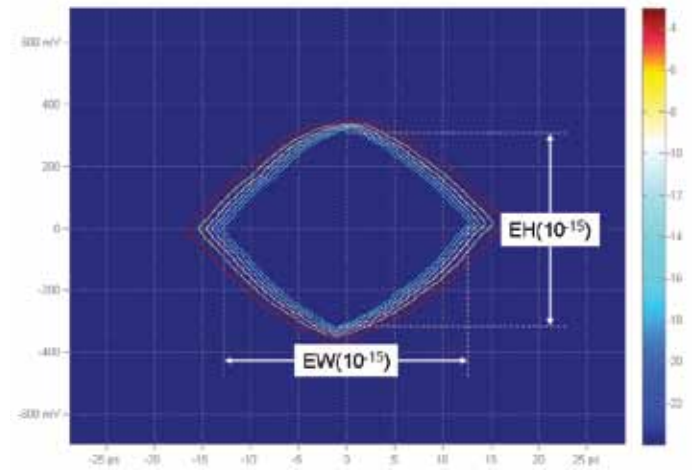
Figure 13. Measurements of EH(10^{-15}) and EW(10^{-15}) with a BER Eye diagram.
