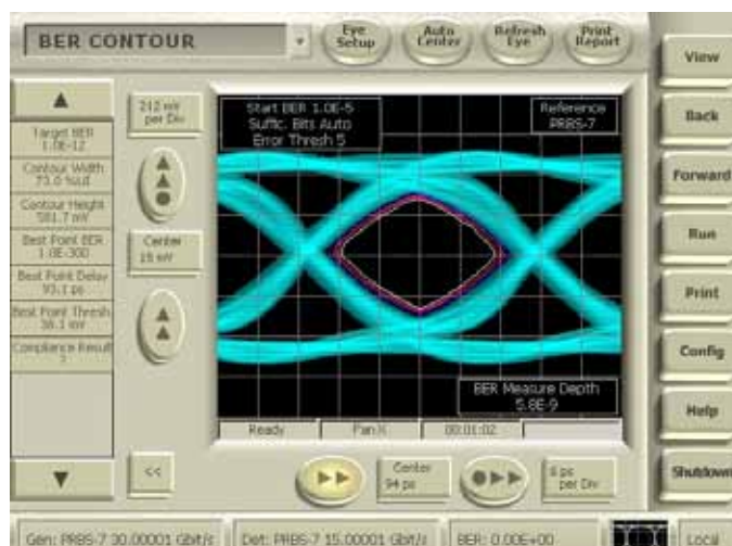
Figure 5b. BER Contour for J9 with BERTScope using a 30 Gb/sec signal.
