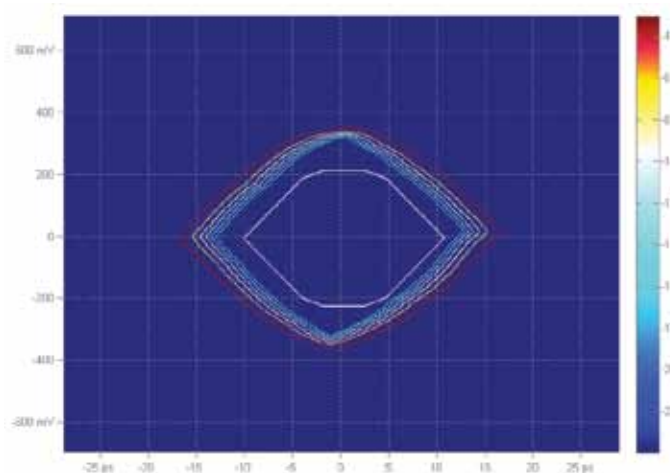
Figure 5a. Eye mask testing with BER contours. The BER=10^{-6} contour, the outer yellow-orange contour, corresponds to a 5 \times 10^{-5} hit ratio.
