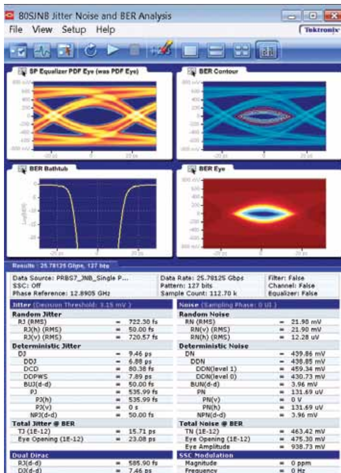
Figure 15. A stressed signal.
