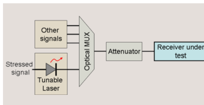
Figure 11. Optical stressed receiver test.
