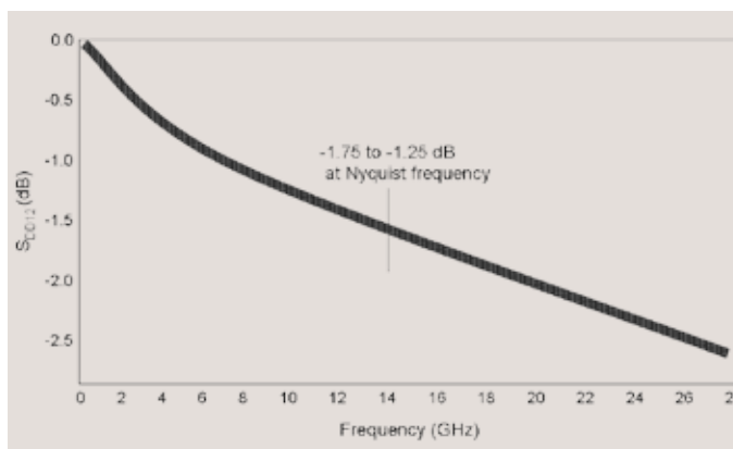
Figure 12. Differential frequency response of typical compliance test boards.
