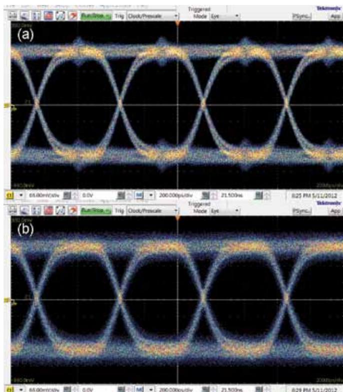
Figure 3. Victim eye diagrams for (a) synchronous and (b) asynchronous crosstalk.
