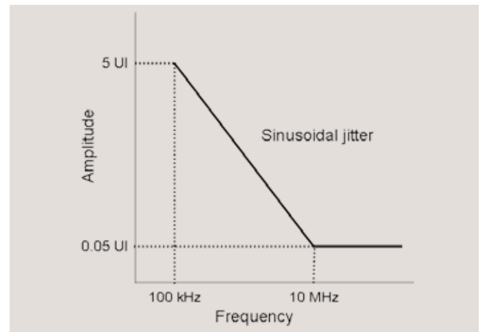
Figure 7. Sinusoidal Jitter stress template.
