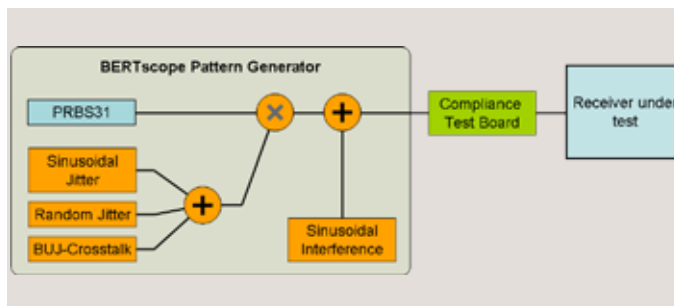
Figure 14. Electrical stressed receiver test setup.
