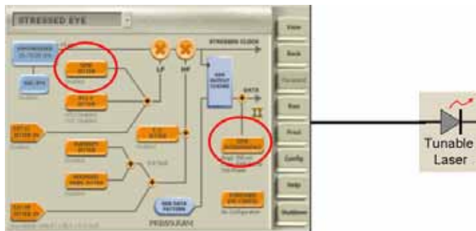
Figure 6. Sinusoidal Interferers directly from the BERTScope driving a laser for Optical Receiver Testing.
