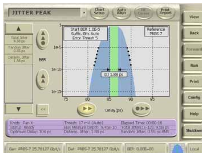
Figure 10. Jitter Peak with J9 measured on a BERTScope.
