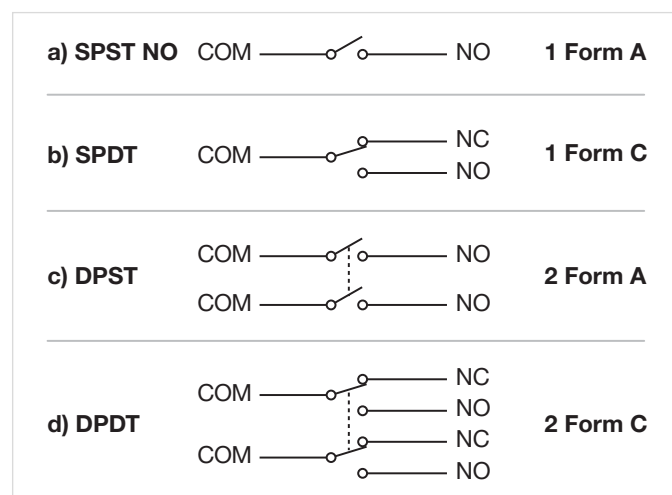
Figure 4. Relay type schematics.
