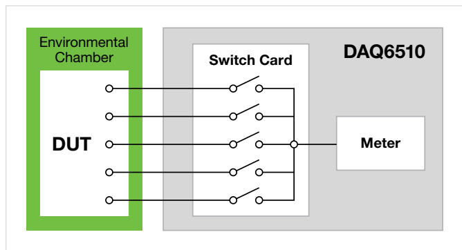
Figure 27. Block diagram of a potential temperature profiling setup.
