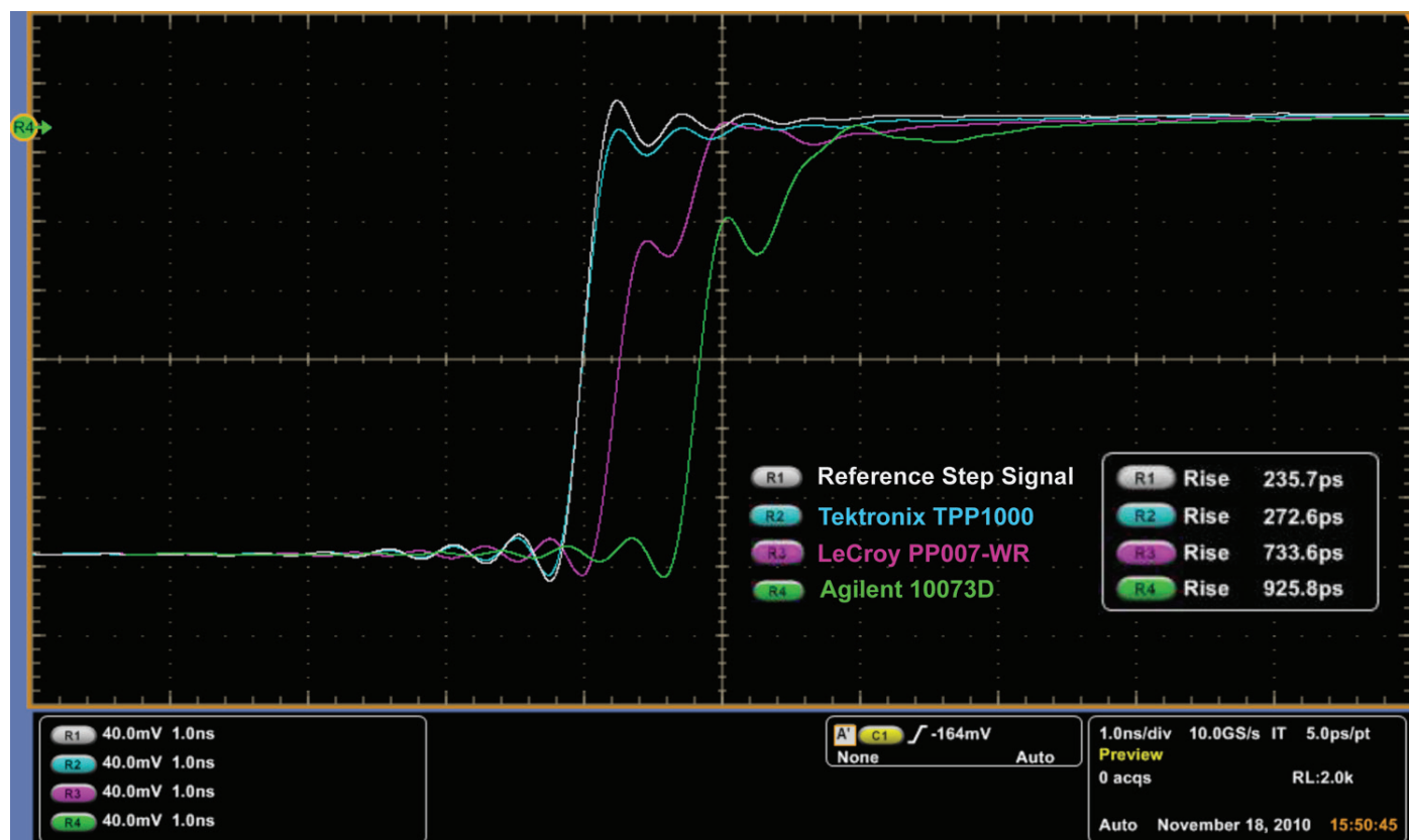
Figure 3. Probe Loading Impacts of Standard Passive Voltage Probe.
