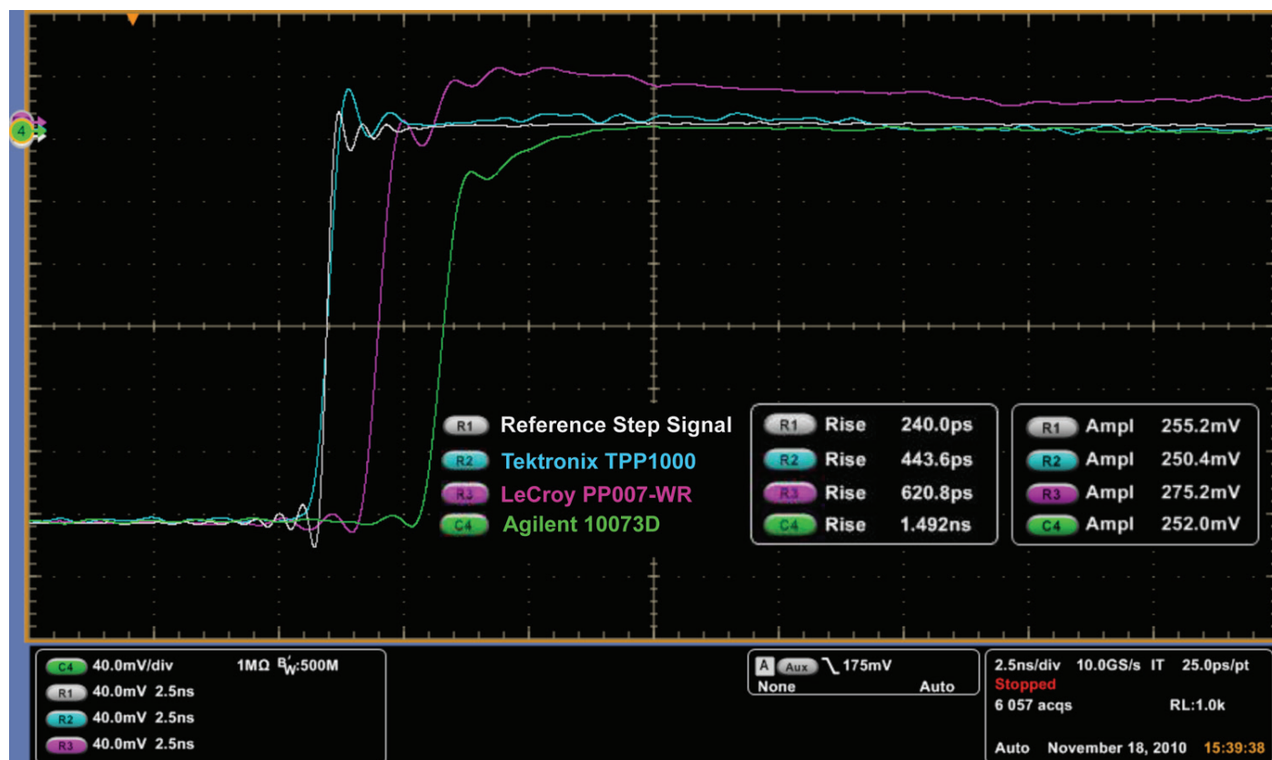
Figure 1. Rise Times of Tektronix, LeCroy, and Agilent Standard Passive Voltage Probes.
