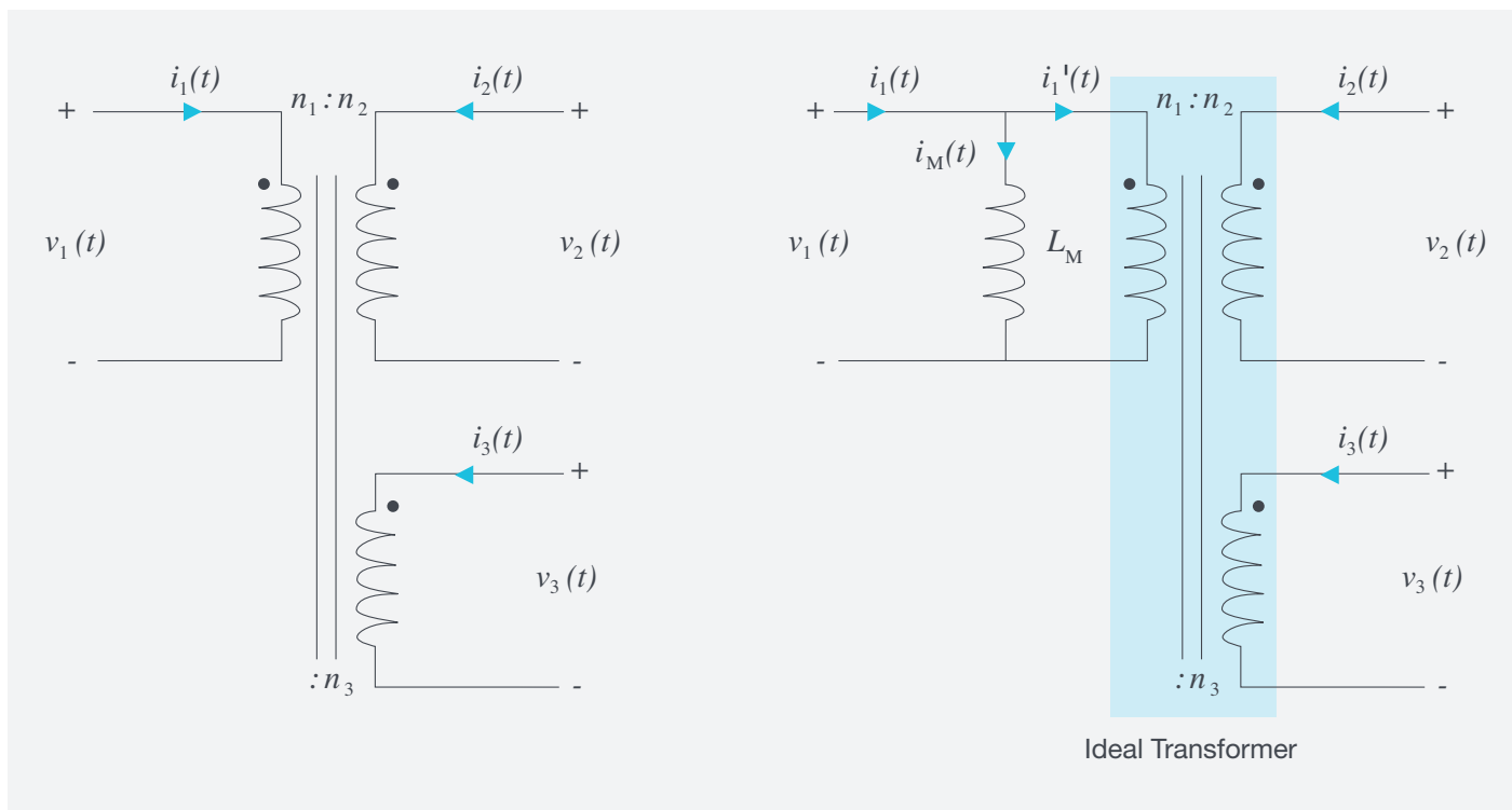
FIGURE 9. Transformer schematic (left) and equivalent circuit (right) showing magnetizing current flowing through an imaginary inductor, L_M in parallel with the primary. L_M models the magnetic characteristics of the transformer.
