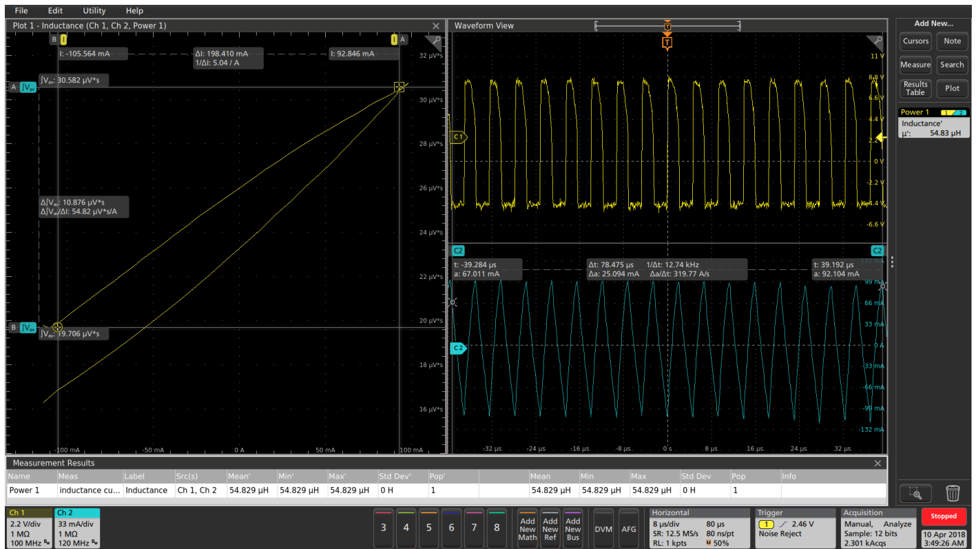
FIGURE 4. Inductance measurement gives the average inductance value in Henries. The yellow waveform (CH1) is the voltage across the inductor and the blue waveform (CH2) is the current through the inductor. The plot on the left shows current, i versus \int v dt , the slope of which is inductance.
