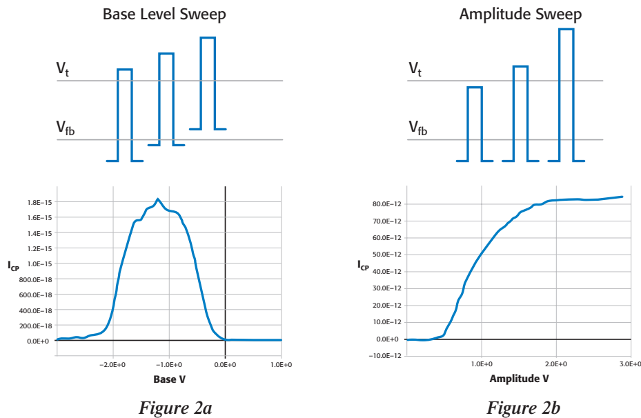
Figure 2. Two types of sweeps for charge pumping: a) base voltage sweep, b) pulse amplitude sweep.
