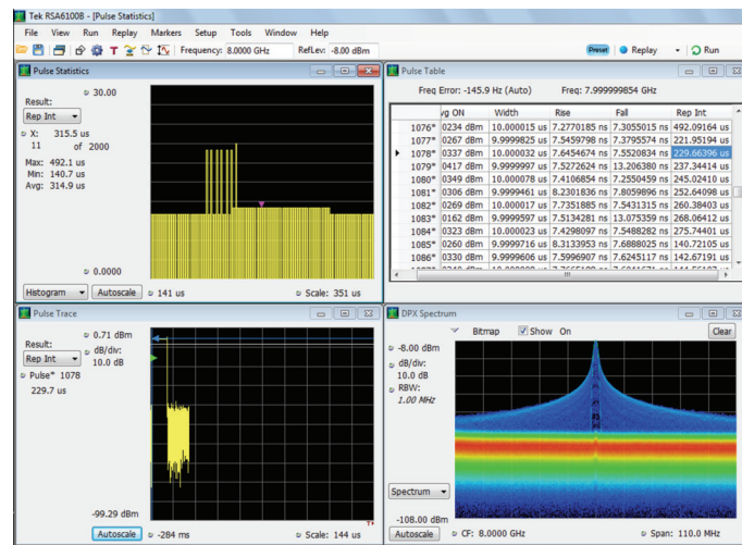
Figure 11. This test result evaluates the pulse repetition interval (PRI) is being measured on a set of 2000 pulses constructed as a staggered PRI CW pulse waveform on the AWG70001B.
