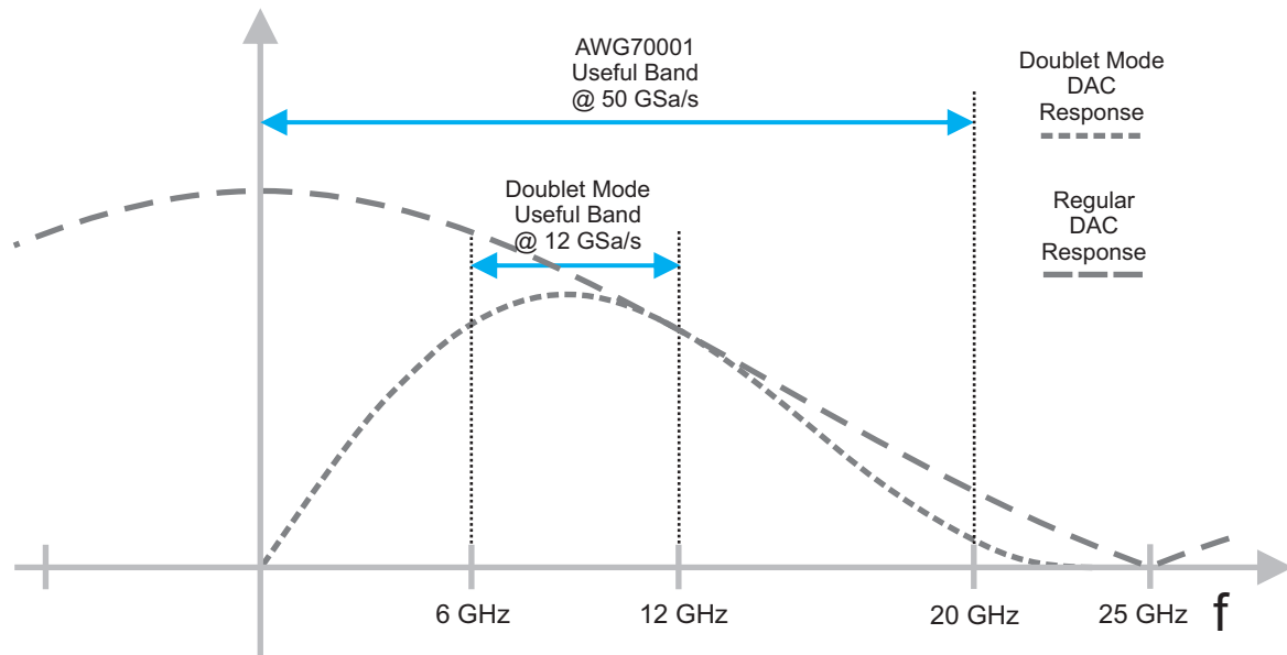
Figure 14. The generation of signals in the second Nyquist zone may be improved with the “Doublet” DAC mode. This mode is specifically designed to boost im-ages in the second Nyquist zone and attenuate the direct signal located in the first Nyquist zone. Here the response of a 12 GS/s generator using a “doublet” mode DAC and that of the Tektronix AWG70001 running at 50 GS/s are compared. Although the frequency coverage of the 12 GS/s generator has been extended, the AWG70001 clearly outperforms it in terms of both carrier frequency range (0-20GHz vs. 6-12GHz) and modulation bandwidth (20 GHz vs. 6GHz).
