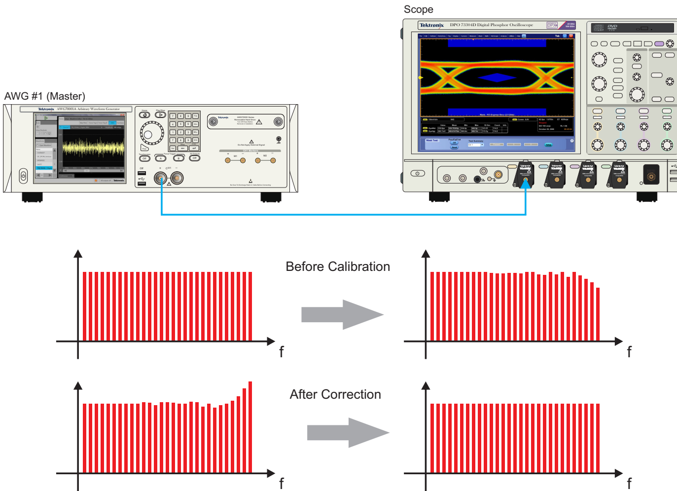
Figure 17. Good-quality wideband signal generation requires proper equalization to make sure flatness and group delay are kept within acceptable limits. Proper correction filters can only be obtained after calibration and they must incorporate the effects of external components such as cabling and amplifiers. The excellent flatness and phase linearity of the Tektronix DPO/DSA70000 Series oscilloscopes makes them an ideal calibration solution. Oscilloscopes, unlike traditional spectrum analyzers, can easily obtain System Under Test frequency response for both amplitude and phase and, equipped with the right software, can also be used to analyze RF wideband signals.
