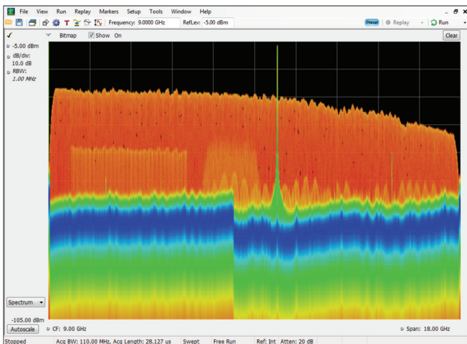
Figure 10. Wide-band environment generated by a one-channel AWG70001B.
