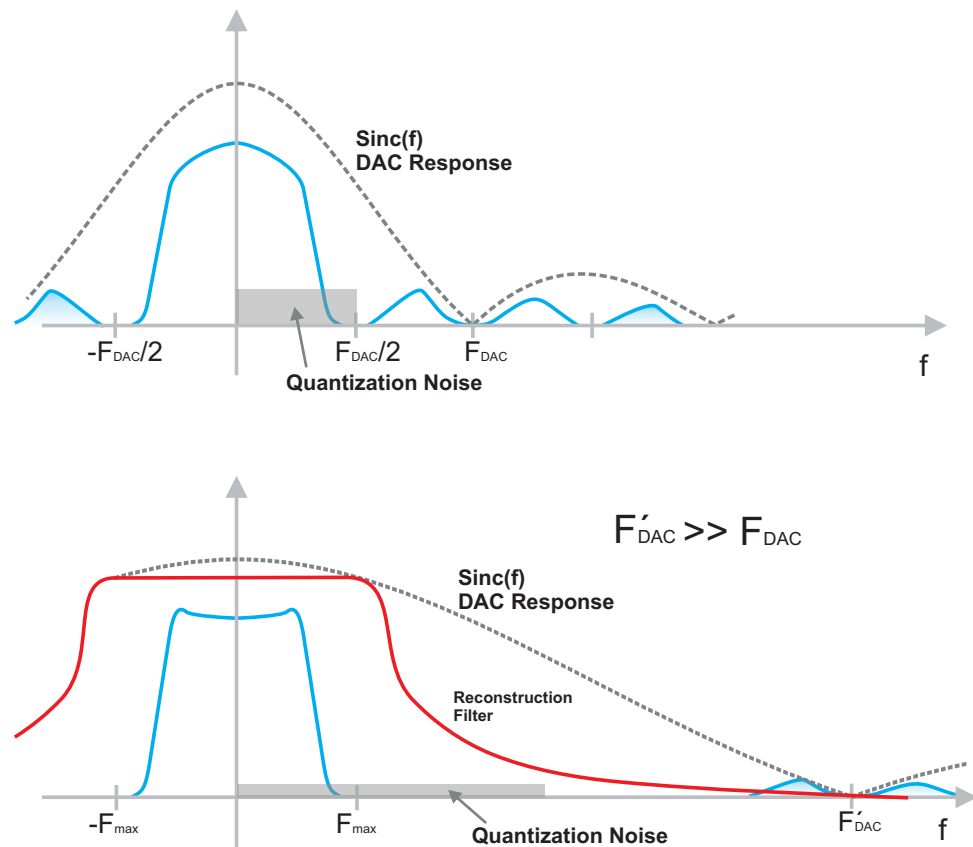
Figure 7. Generating a limited bandwidth signal at a much higher sampling rate than that required by the sampling theorem ( F_s = 2 \times BW ) is known as oversampling. This technique improves the quality and usability of the signal as it improves SNR (and effective bits) and flatness while relaxing the requirements for reconstruction filters.
