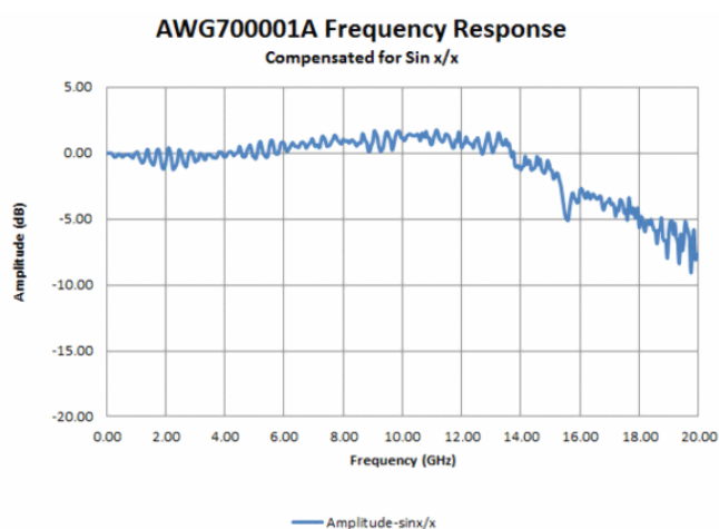
Figure 13. AWG70001A frequency response after removing the influence of the DAC's \text{Sinc}(f) response. The low attenuation of frequencies as high as 20 GHz permits the direct generation of modulated carriers at those frequencies.
