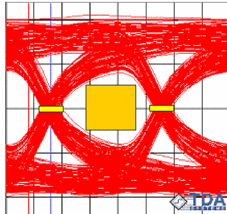
2 10 -1 IConnect eye from TDT measurement
