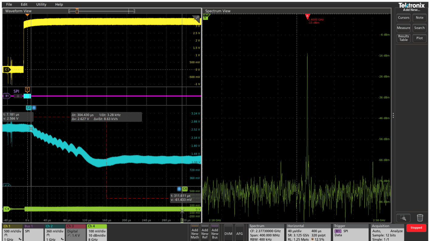
FIGURE 13. We are triggering on the SPI bus command that tells the VCO what frequency to tune to. In this case, it's 2.4 GHz. Using Spectrum Time, we were able to scroll through the acquisition and see when the RF output stabilized at 2.4 GHz. Then, using cursors, we can measure from the trigger event to Spectrum Time's location and see that it took 304 μs for the output to achieve the desired frequency.
