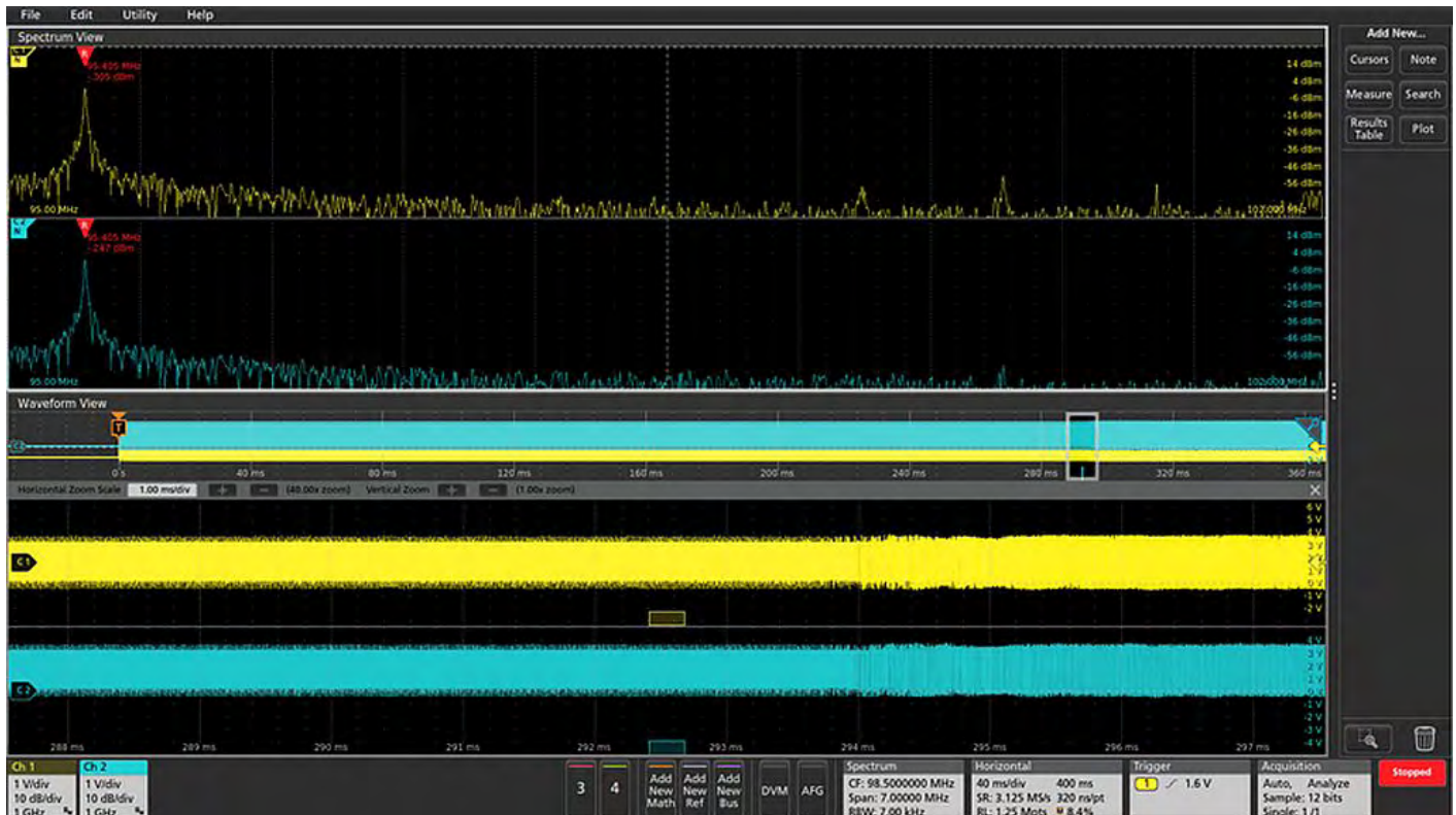
FIGURE 14. When debugging tasks demand it, multiple channels can be analyzed simultaneously. Here, two channels show the startup of a clock signal from two different points in a circuit.
