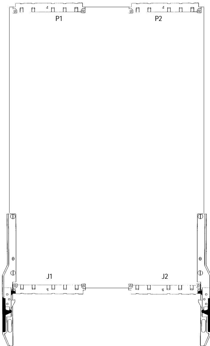
Figure 1: Side View of Extender Board
