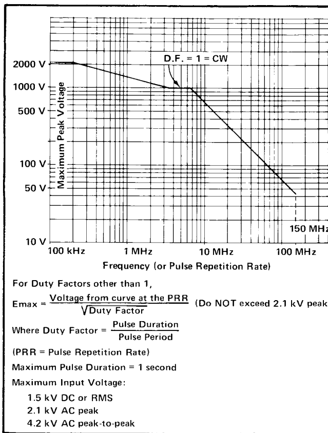
Fig. 2. P6009 Probe, maximum input voltage versus frequency.
