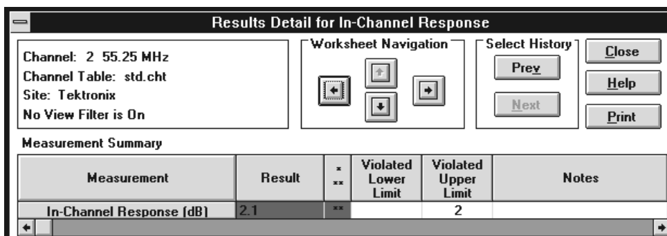
Figure 2–47: The Results Detail dialog box for the In-Channel Response measurement for the first channel
