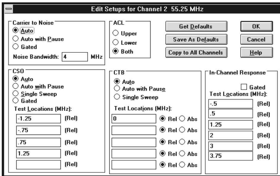
Figure 2–35: The Edit Setups dialog box for channel 2
