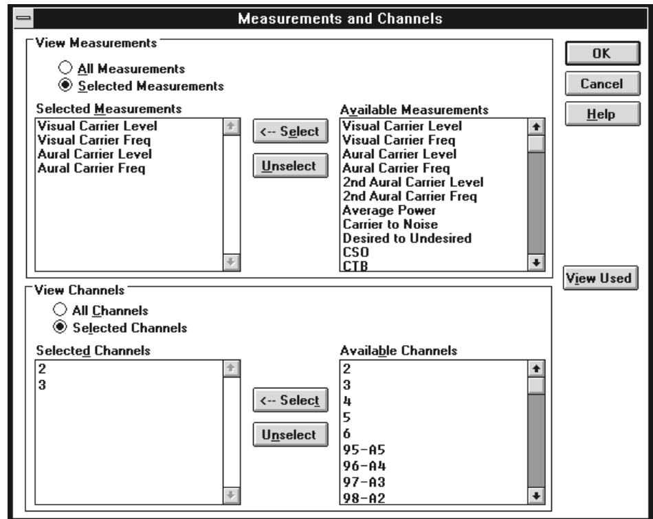
Figure 2-59: The Measurements and Channels dialog box
