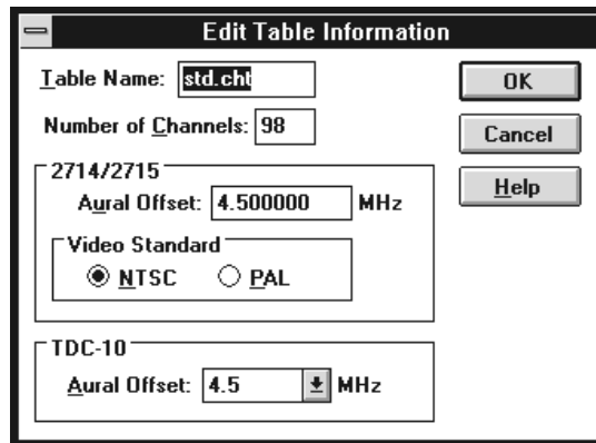
Figure C-20: The Edit Table Information dialog box
