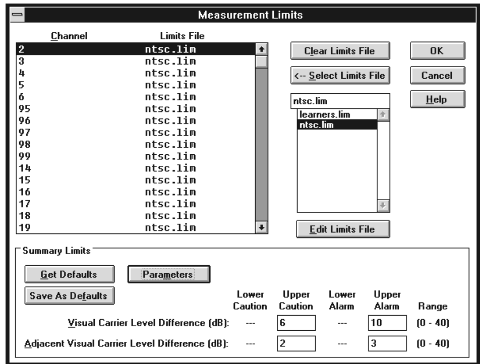
Figure 2–68: The summary limits
