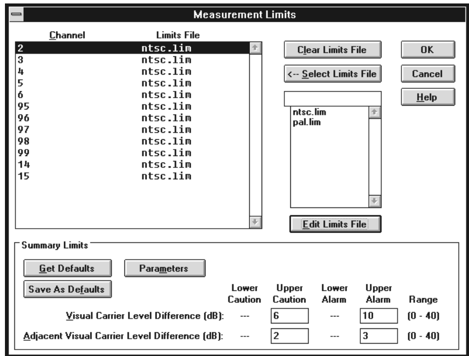
Figure 3–43: Summary Limits dialog box
