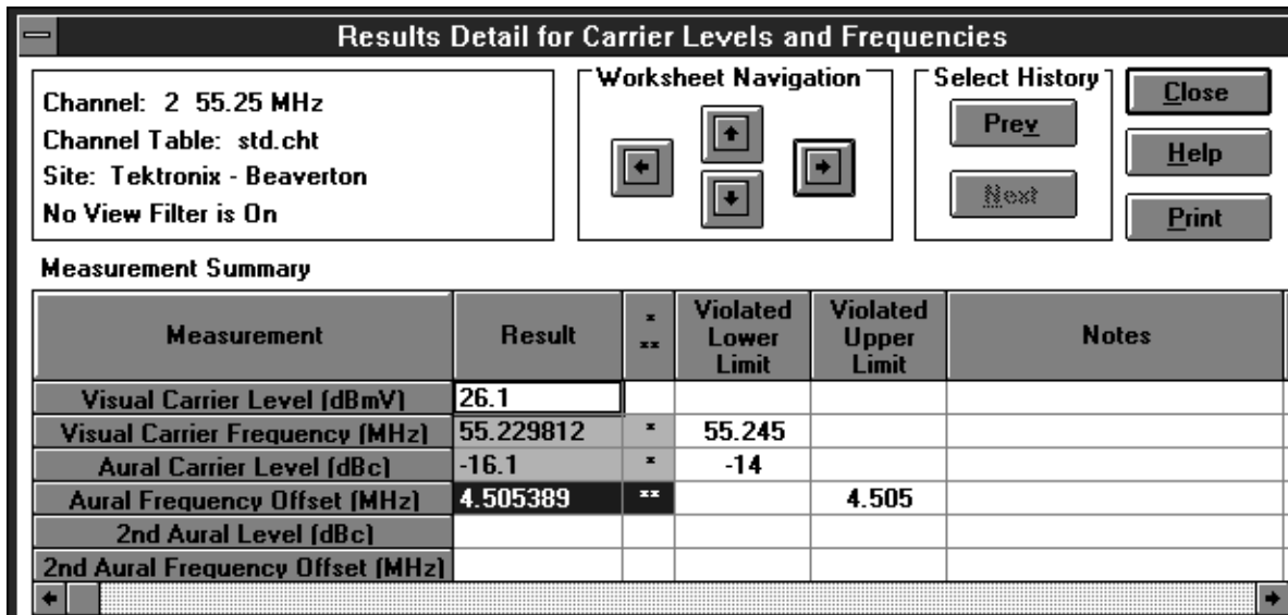
Figure 2-51: The Results Detail display
