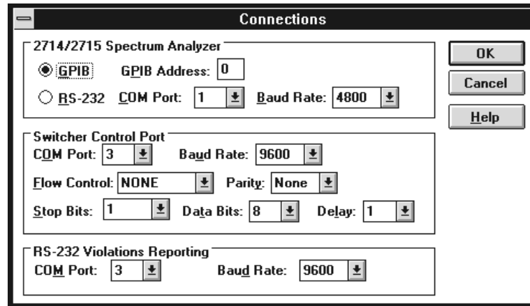
Figure 3–51: Connections dialog box
