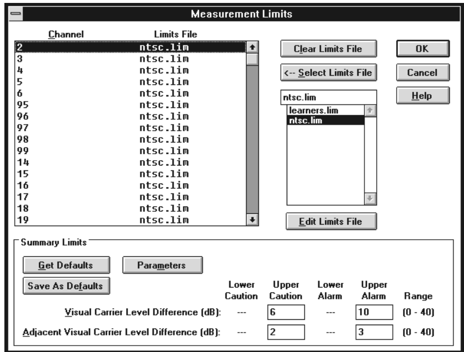
Figure 2–64: The Measurement Limits dialog box
