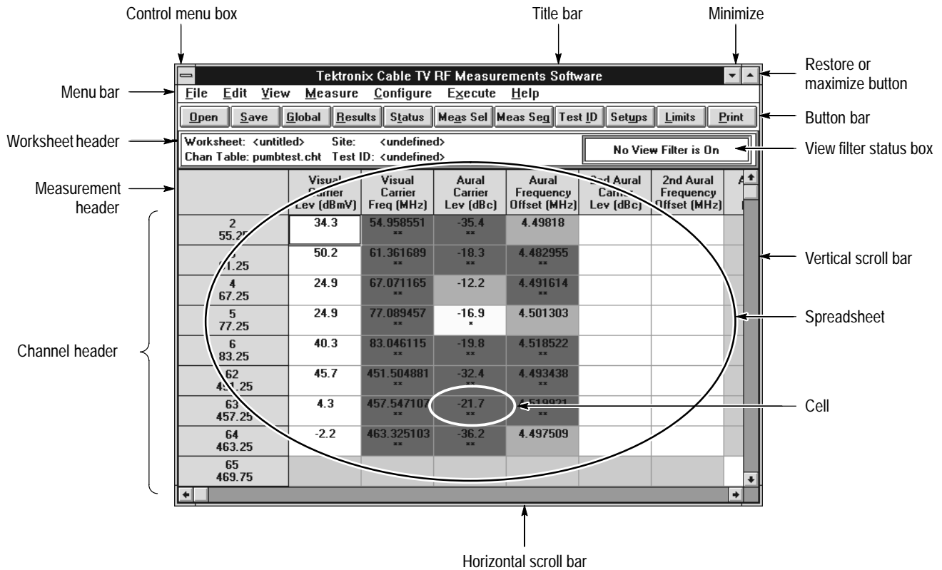
Figure 3-1: Parts of the Cable TV RF Measurements Software for Windows worksheet
