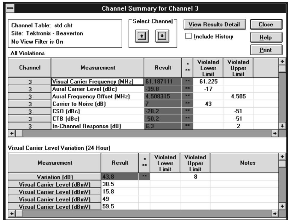
Figure 3–20: Example of a Channel Summary
