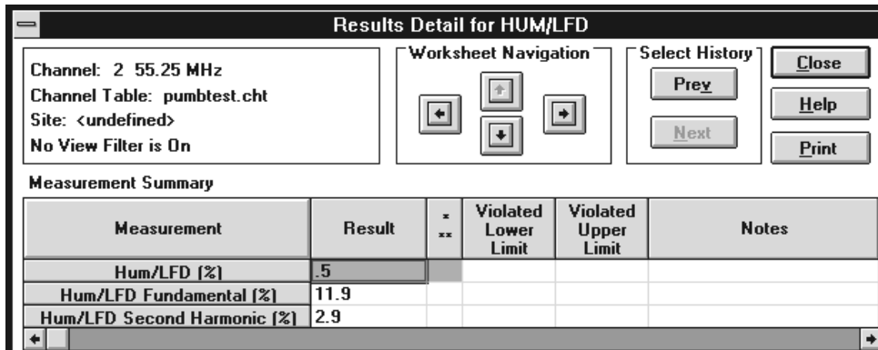
Figure 2–46: The Results Detail dialog box for the Hum/LFD measurement
