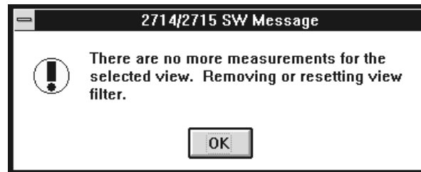
Figure 3–25: Warning message
