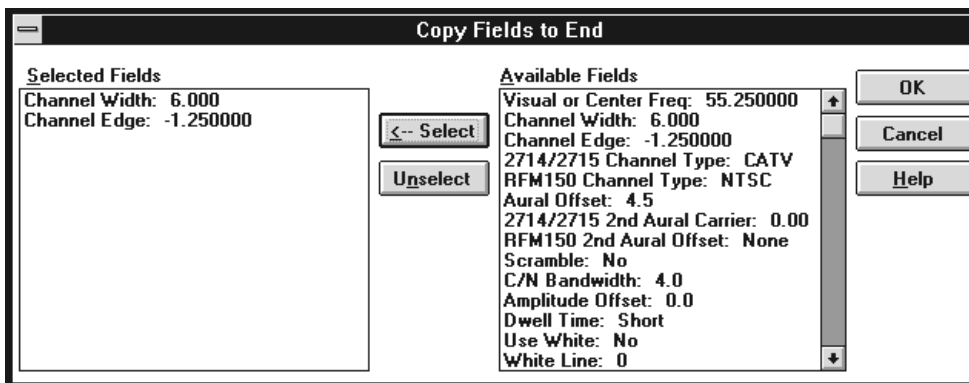
Figure C–19: The Copy Fields to End dialog box
