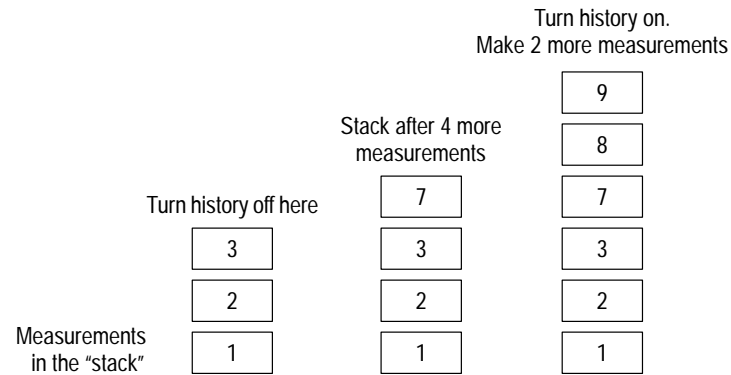
Figure 2–41: The life of a cell with Collect History turned on and off
