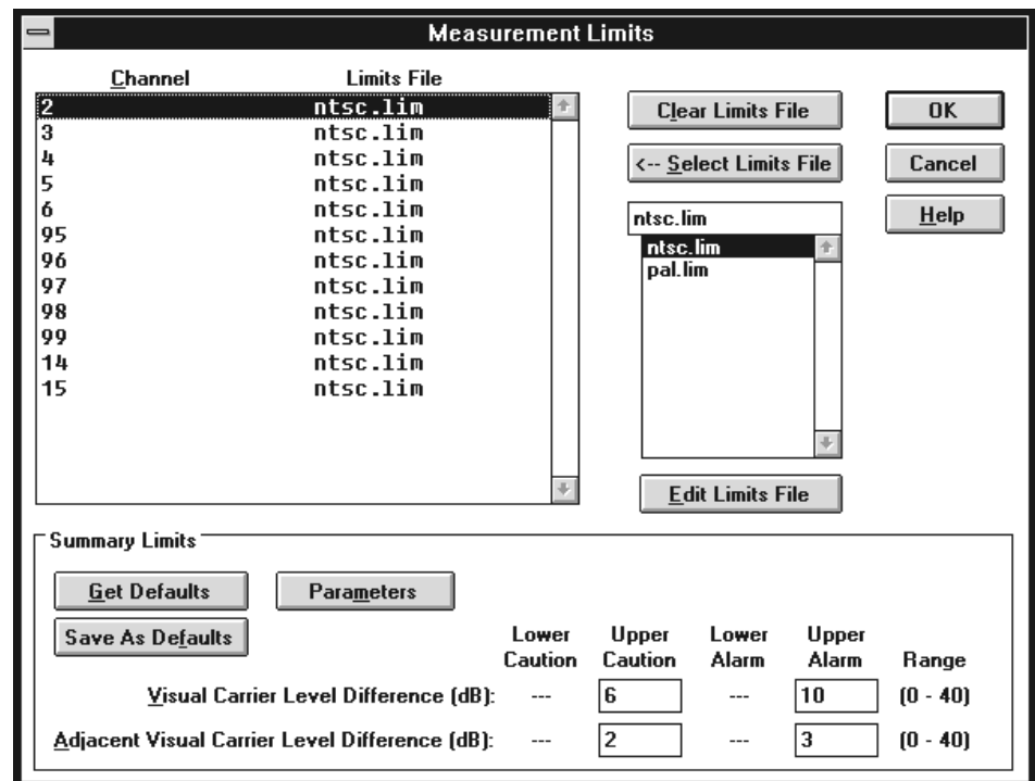
Figure 3–39: The Measurement Limits dialog box
