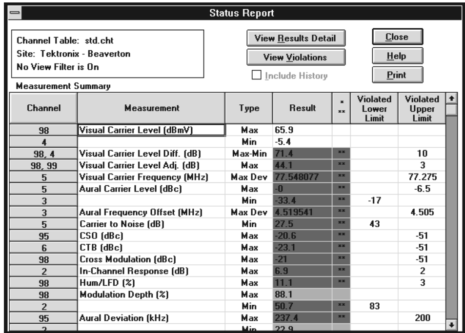
Figure 3–16: The Status Report
