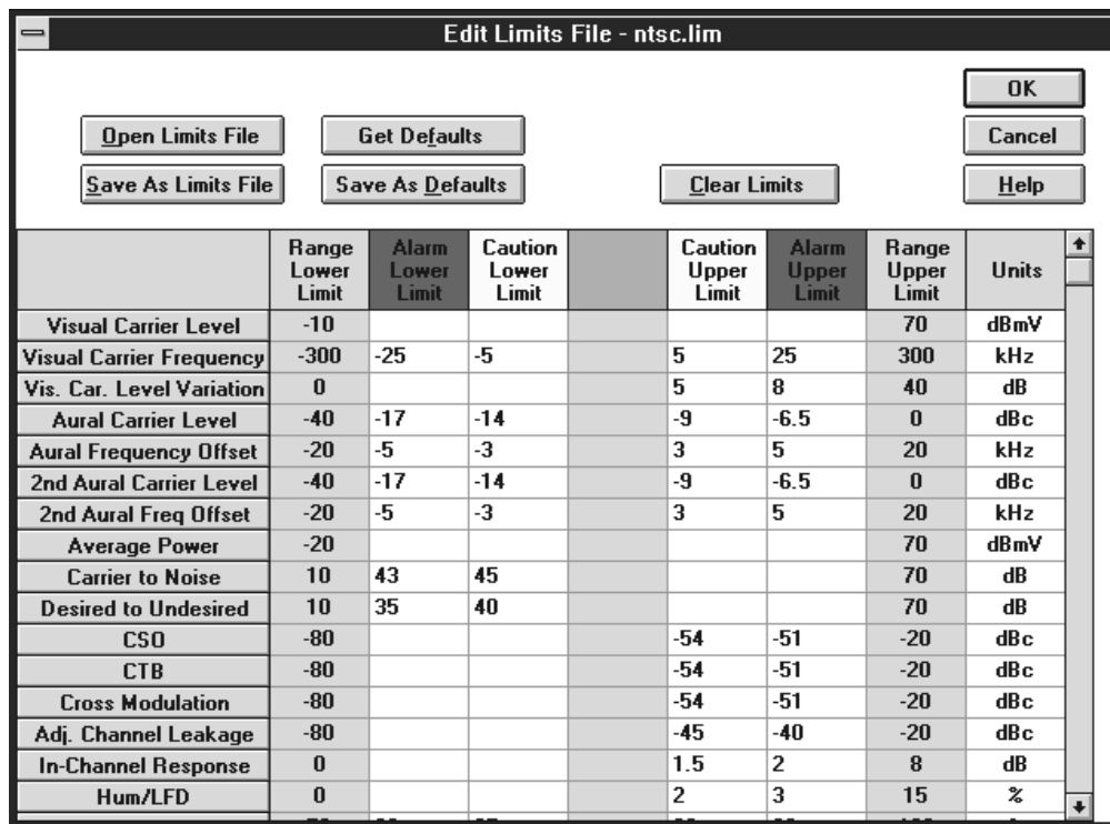
Figure 3–40: The Edit Limits File dialog box
