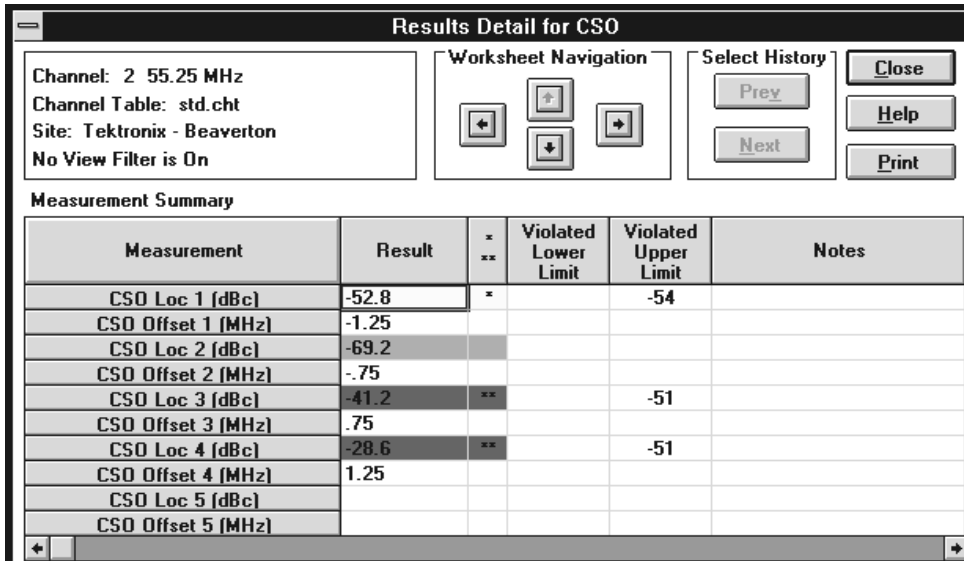
Figure 3–18: Results Detail dialog box
