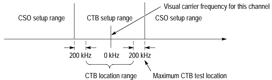
Figure 3-47: CTB/CSO measurement results distribution and CSO setup restrictions
