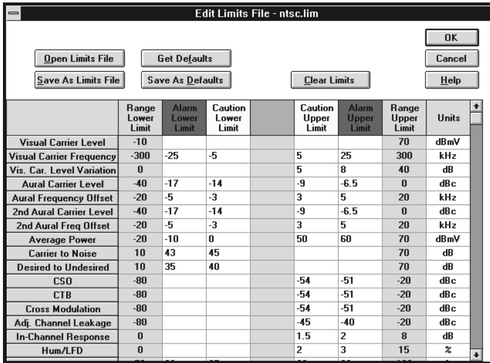
Figure 2-65: The Edit Limits File – ntsc.lim dialog box.
