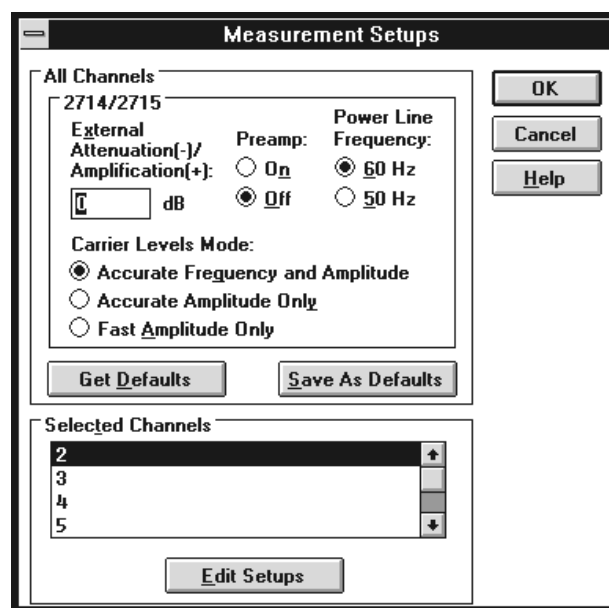
Figure 2–34: The Measurement Setups dialog box
