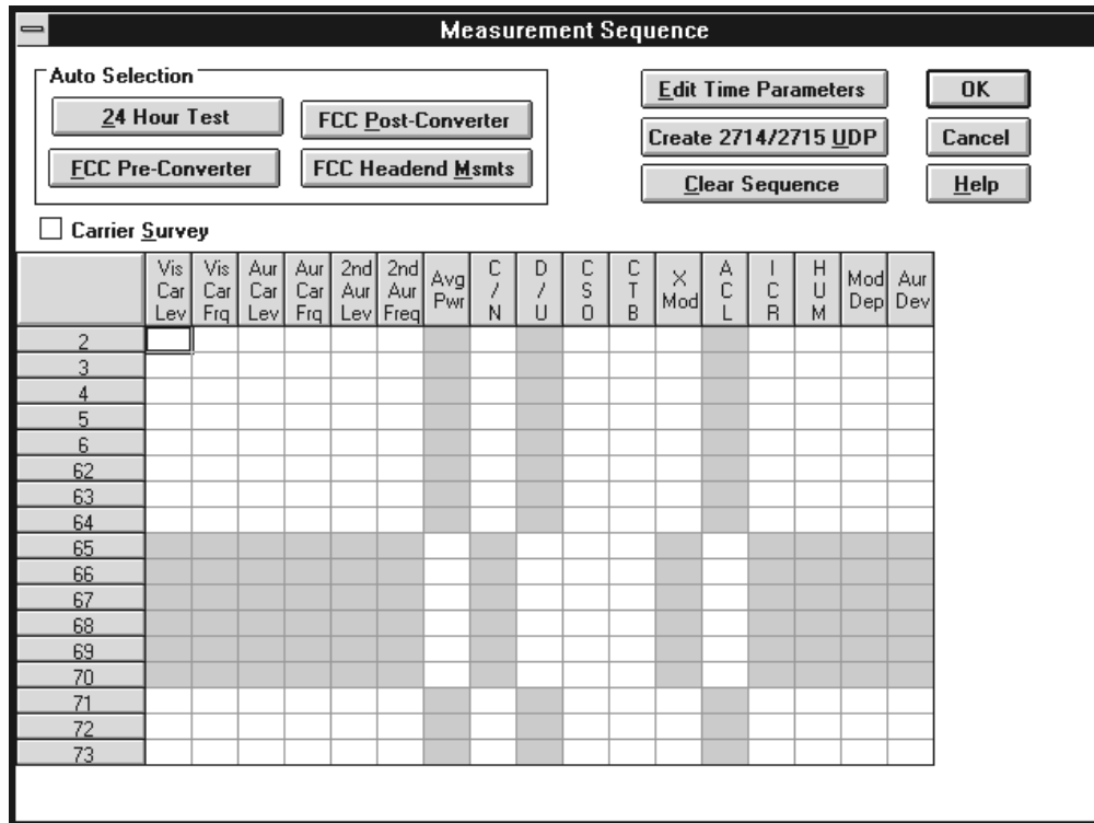
Figure 2–22: The Measurement Sequence dialog box (U.S.A. only)
