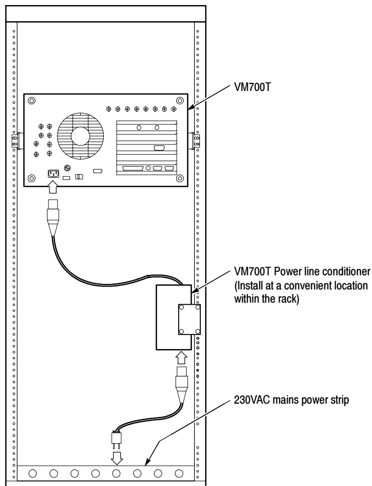
Figure 1-2: Power line conditioner with rackmounted VM700T
