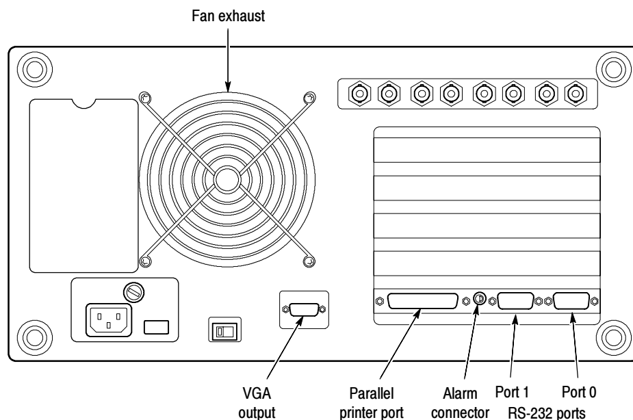
Figure 1-9: VM700T rear panel
