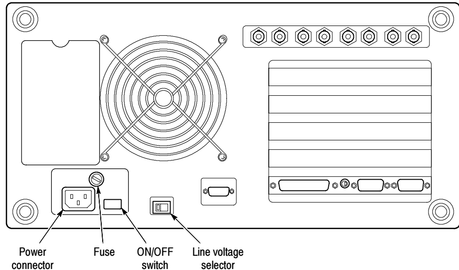
Figure 1- 1: Rear-panel fuse, power connector, ON/OFF switch and Line selector
