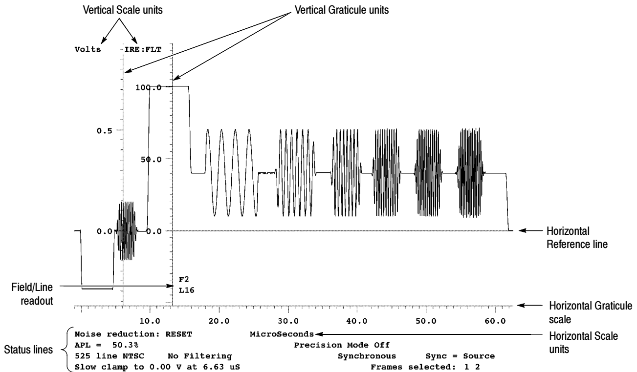
Figure 3- 1: Typical NTSC Waveform display
