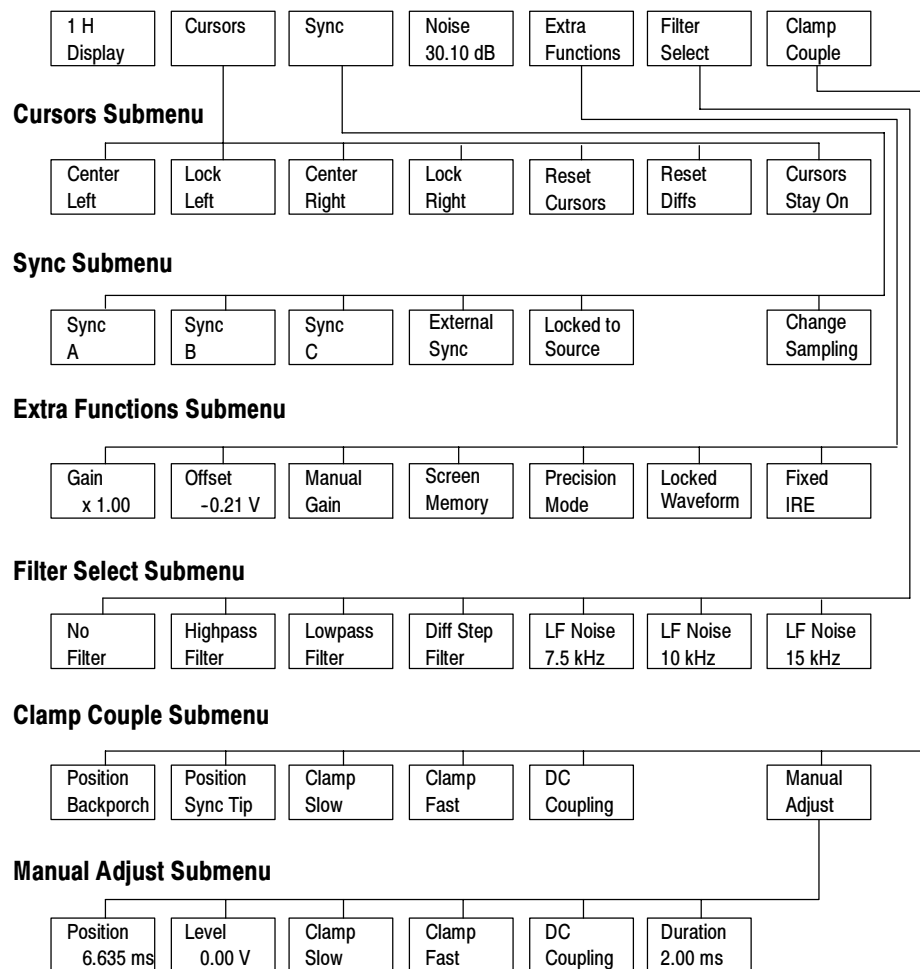
Figure 3-2: Waveform menu tree
