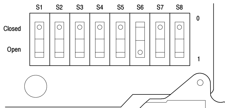
Figure 2-13: DIP switch setting to enable Password
