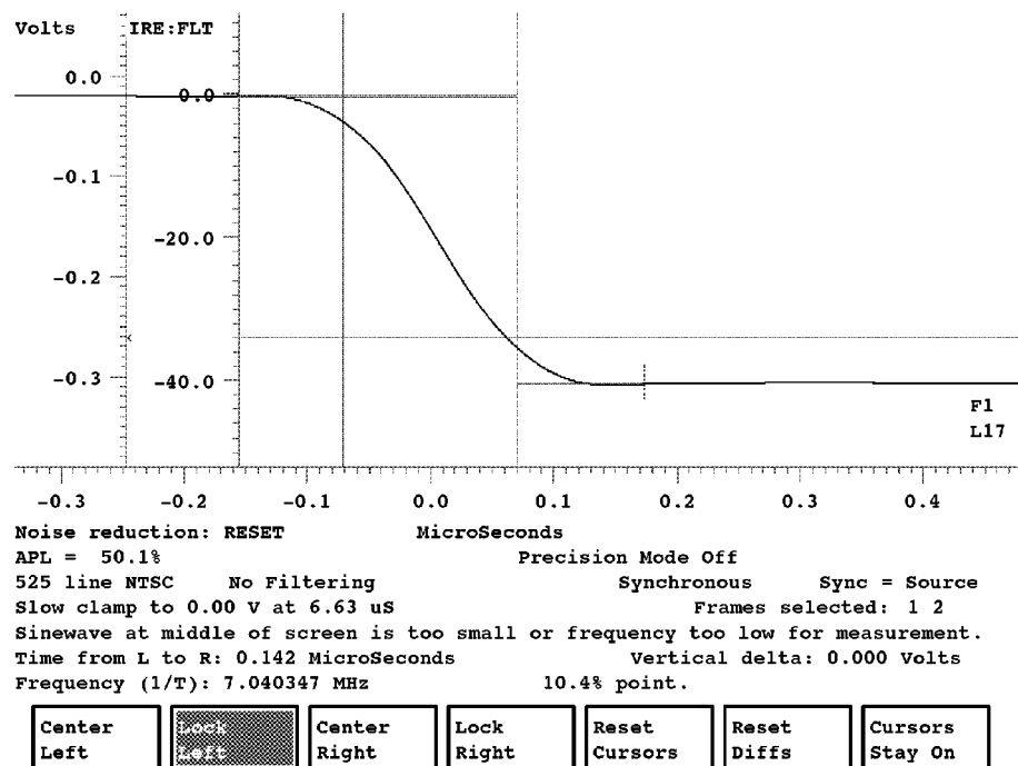
Figure 3-3: Left cursor locked to 90% point of sync edge, right cursor to 10% point
