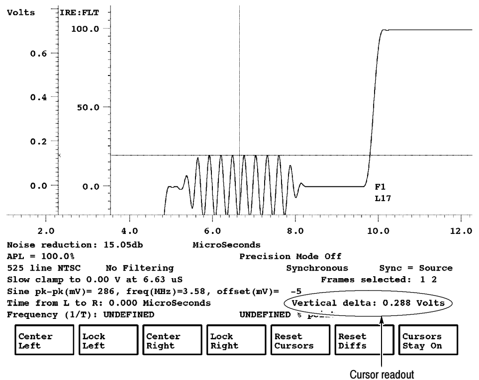
Figure 3-5: Cursors mode indicating color burst amplitude
