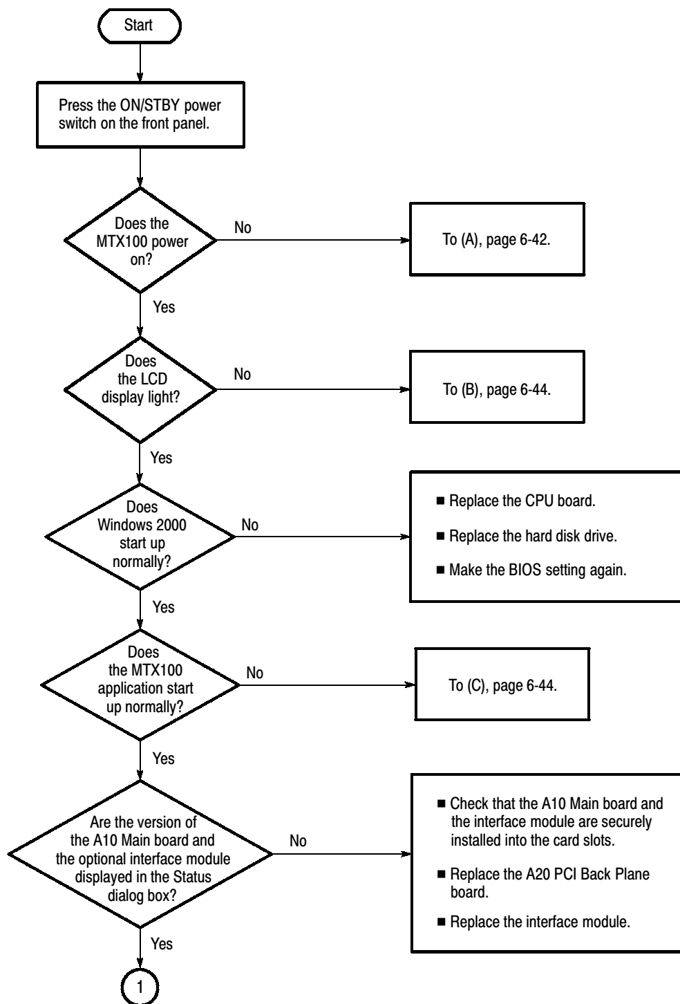
Figure 6-17: Troubleshooting procedure (1)
