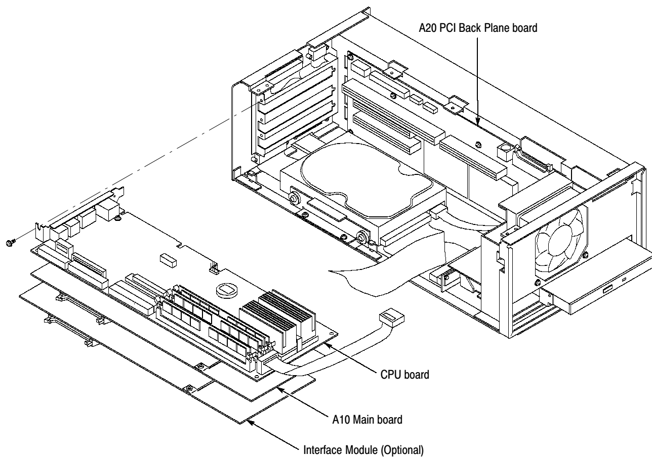
Figure 6-3: Board modules
