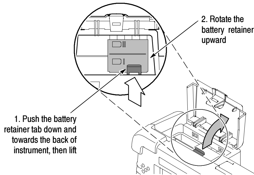
Figure 1-10: Opening the battery retainer
