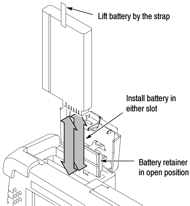
Figure 1-11: Installing/removing a battery
