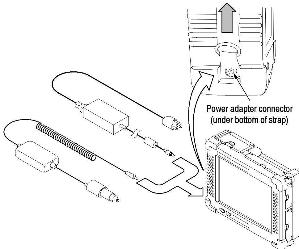
Figure 1-8: External power supplies
