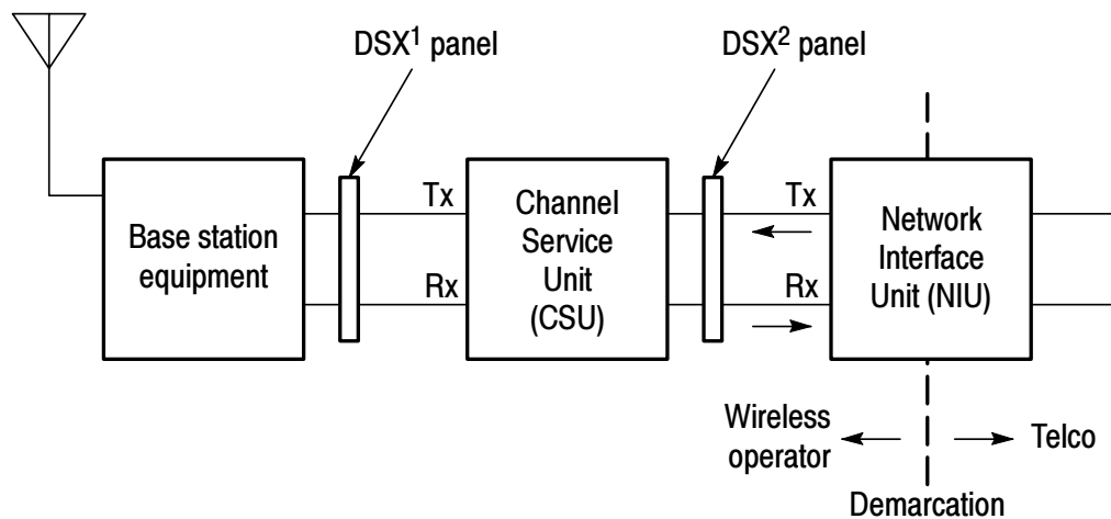
Figure 3-1: Typical base station showing network interfaces
