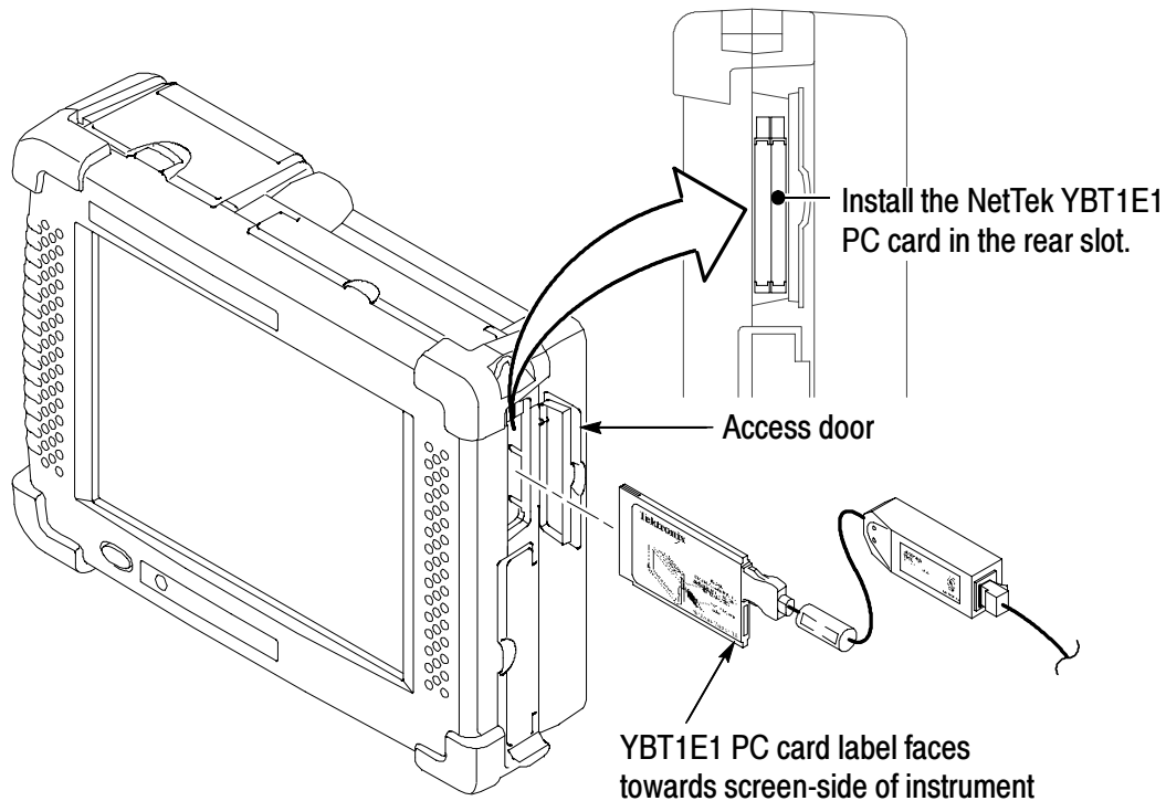
Figure 1-5: Installing the YBT1E1 PC card in the NetTek Analyzer
