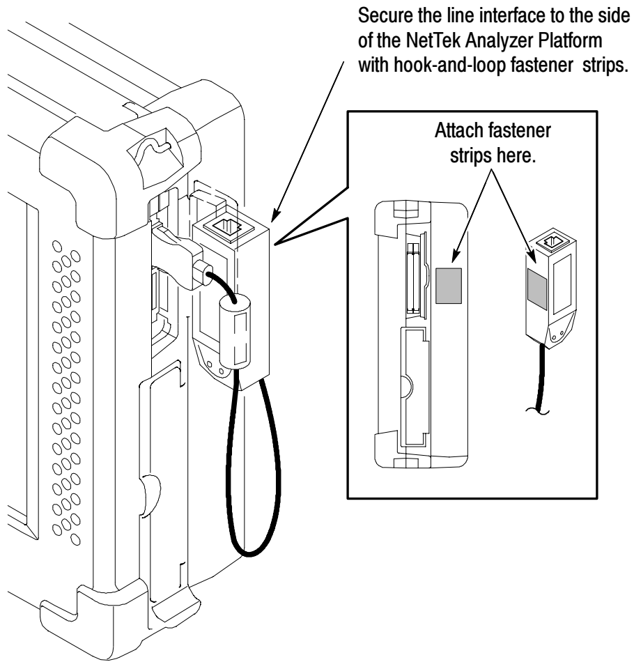
Figure 1-6: Attaching the line interface to the NetTek Analyzer Platform
