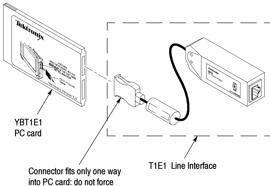
Figure 1-4: Connect the T1E1 Line Interface to the YBT1E1 Tester
