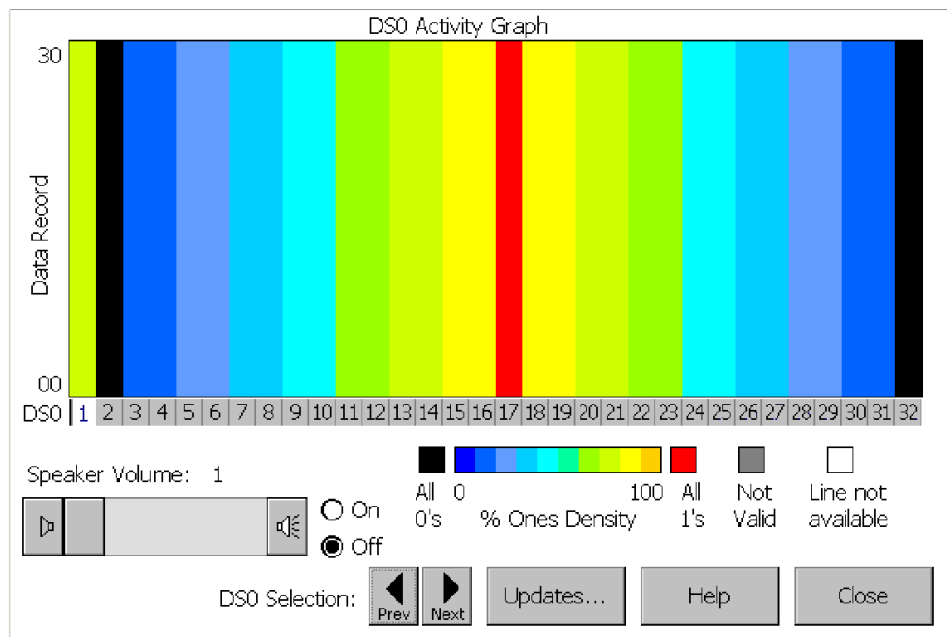
Figure 3-12: The Drop DSO view
