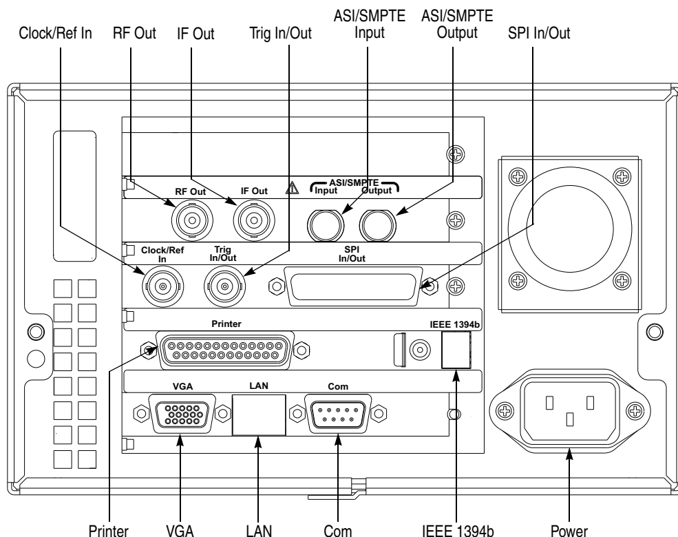
Figure 2-2: RTX130A rear panel
