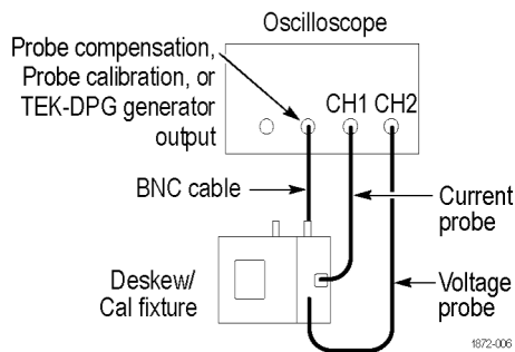
Figure 1: Typical small current probe connection
