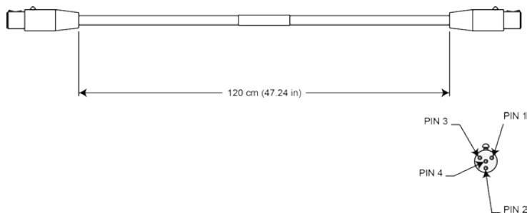
Figure 2: Model 8020-ILC-1 interlock cable dimensions
