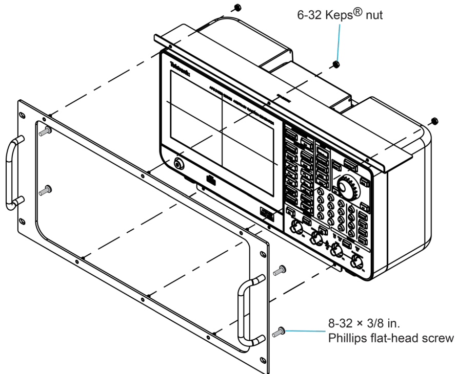
Figure 7: AFG31000-RMK front bracket installation
