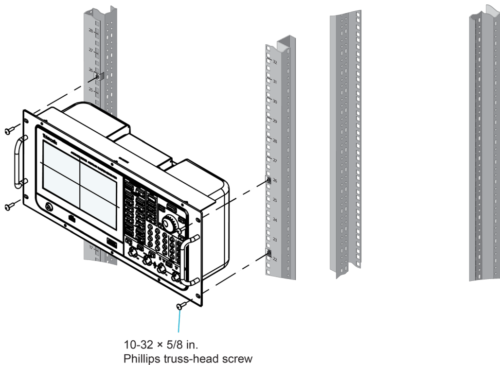
Figure 8: AFG31000-RMK rack installation
