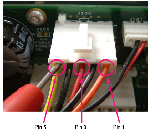
Figure 34: PWR board test points (J104)
