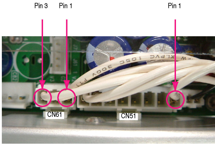
Figure 35: Secondary power supply test points (CN51 and CN61)
