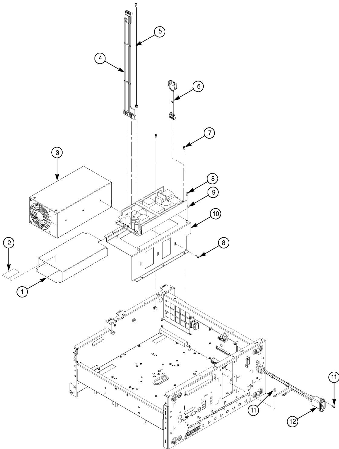
Figure 50: Power supply assembly
