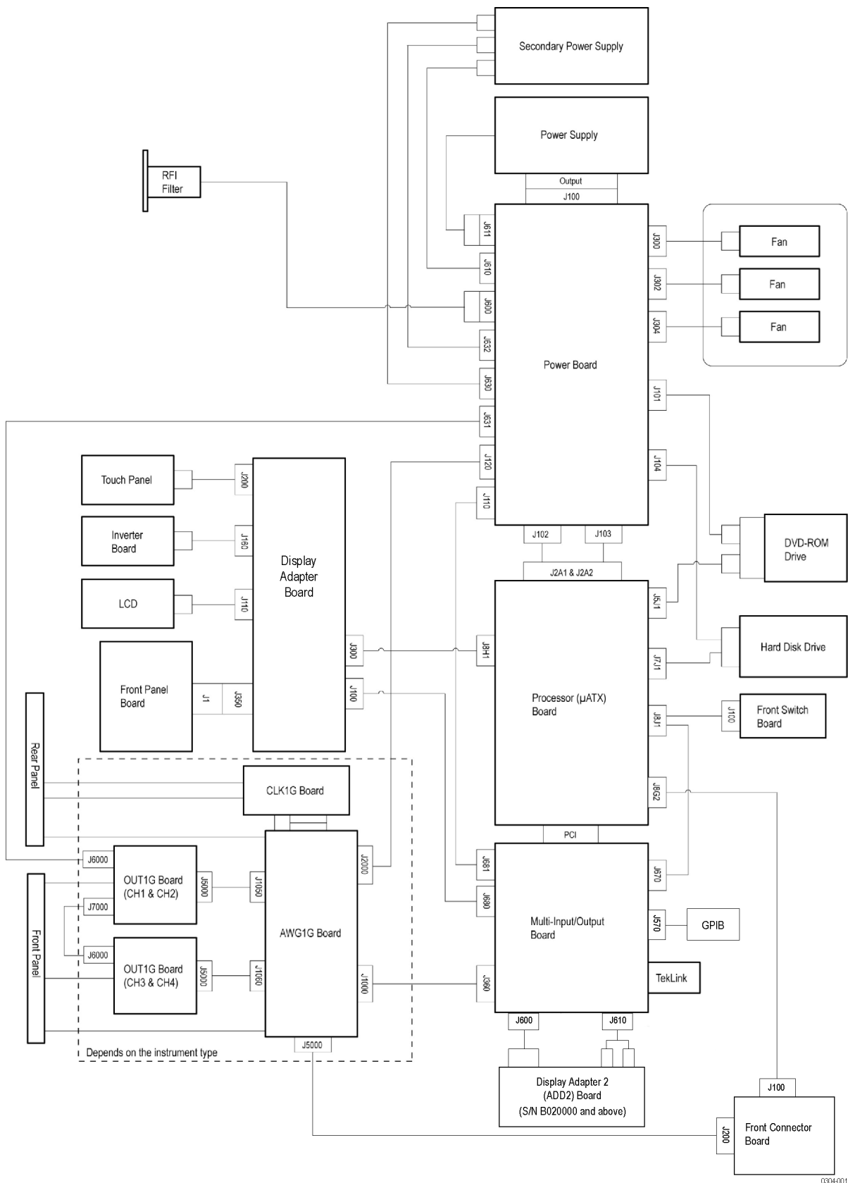
Figure 2: AWG5000B Series block diagram
