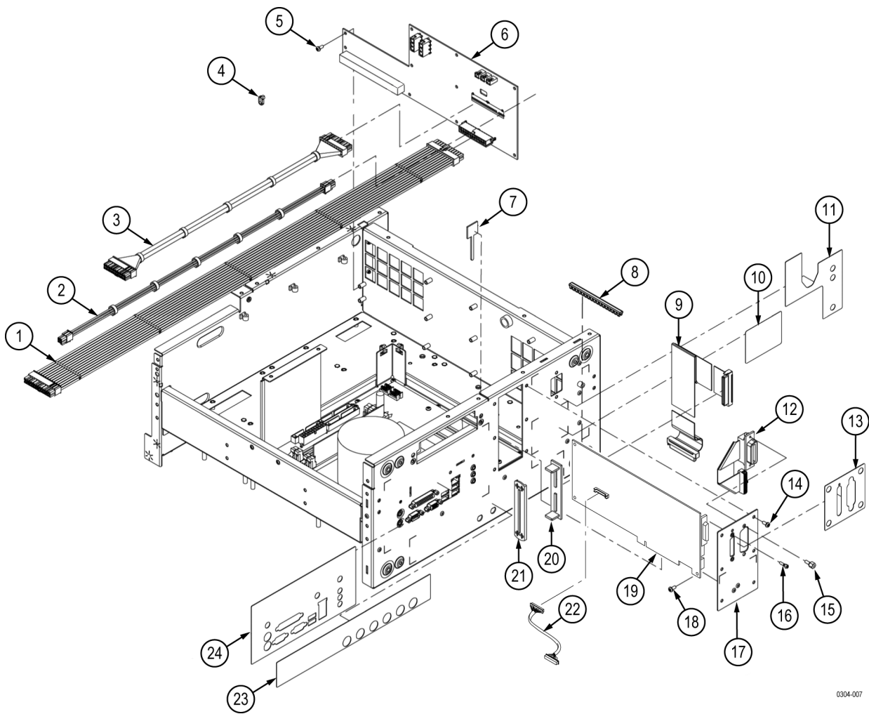
Figure 51: AWG5000C Series PCI/power interface module
