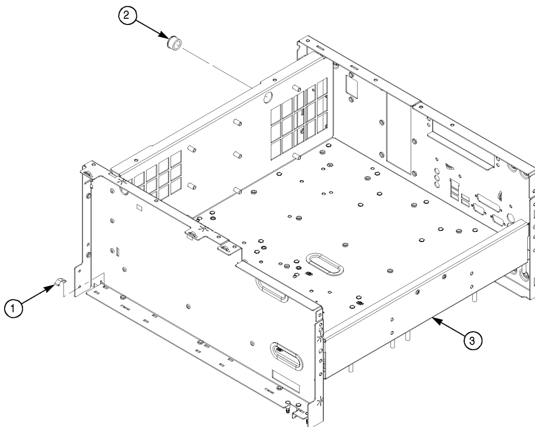
Figure 43: AWG5000B Series Chassis assembly
