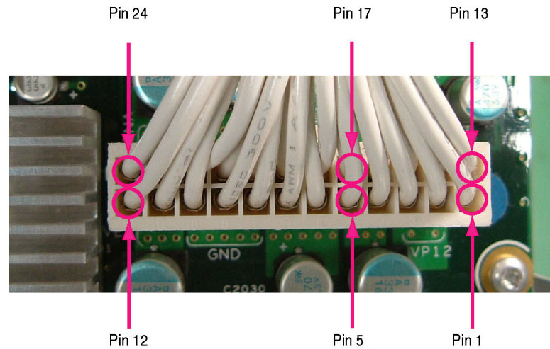
Figure 36: AWG1G board test points (J2000)
