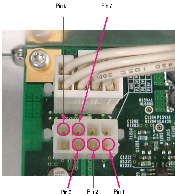
Figure 37: OUT1G board test points (J7000)
