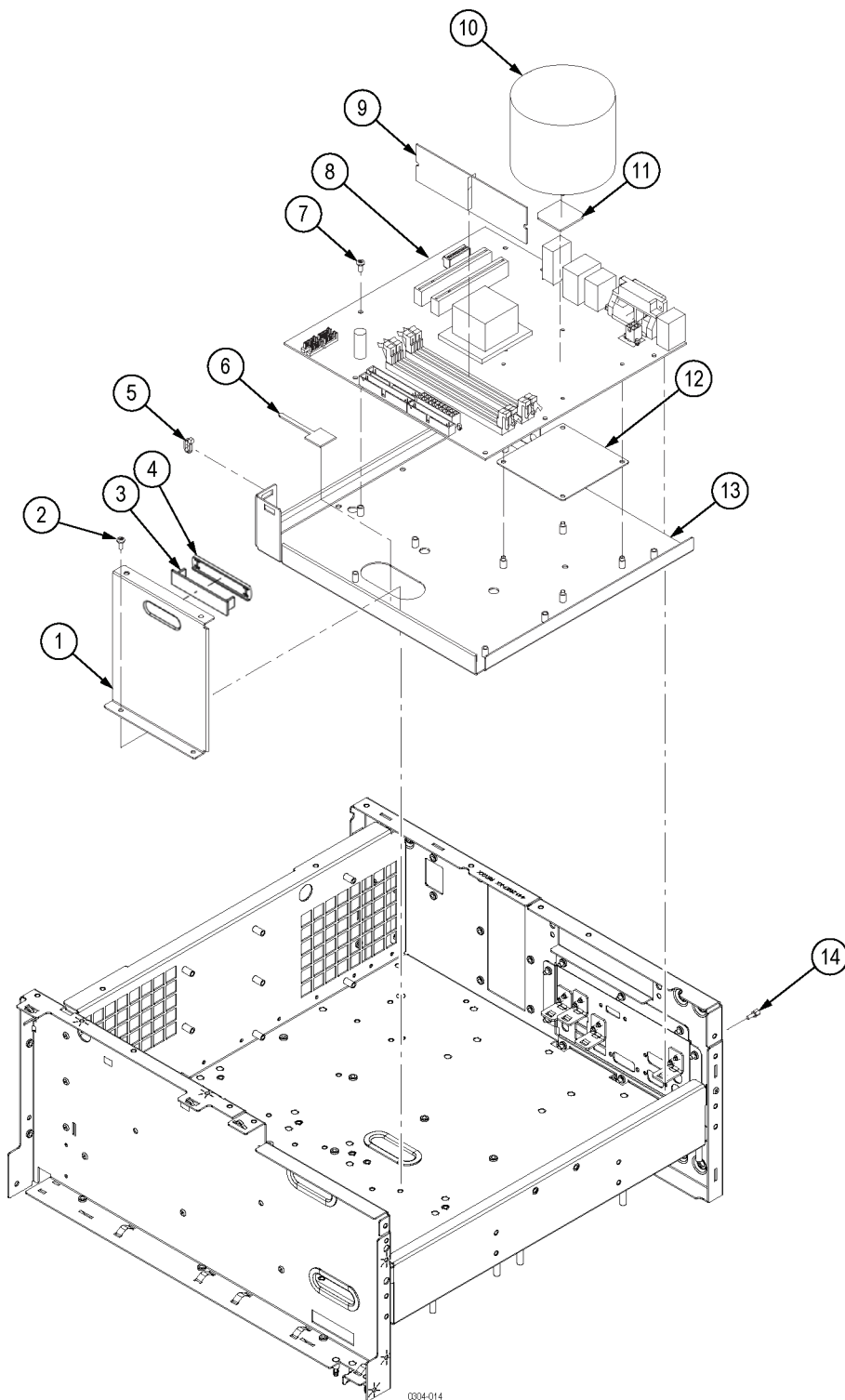
Figure 48: AWG5000C Series Processor module
