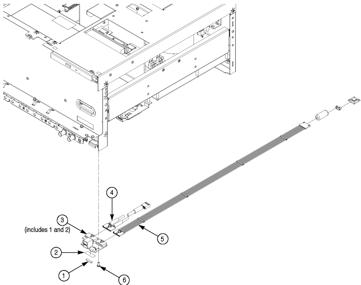
Figure 54: USB module
