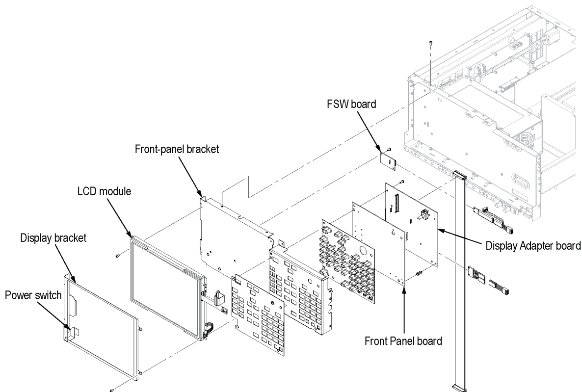
Figure 11: Disassembly of front-panel assembly (AWG5000C Series)
