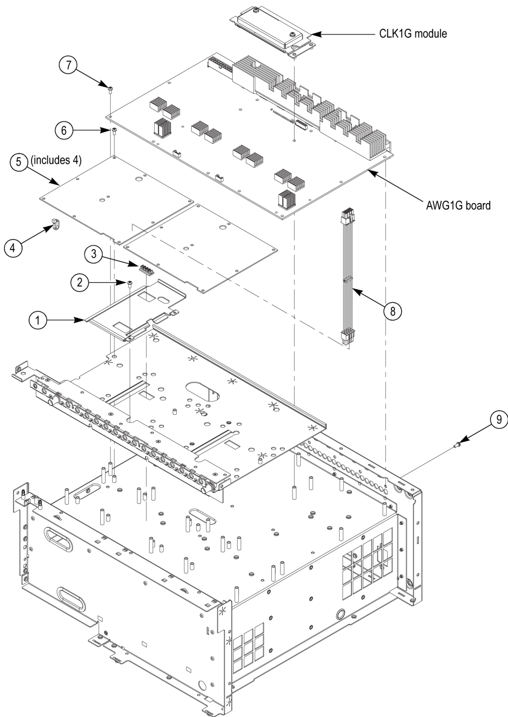
Figure 55: AWG1G/CLK1G/OUT1G modules
