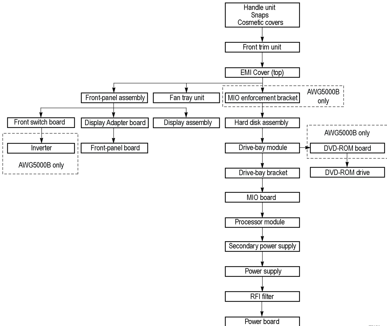
Figure 6: Disassembly procedures for external modules and internal modules (top)
