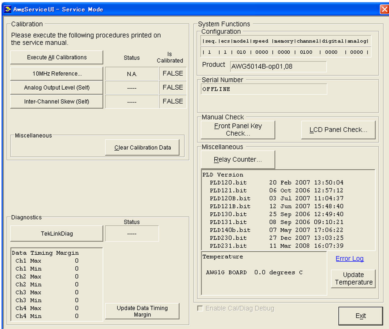
Figure 3: Service UI menu
