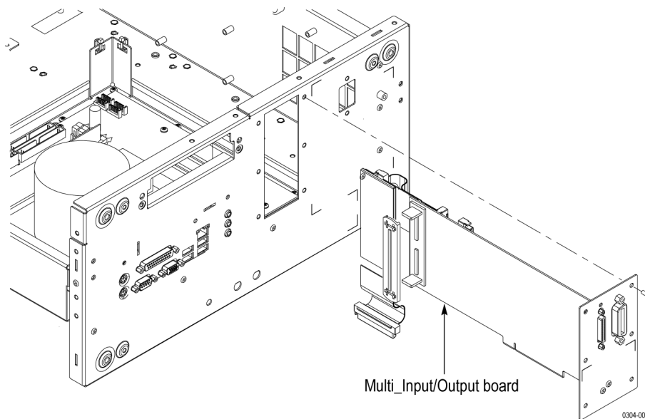
Figure 15: Multi-Input/Output removal (AWG5000C Series)
