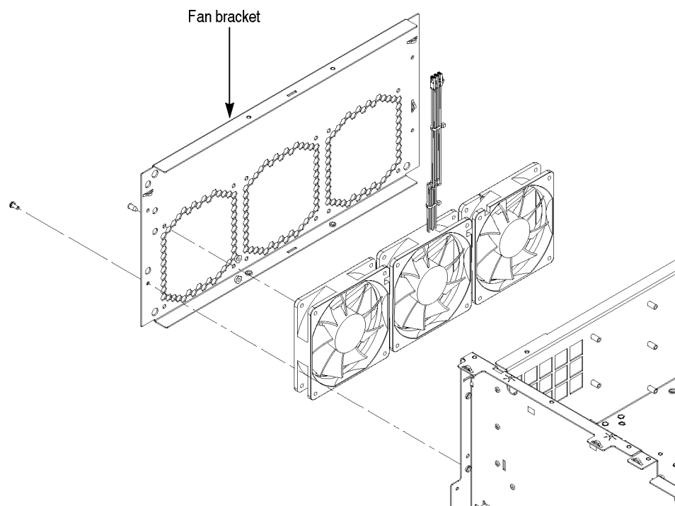
Figure 10: Fan tray unit removal
