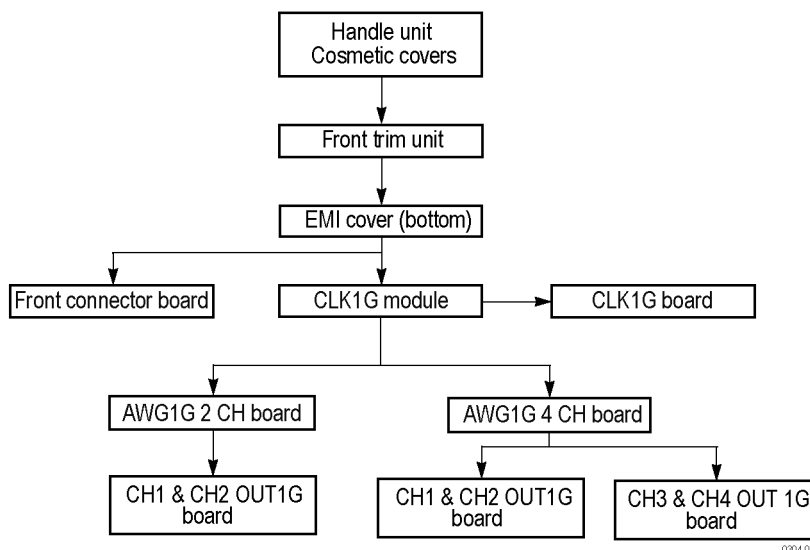
Figure 7: Disassembly procedures for internal modules (bottom)
