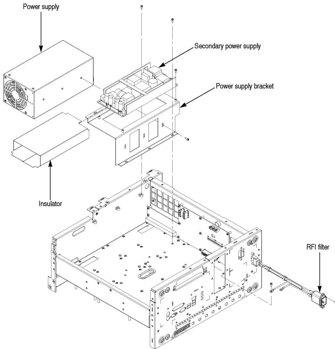
Figure 17: Secondary power supply, power supply, and RFI filter removal
