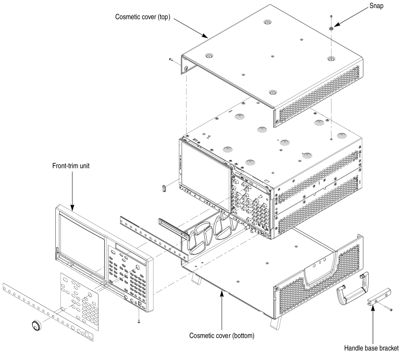
Figure 8: Handle, snaps, cosmetic covers, and front-trim unit removal
