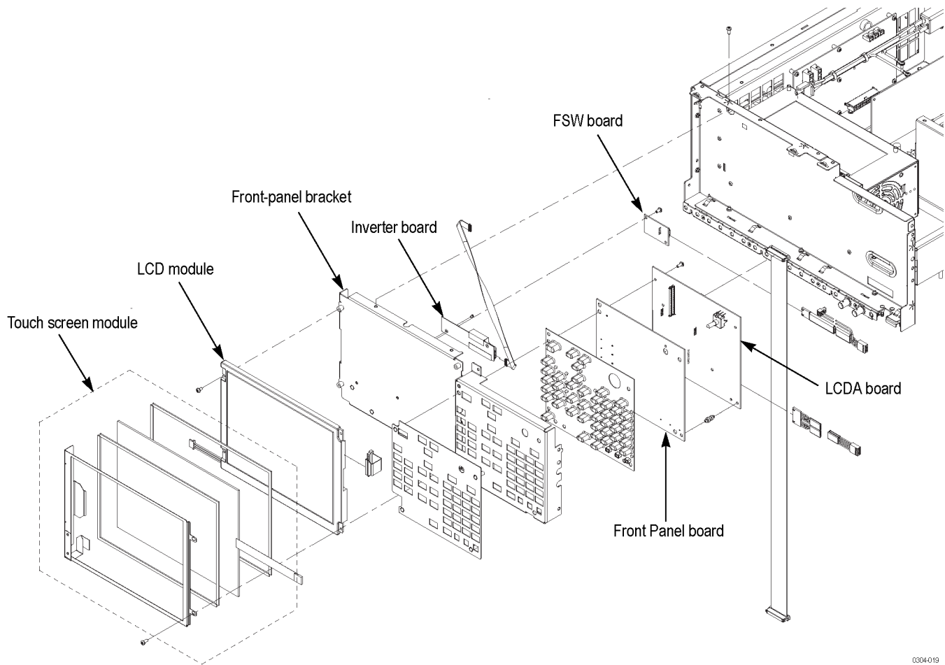
Figure 12: Disassembly of front-panel assembly (AWG5000B Series)
