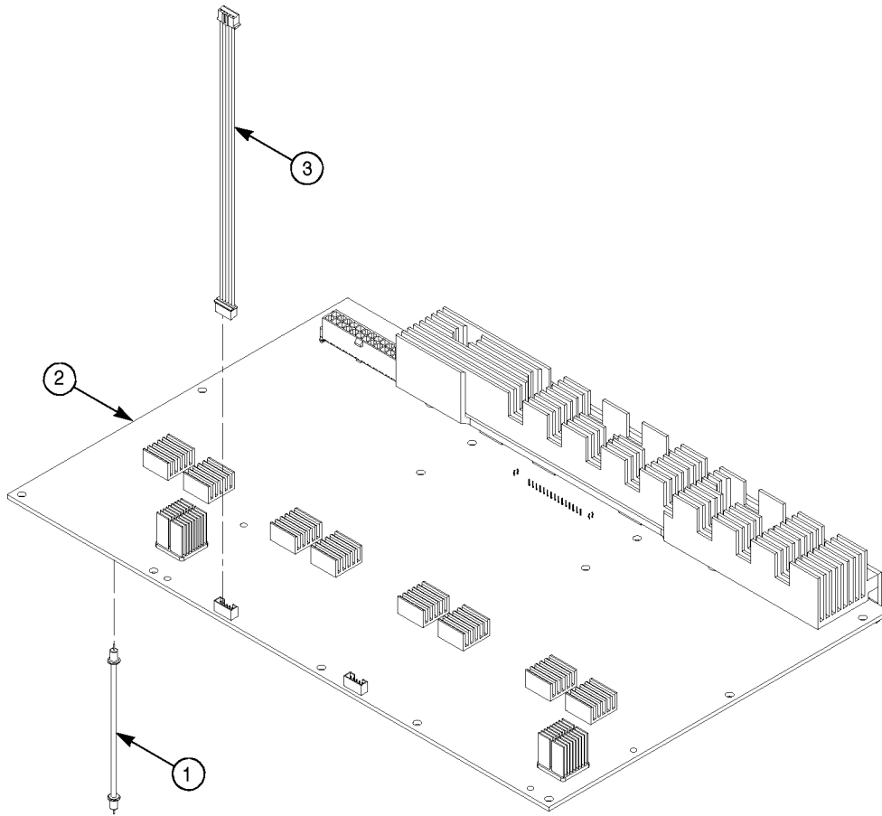
Figure 57: AWG1G module
