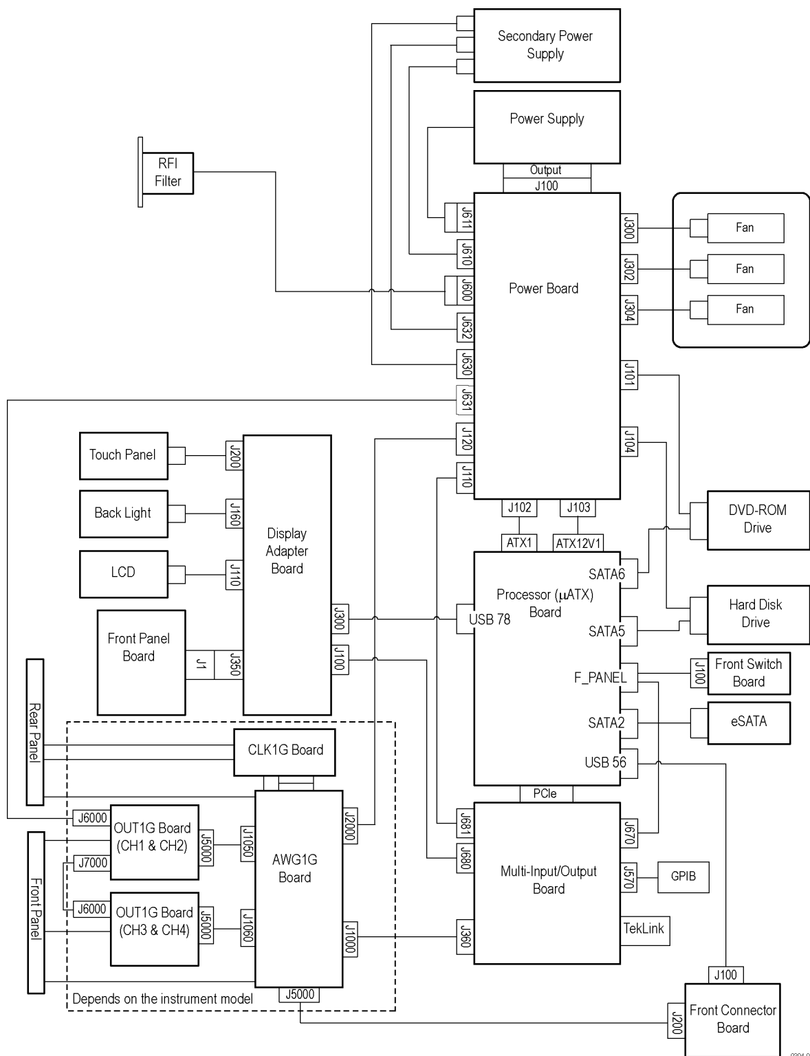
Figure 1: AWG5000C Series block diagram
