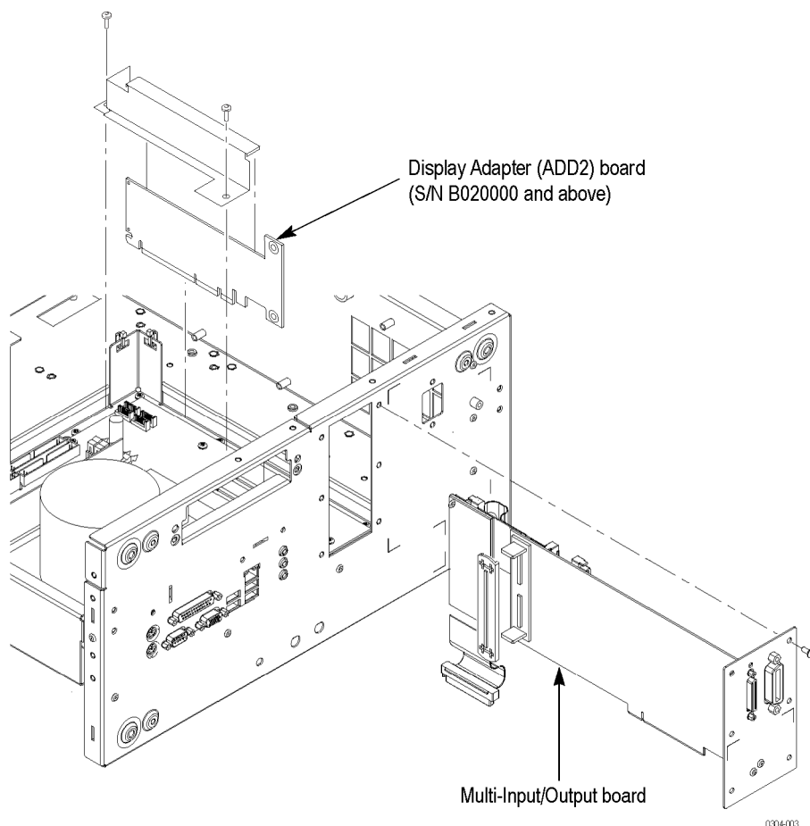
Figure 22: Multi-Input/Output and Display Adapter board removal (AWG5000B Series)
