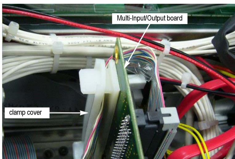
Figure 21: Removing the clamp cover
