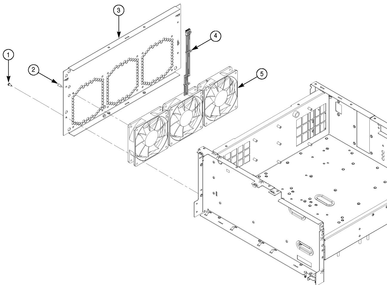
Figure 53: Fan tray assembly
