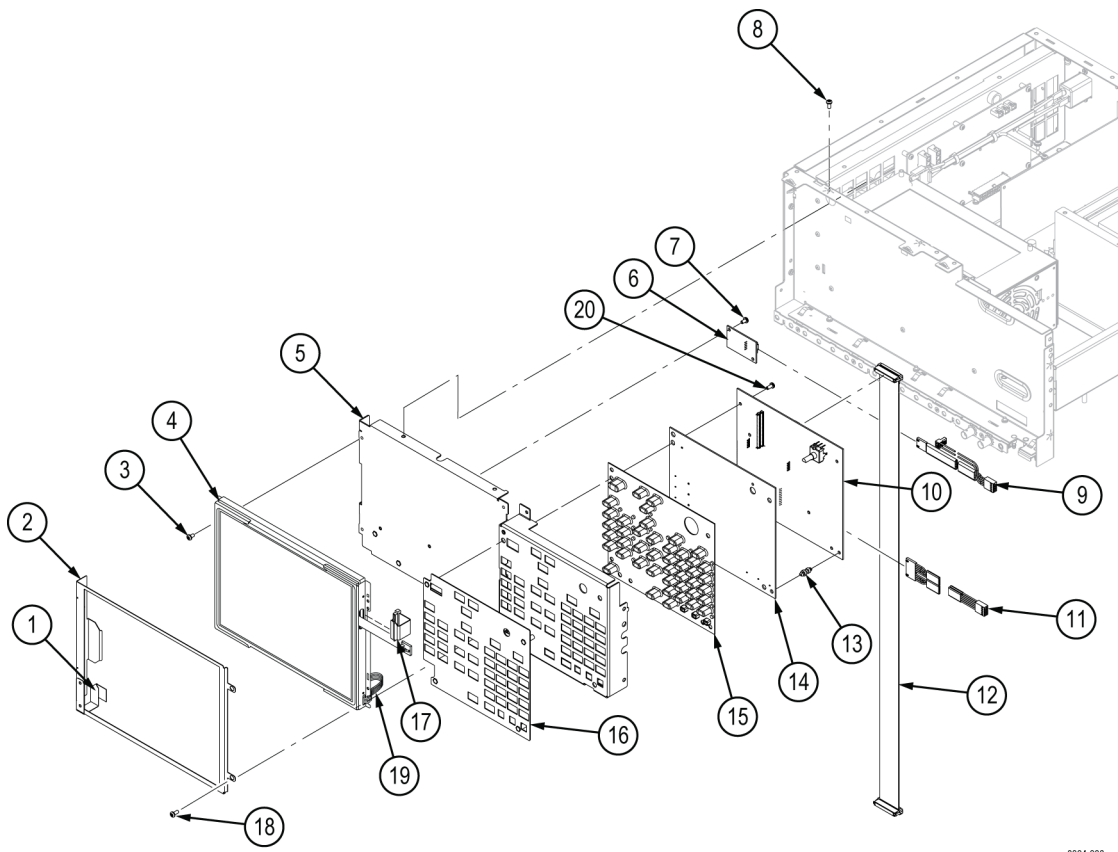
Figure 44: AWG5000C Series front-panel assembly
