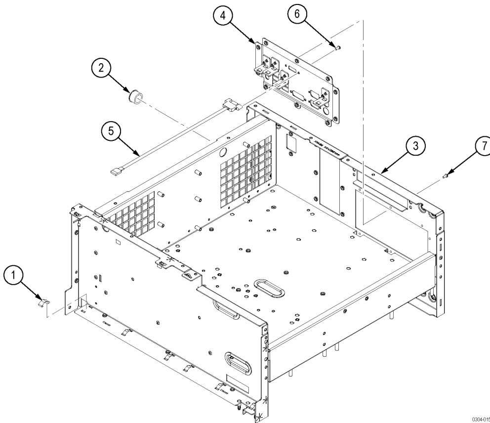
Figure 42: AWG5000C Series Chassis assembly
