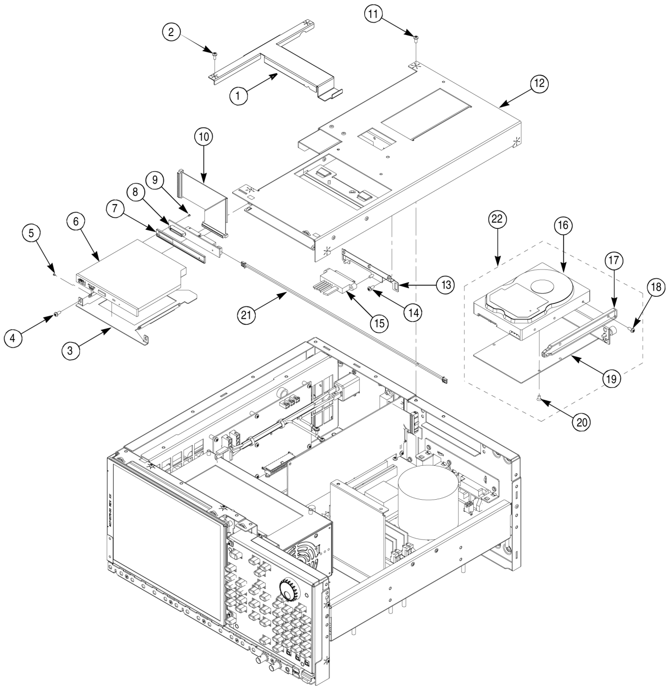
Figure 47: AWG5000B Series drive modules
