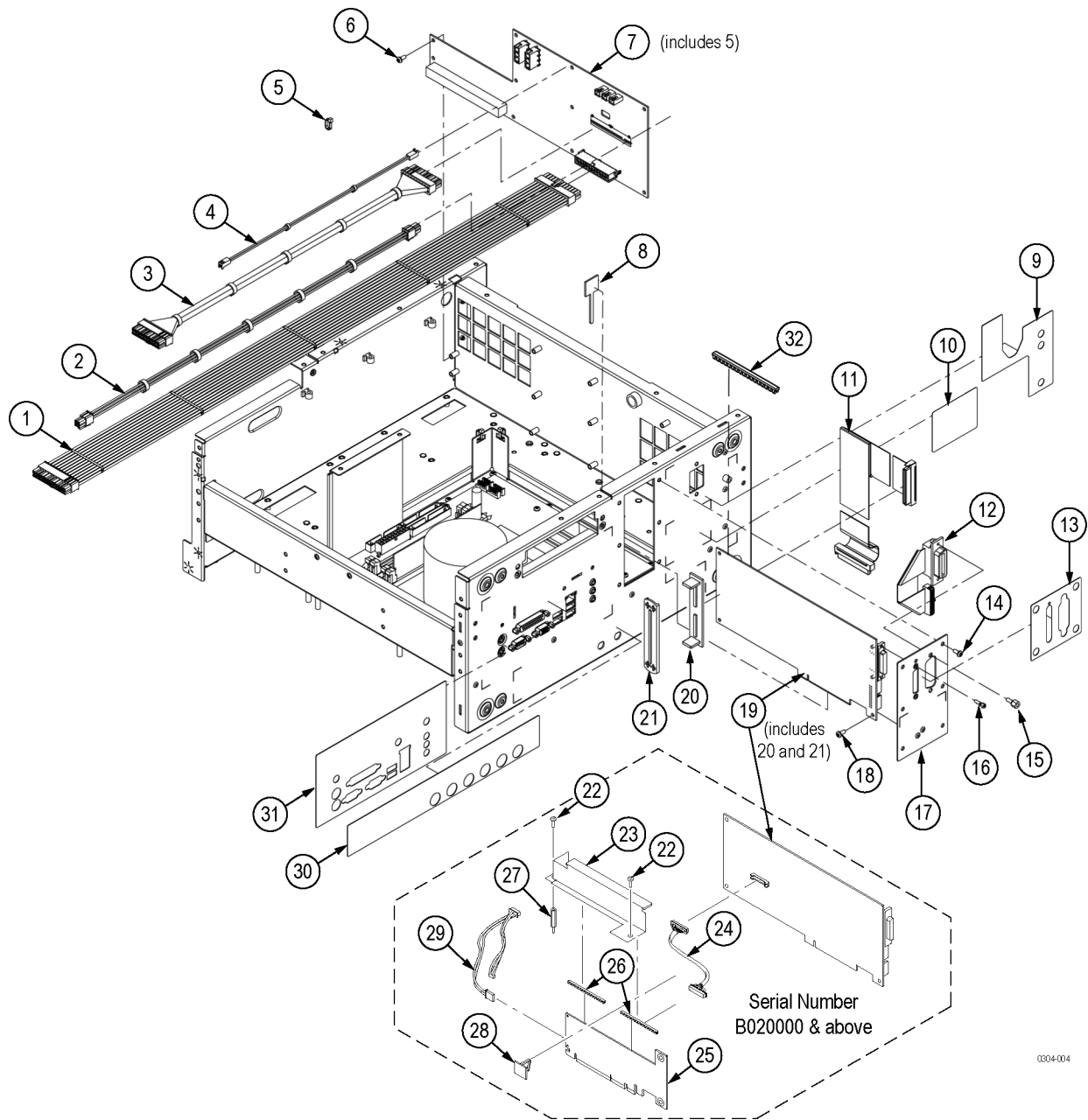
Figure 52: AWG5000B Series PCI/power interface module
