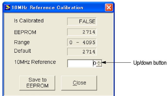
Figure 5: 10 MHz Reference Calibration dialog box
