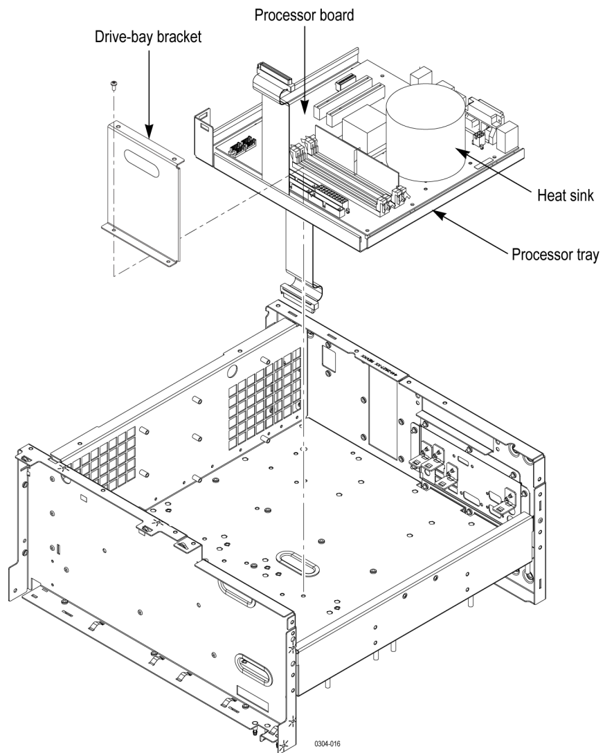
Figure 16: Processor board removal (AWG5000C Series)
