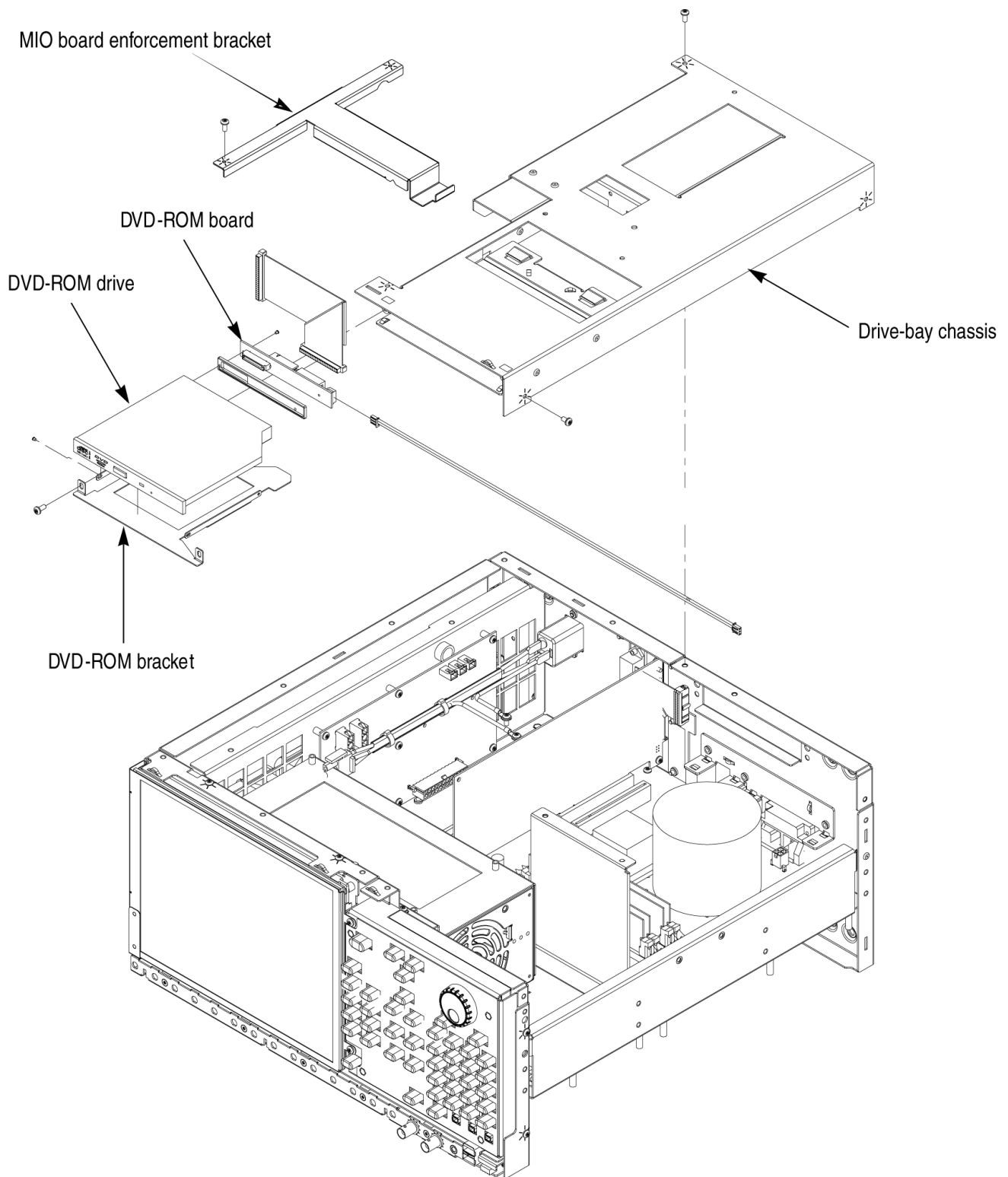
Figure 20: Drive module removal (AWG5000B)
