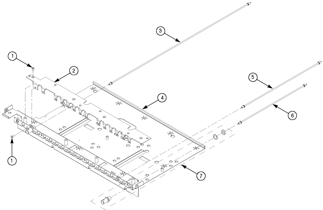
Figure 58: BNC bracket
