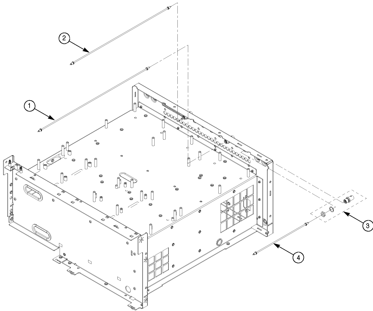
Figure 59: Rear connectors
