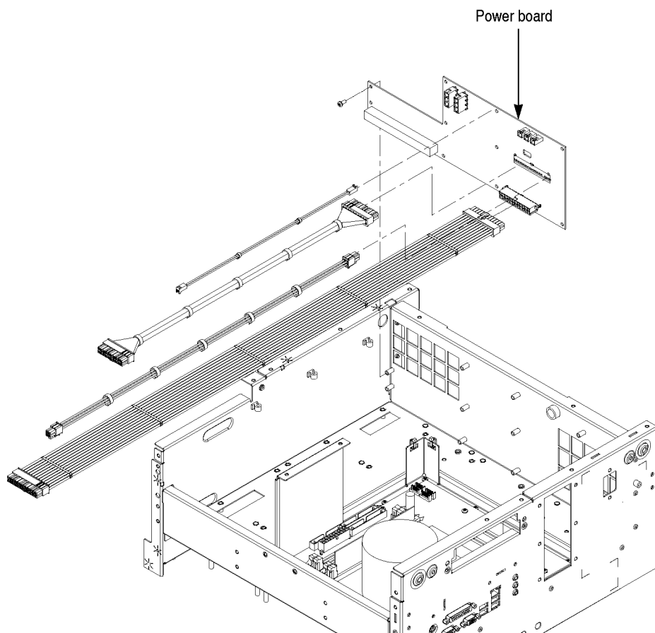
Figure 25: Power board removal
