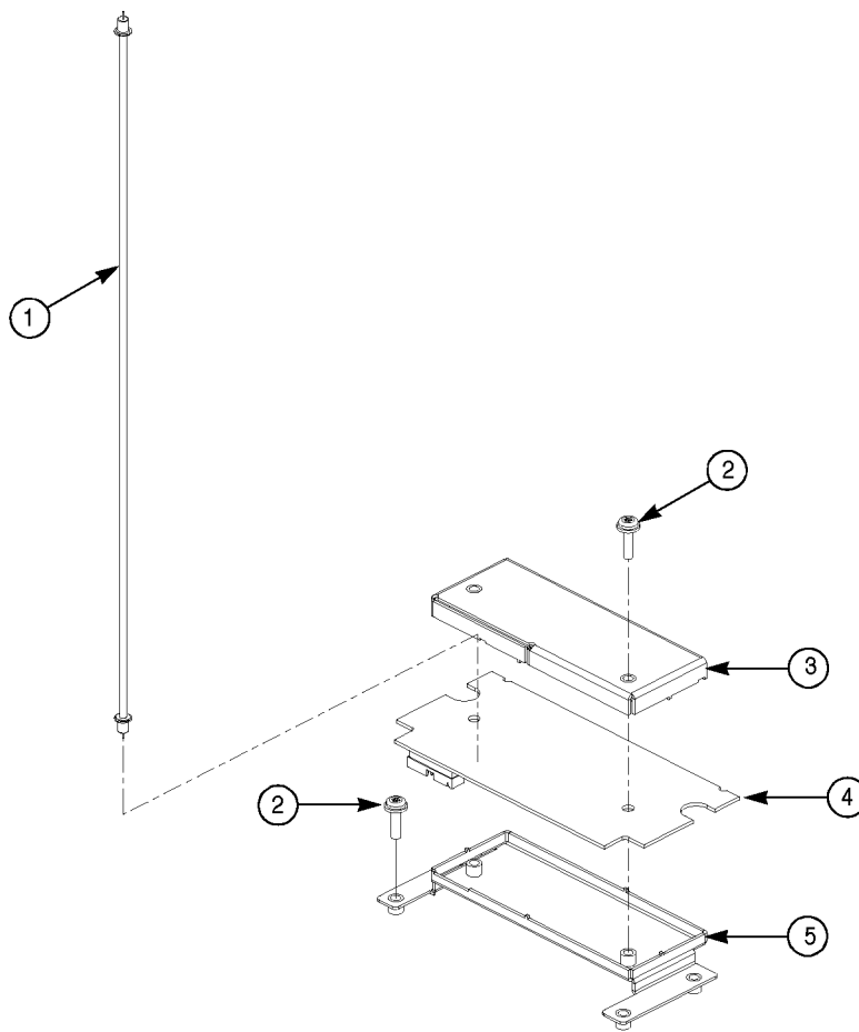
Figure 56: CLK1G module
