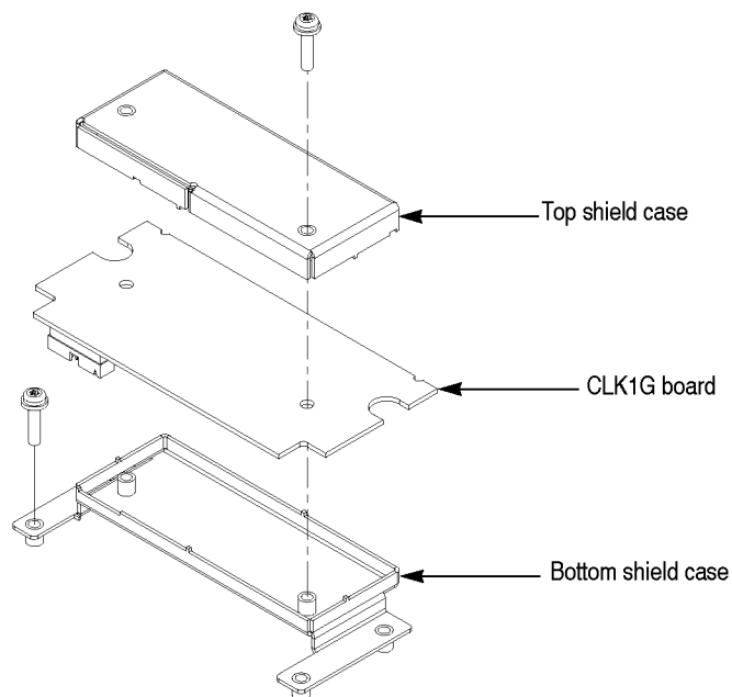
Figure 27: Disassembly of the CLK1G module
