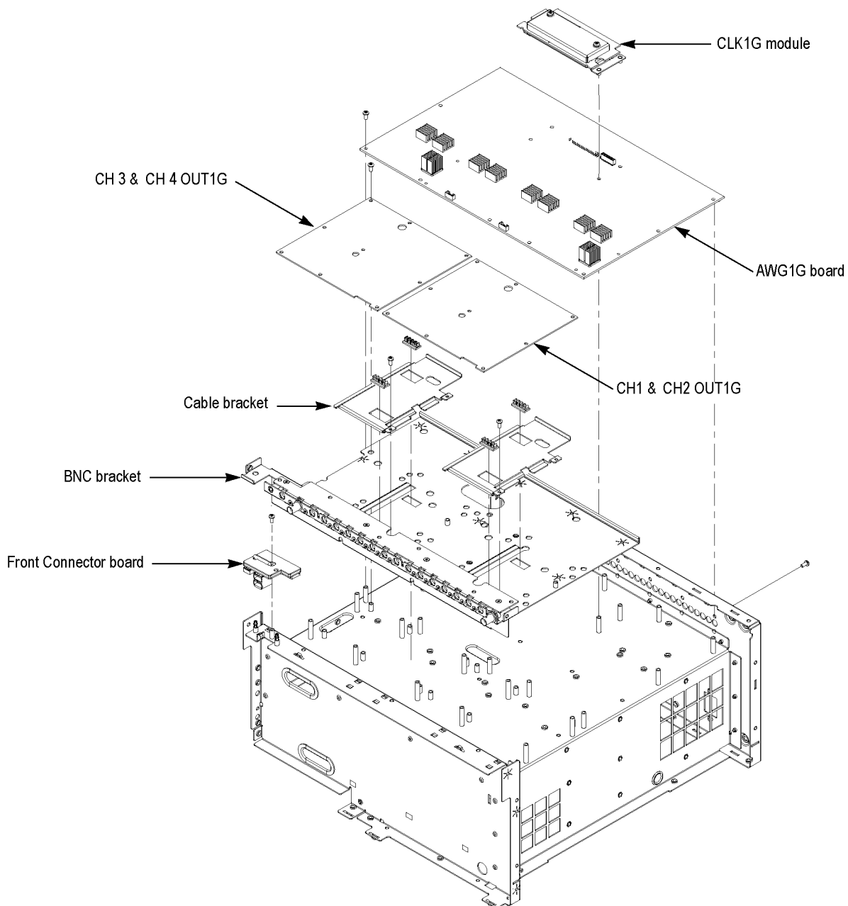
Figure 26: Front Connector board, CLK1G module, AWG1G board, and OUT1G boards removal (4-channel model)
