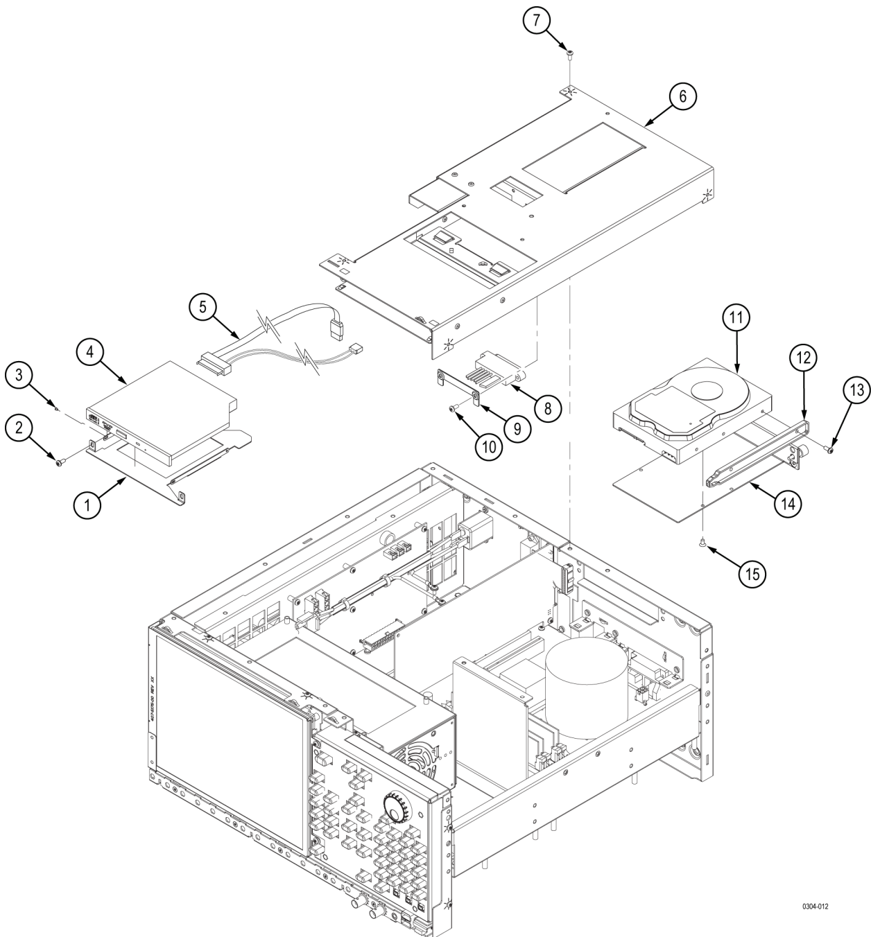
Figure 46: AWG5000C Series drive modules
