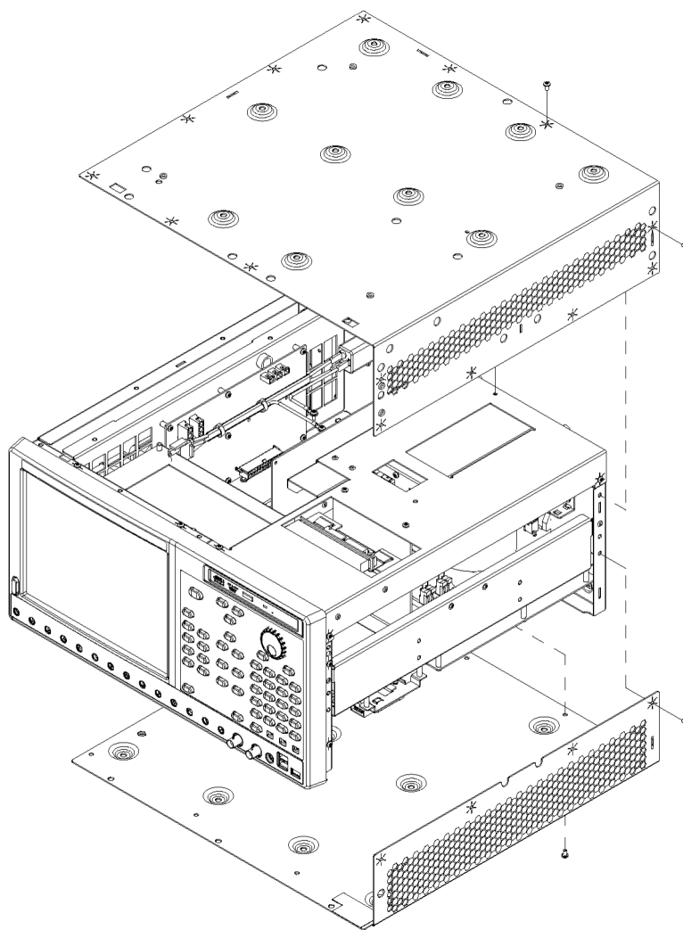
Figure 9: EMI cover removal
