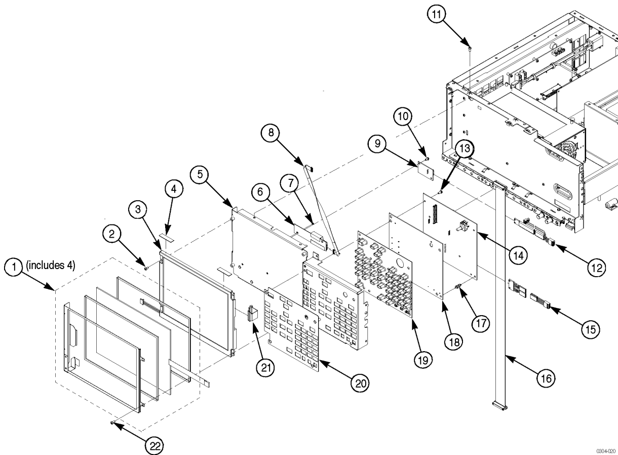
Figure 45: AWG5000B Series front-panel assembly
