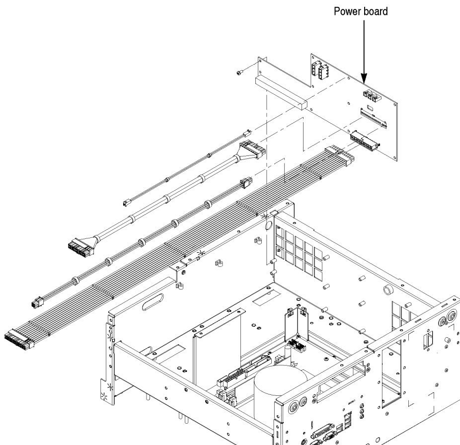
Figure 18: Power board removal
