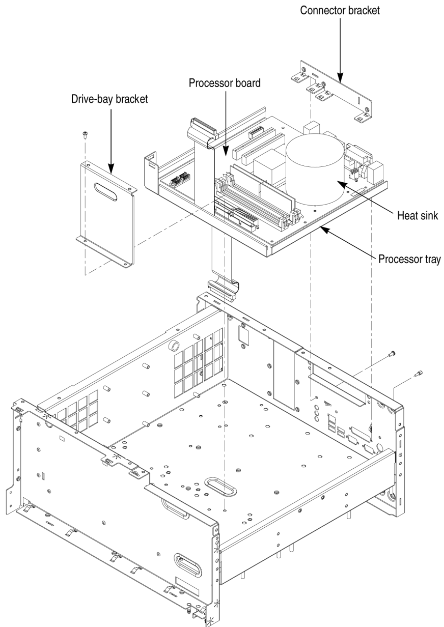
Figure 23: Processor board removal (AWG5000B Series)
