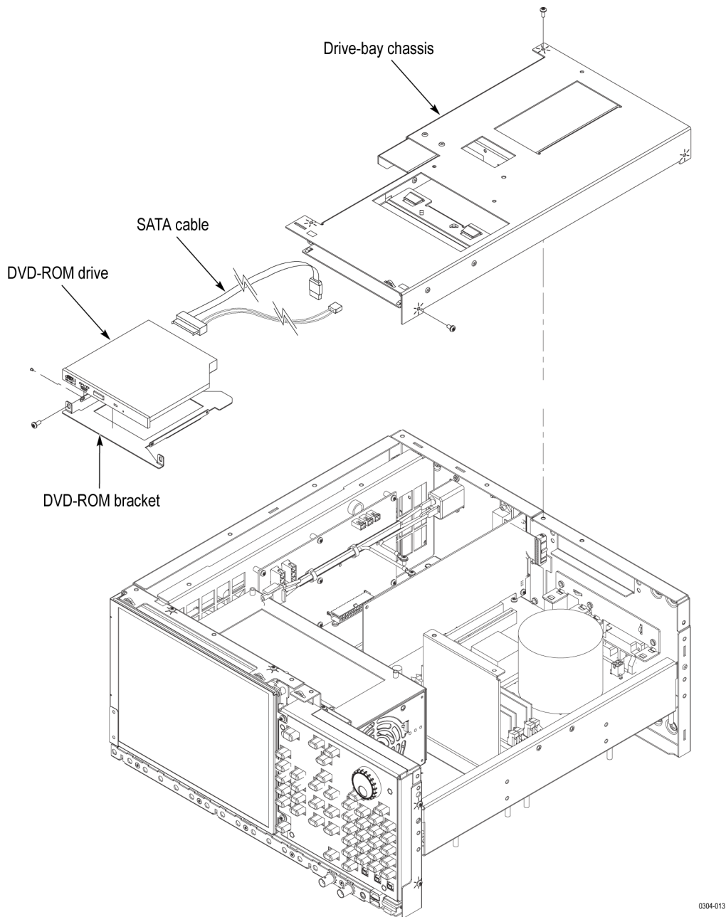
Figure 14: Drive module removal (AWG5000C Series)
