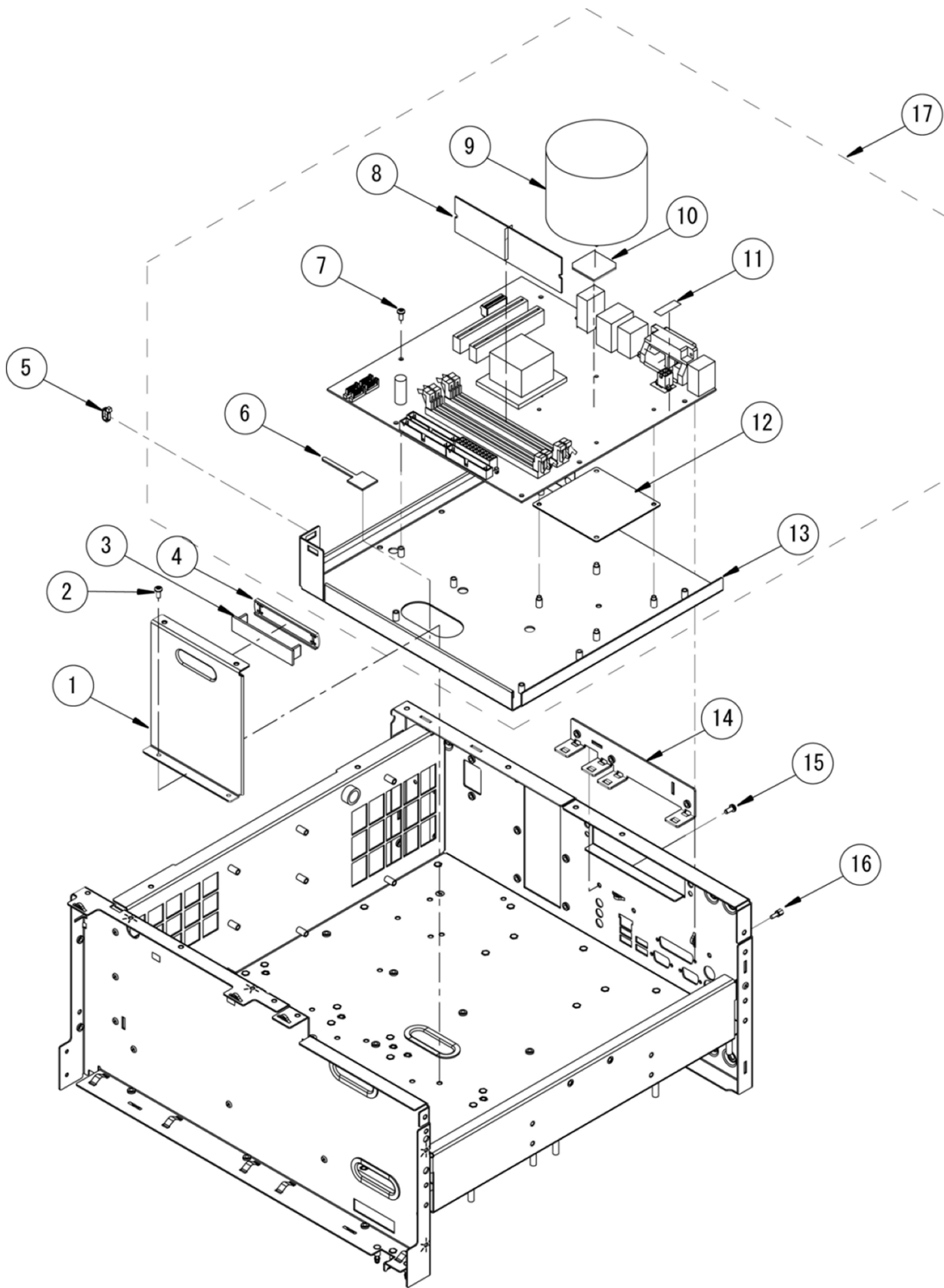
Figure 49: AWG5000B Series Processor module
