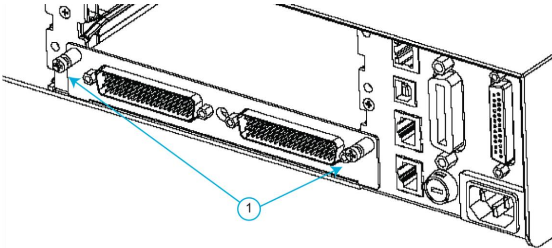
Figure 9: Check 3700A card mounting screws
