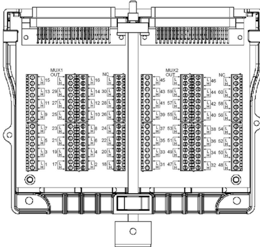
Figure 5: Model 3724-ST Screw-Terminal Accessory
