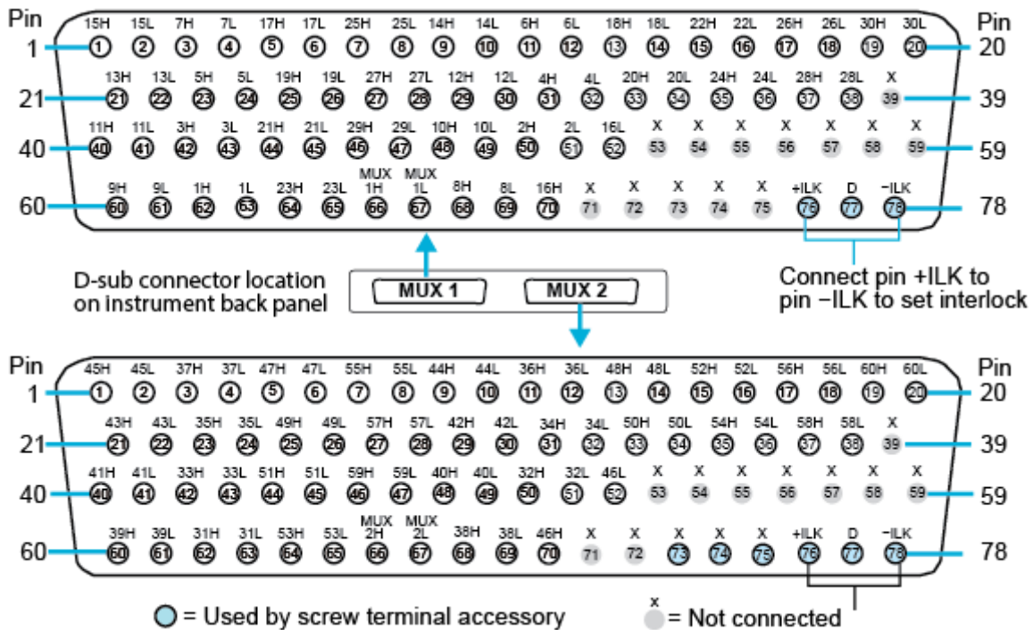
Figure 3: 3724 D-sub connections
