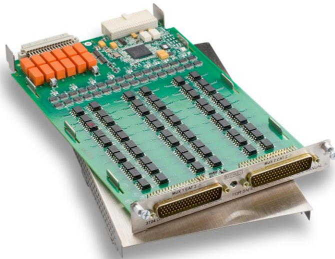
Figure 1: Model 3724 Dual 1 x 30 Multiplexer Card
