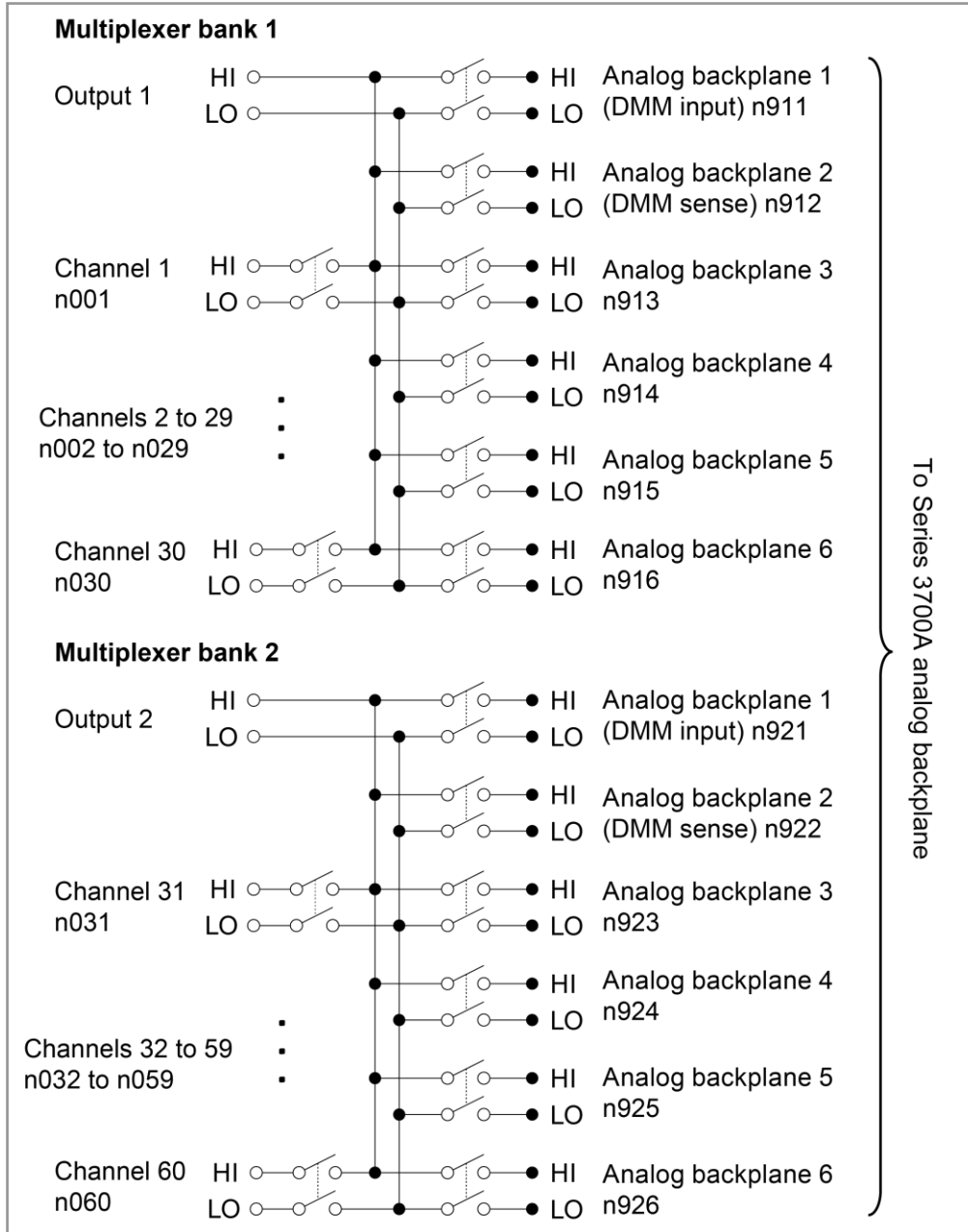
Figure 4: Model 3724 schematic
