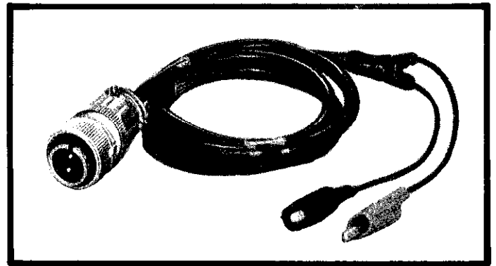
FIGURE 4. Model 1481 Low-Thermal Input Cable. The Model 1482 Low-Thermal Input Cable is similar except it has bare copper leads instead of alligator clips.
