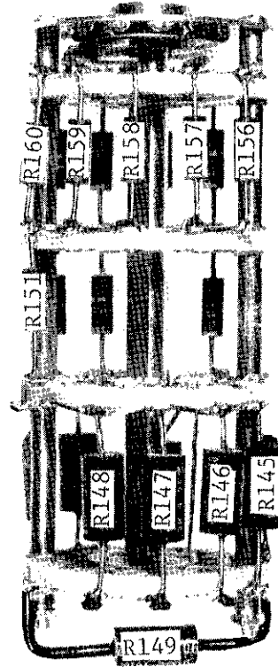
FIGURE 40. Resistor Locations on RANGE Switch (S102). Figure 39 shows resistors on opposite side.
