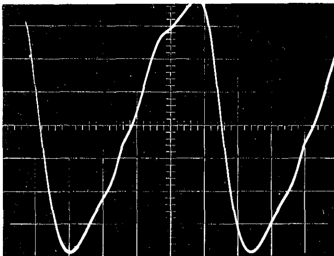
FIGURE 26. Improper Wave Forms at Point F (Figure 30) in Oscillator Circuit. Wave A indicates the wrong bias; wave B is distorted. Scale for both is 2 v/cm vertical, 2 msec/cm horizontal.
