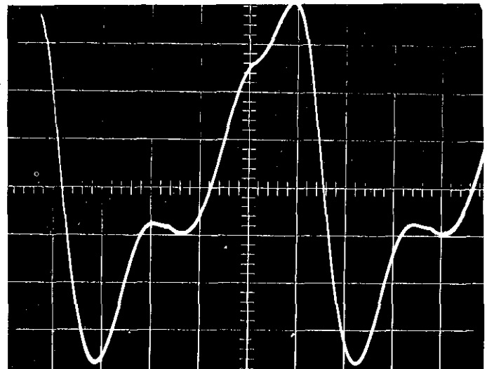
FIGURE 26. Improper Wave Forms at Point F (Figure 30) in Oscillator Circuit. Wave A indicates the wrong bias; wave B is distorted. Scale for both is 2 v/cm vertical, 2 msec/cm horizontal.
