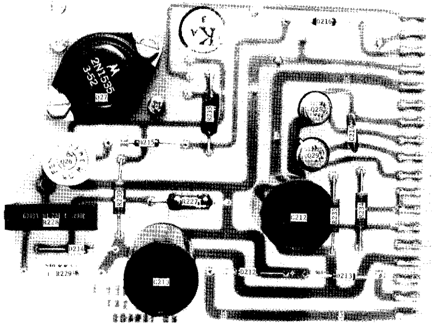
FIGURE 36. Component Locations on Printed Circuit 74, Top Face.
