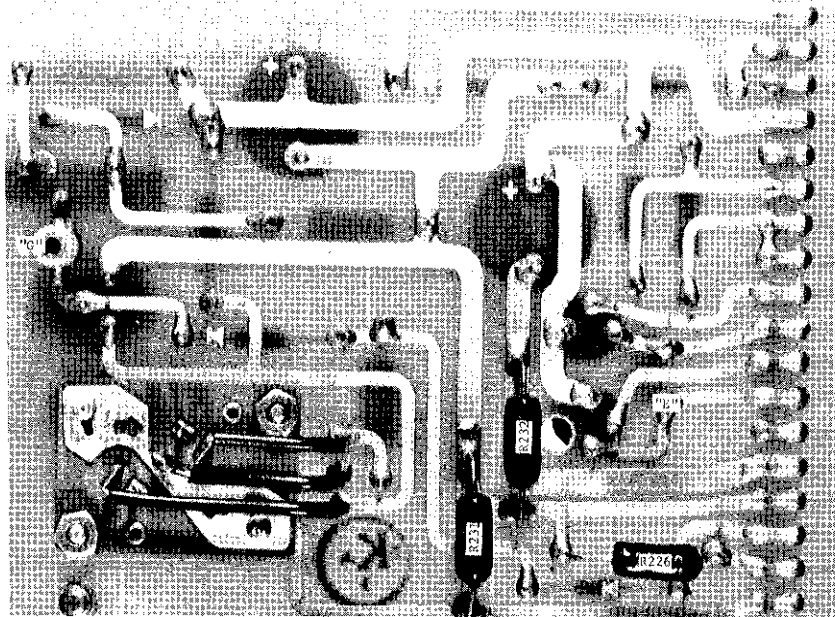
FIGURE 35. Resistor and Test Point Locations on Printed Circuit 74, Bottom Face. Connect to point E at either place, not to both points simultaneously.
