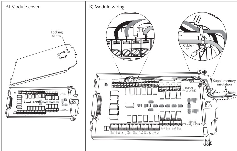
Figure 11 Model 7700 switching module
