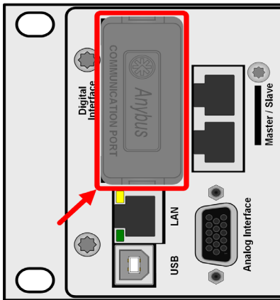
Figure 3 - Emplacement interface
