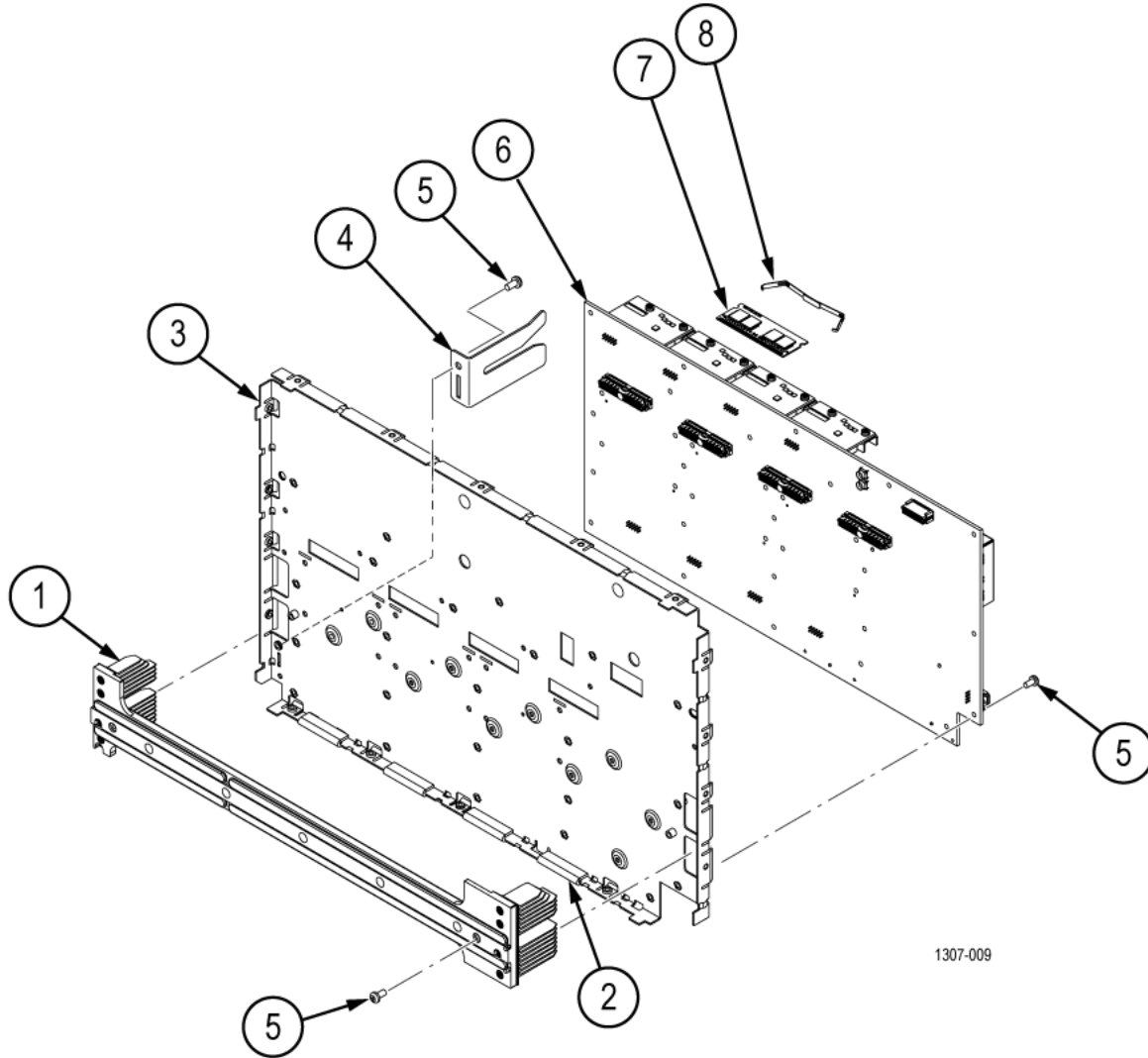
Figure 7: Mid-plane chassis exploded view
