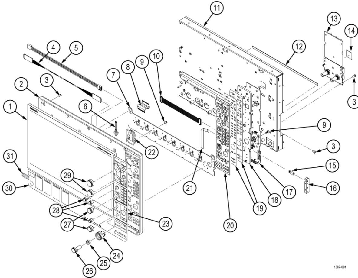
Figure 8: Front panel and display exploded view
