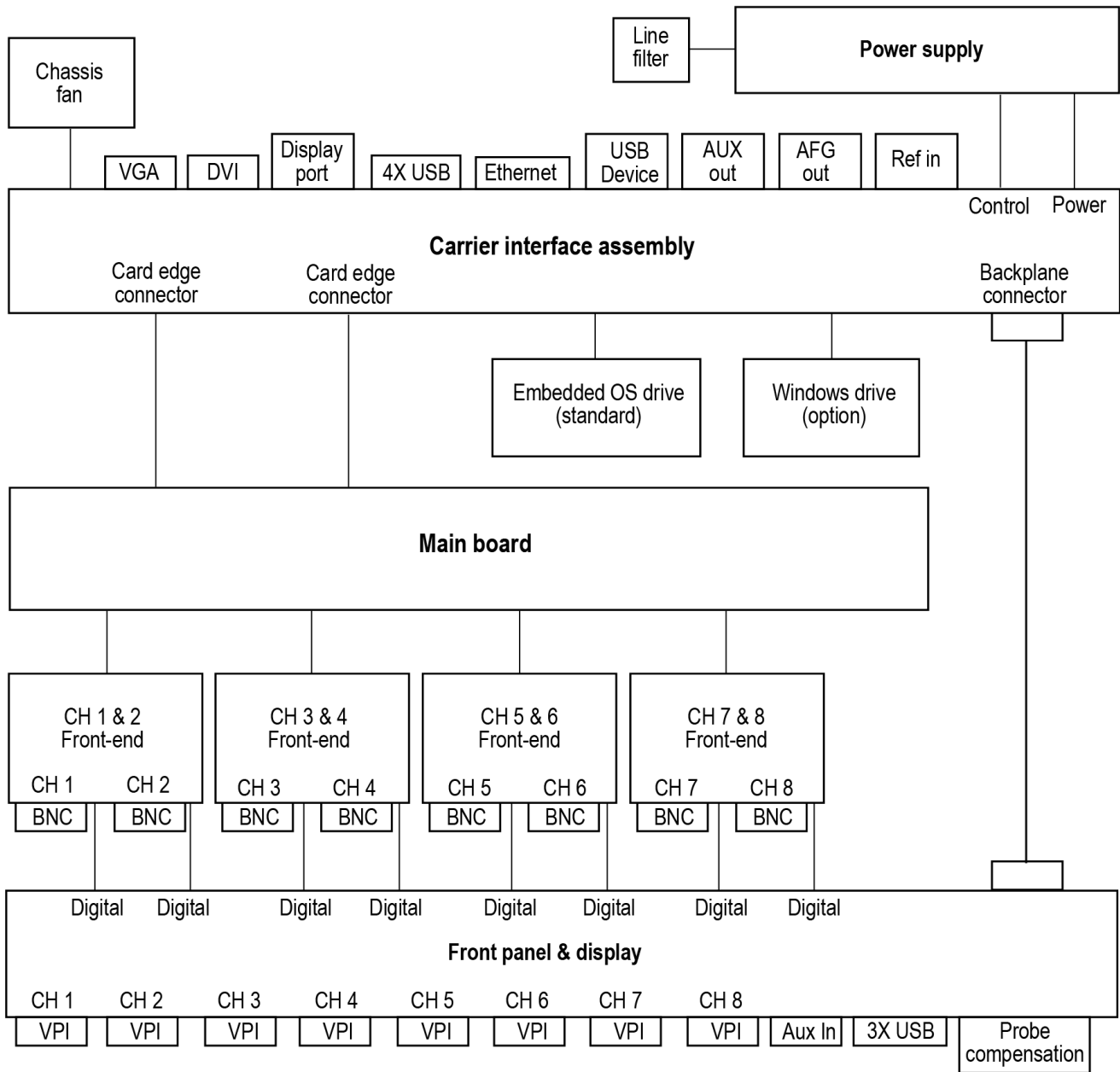
Figure 1: Block diagram
