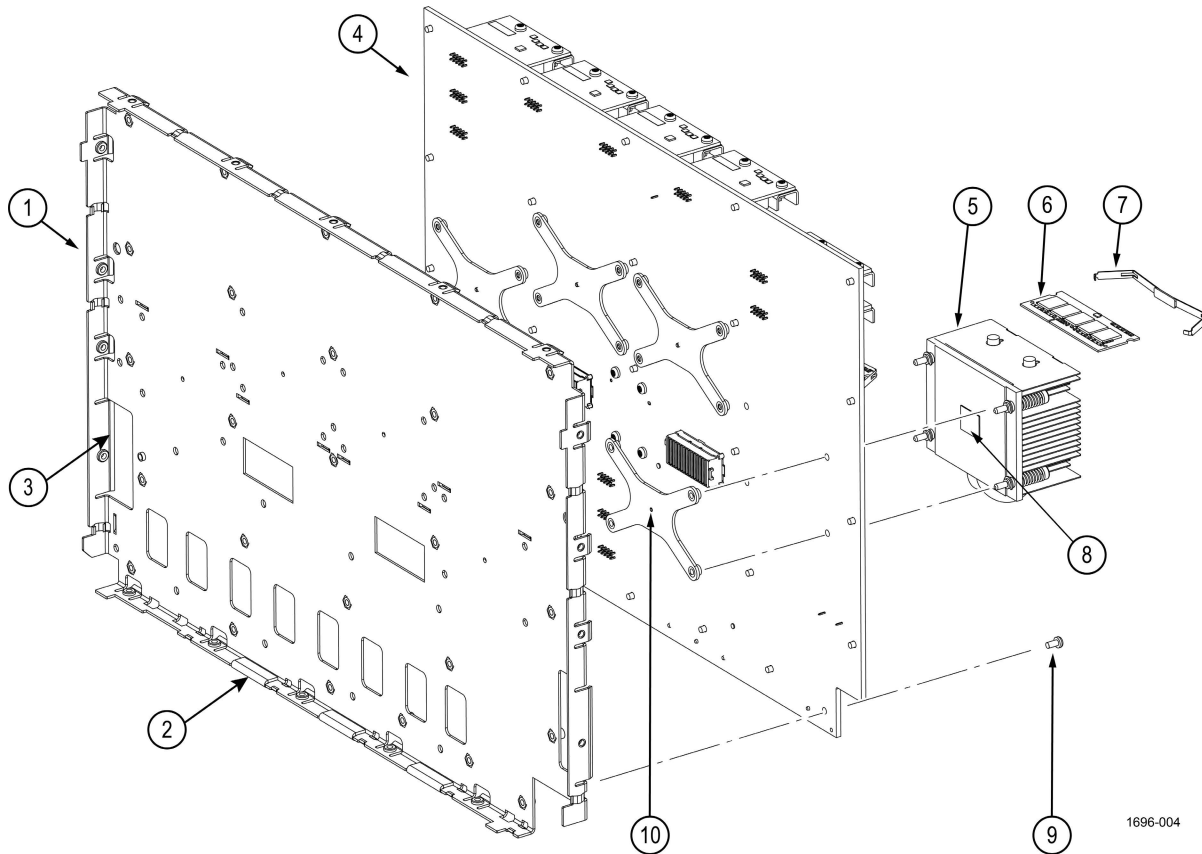
Figure 6: Mid-plane chassis exploded view
