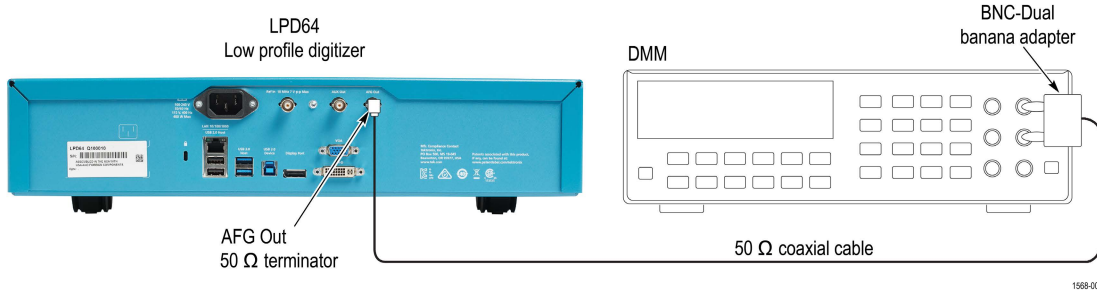
Figure 6: DC offset tests
