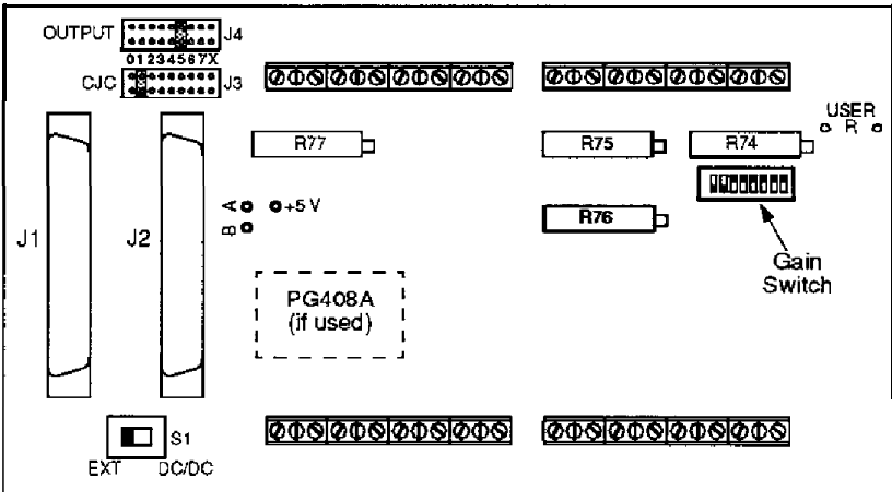
Figure 3-1. Locations of EXP-16 Key Components
