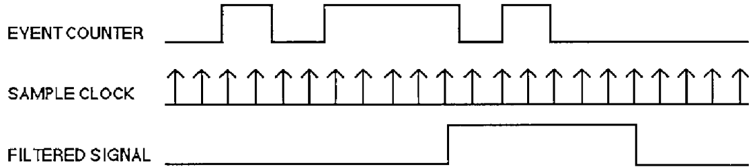
Figure 2.5 Event Counter Debounce Filter.
