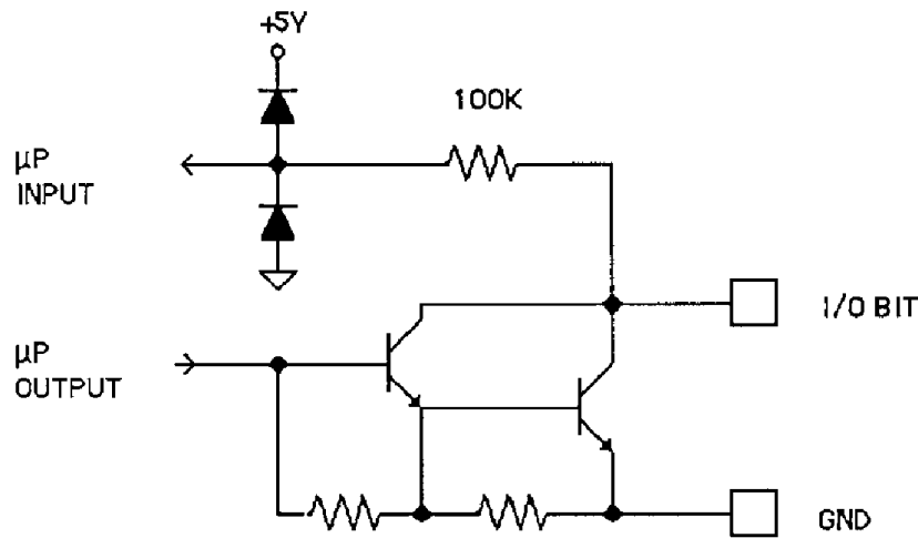
Figure 2.2 Digital I/O Circuit.
