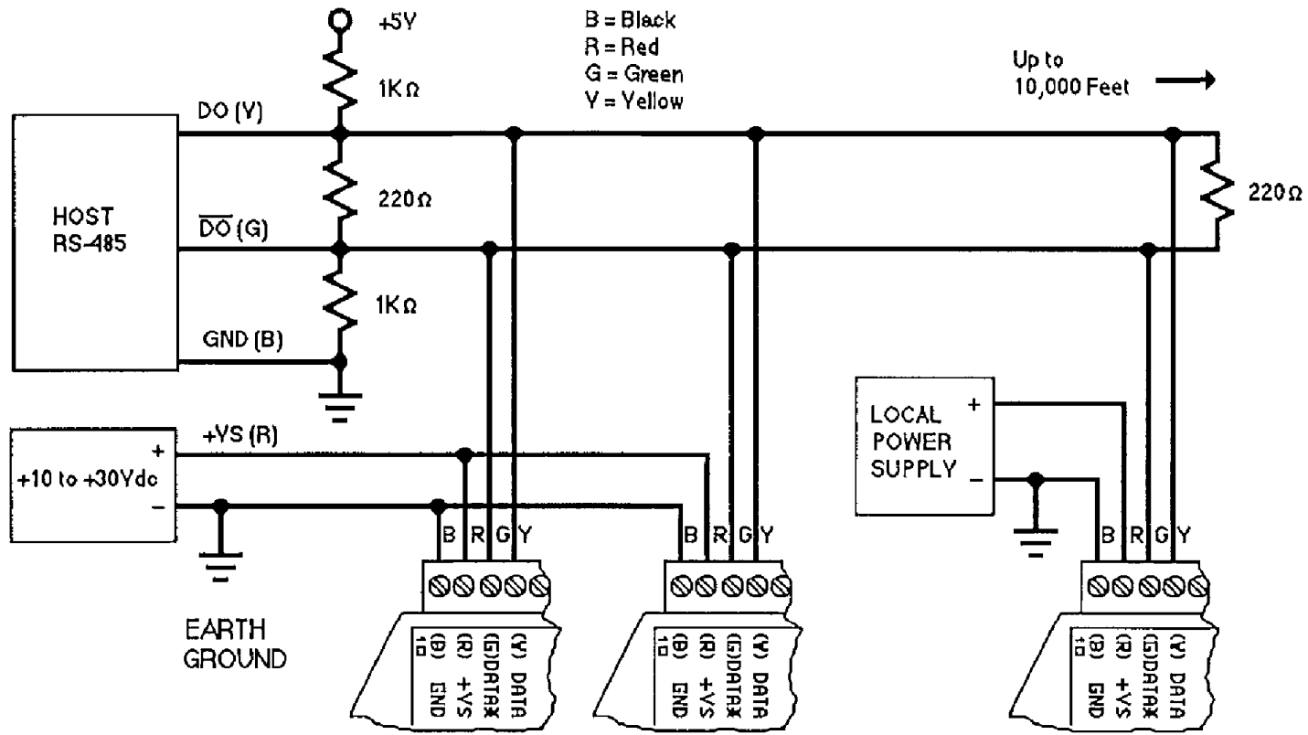
Figure 3.2 RS-485 Network.
