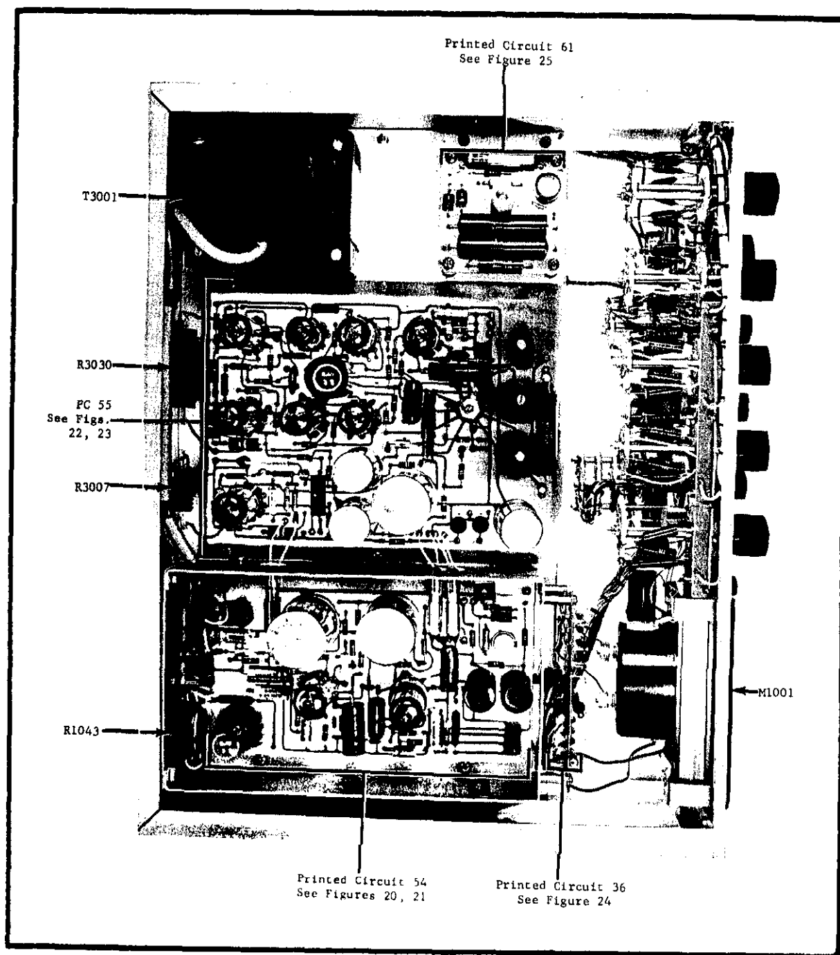
FIGURE 18. Top View of Model 660 Chassis. Location of components and printed circuits is shown above. Refer to Parts List for circuit designations.
