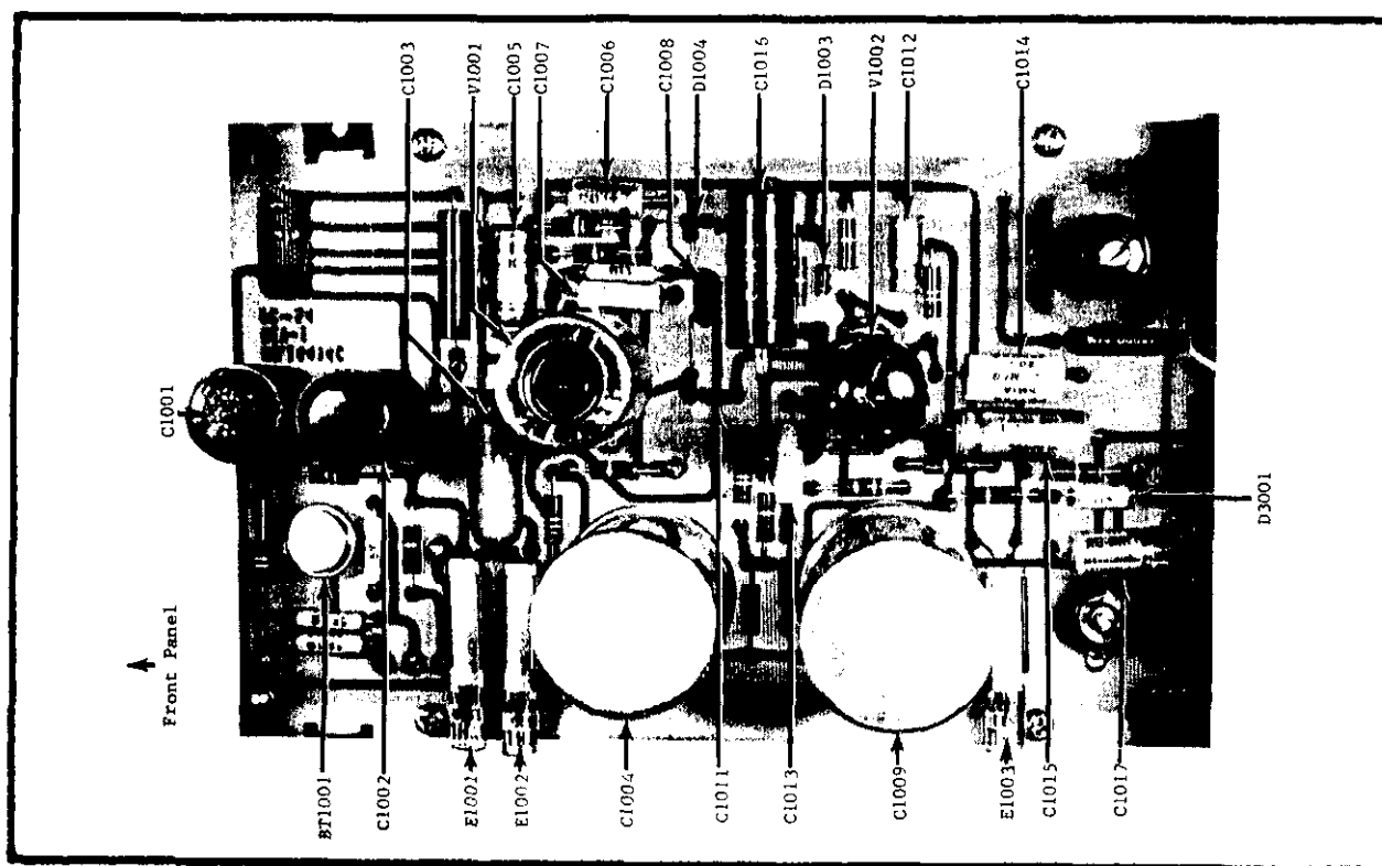
FIGURE 21. Battery, Capacitor, Modulator, Diode and Tube Locations on Printed Circuit 54. Resistors are shown in Figure 20.
