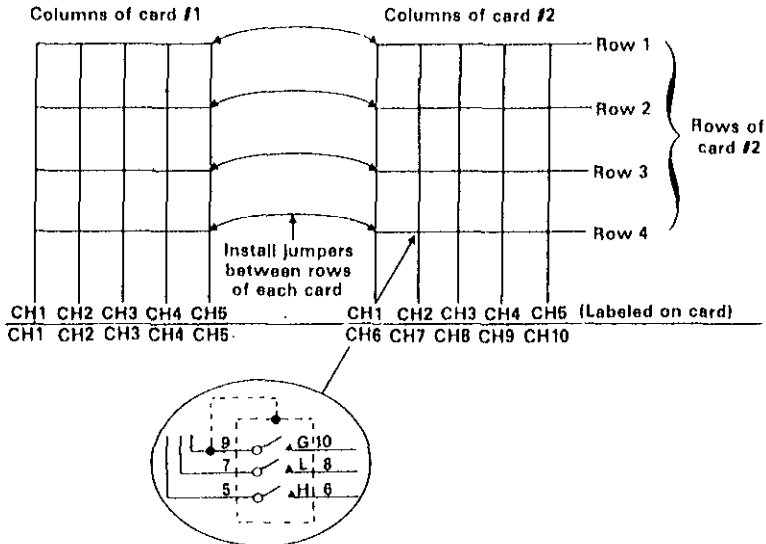
Each cross point in the matrix consists of a 3 pole Form A (normally open) relay as shown
