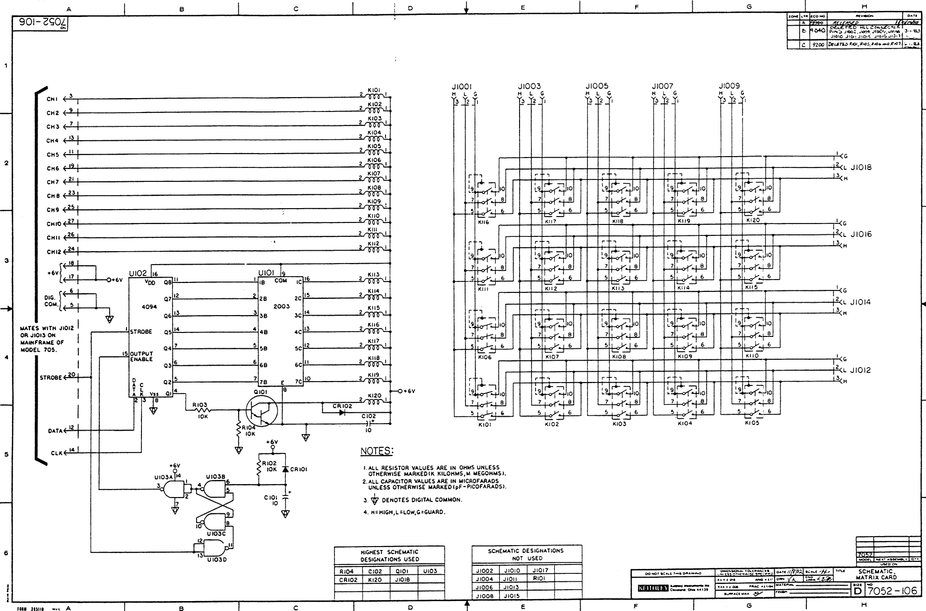
Figure 5. Model 7052 Schematic Diagram
