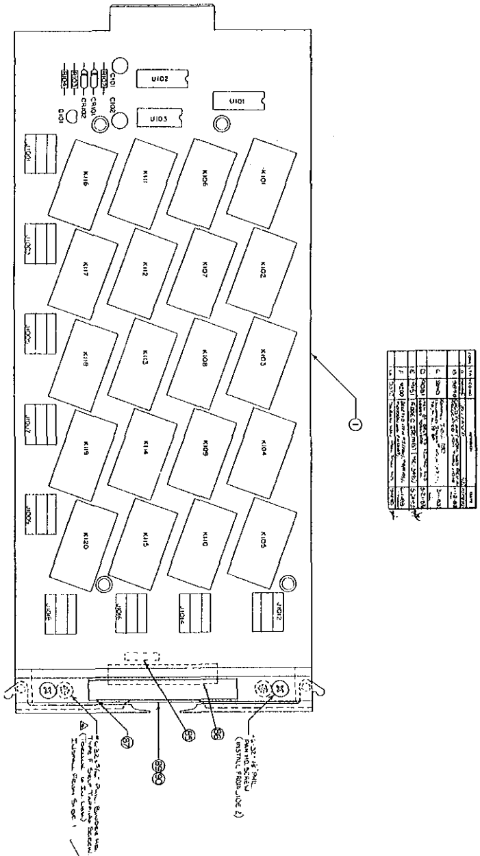
Figure 4. Model 7052 Component Layout
