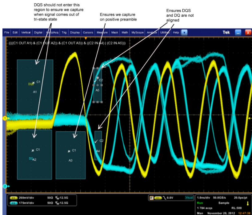
Figure 2: Write burst
