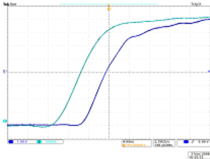
This shows a sample waveform prior to deskew.
