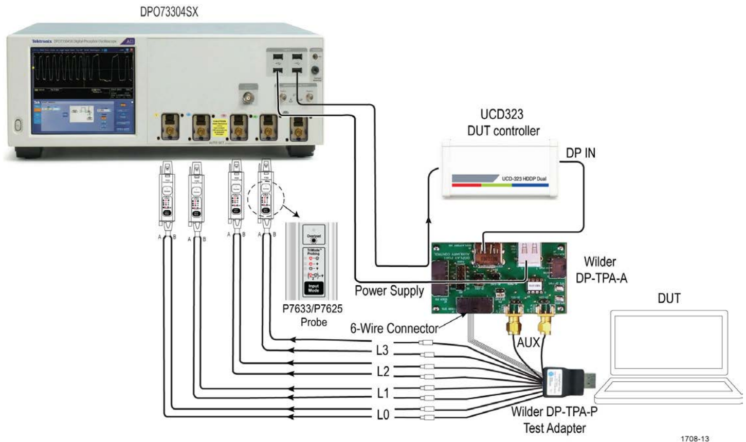
Connection diagram for testing Standard Connector
