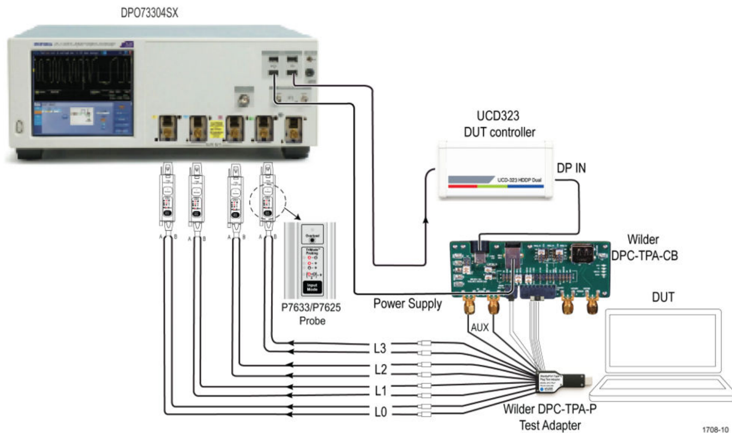
Connection diagram for testing Type-C Connector
