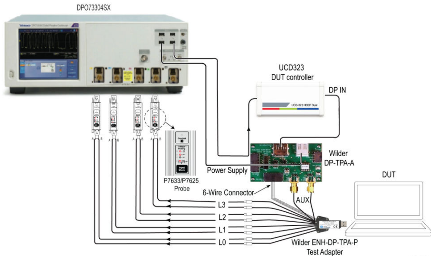
DisplayPort2.1 Standard Type – UCD323 DUT Control
