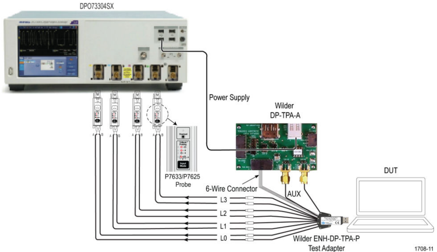
DisplayPort2.1 Standard Type – Manual DUT Control
