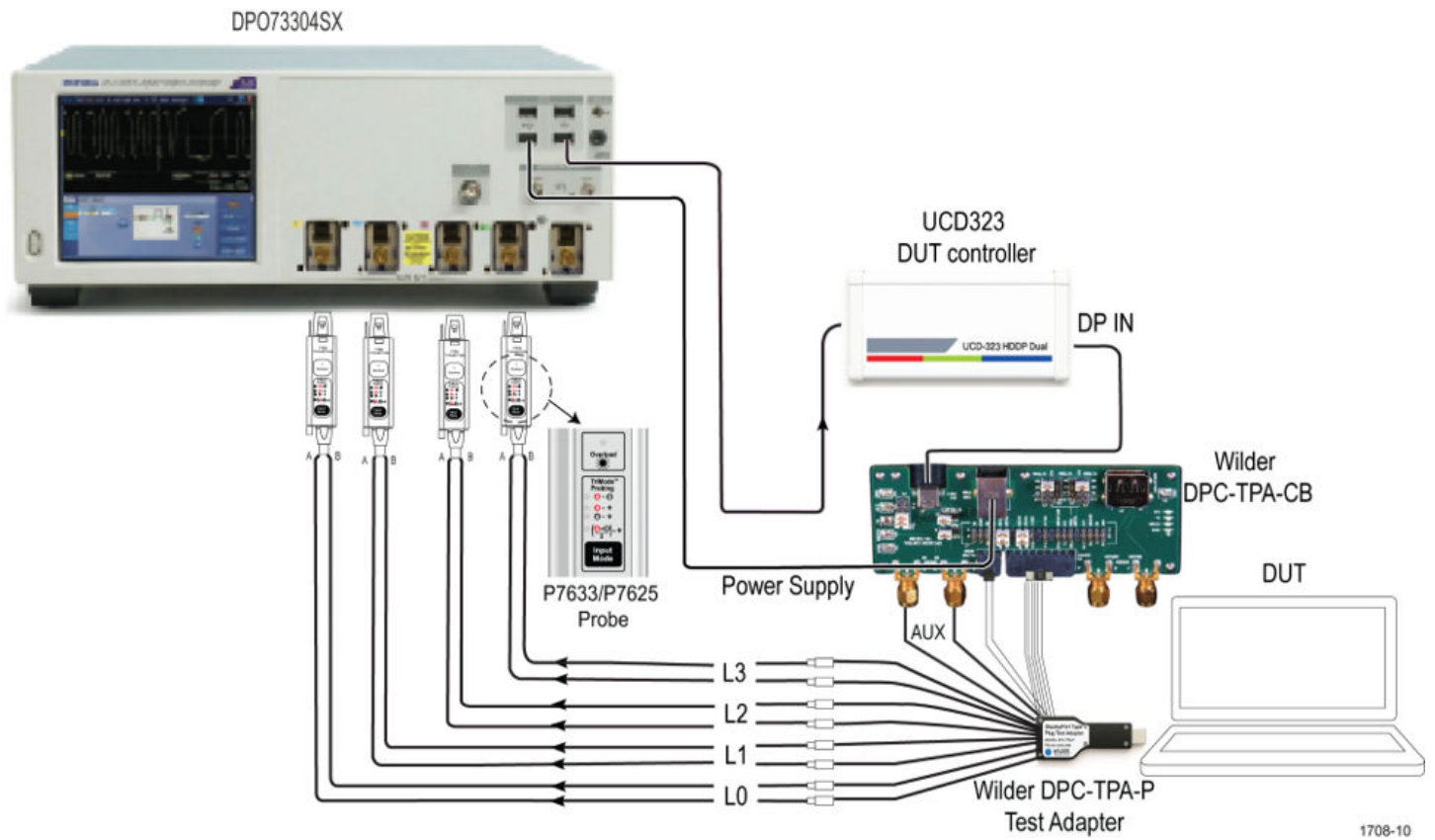
DisplayPort2.1 C-Type – UCD323 DUT Control
