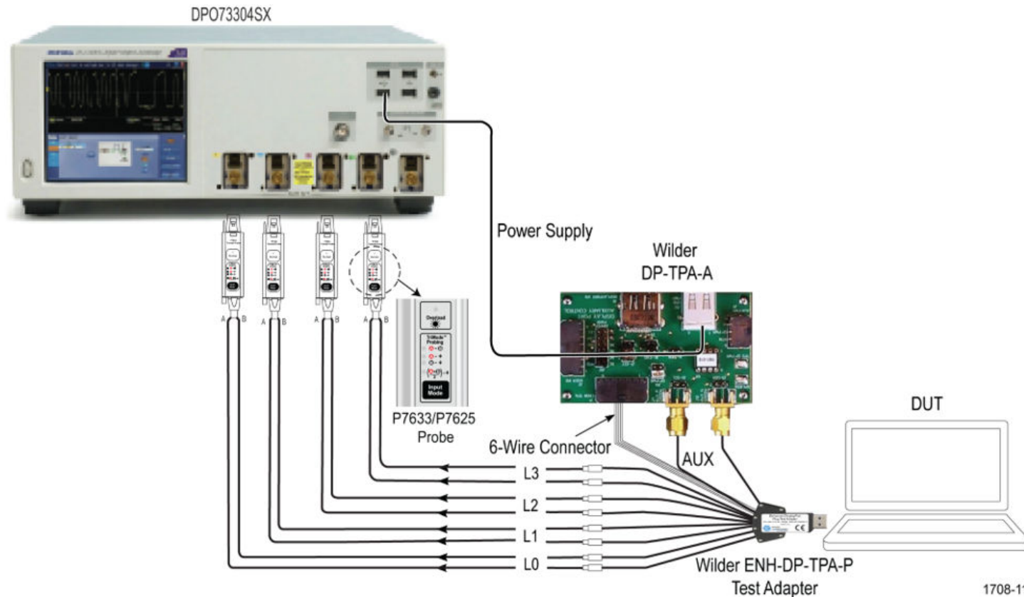
DisplayPort2.1 Standard Type – Manual DUT Control
