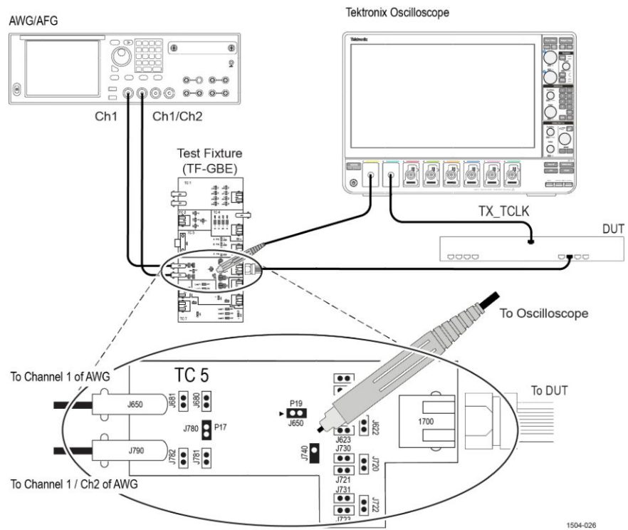
Figure 37: Master Filtered with Clock - Connection 2
