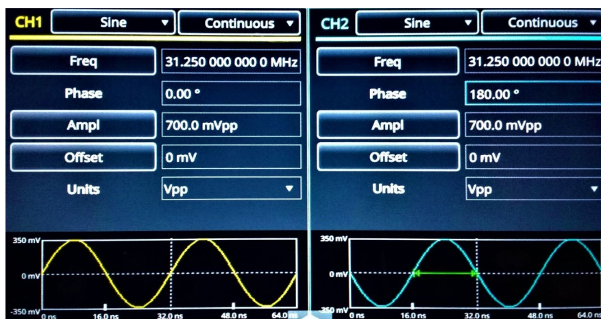
Figure 27: AFG with Test Mode 1 waveform loaded
