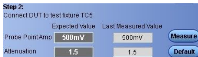
Figure 23: Test Fixture Compensation in JigMatch
