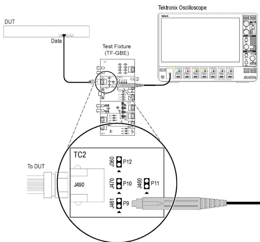
Figure 20: Connection diagram to measure linearities of Test Fixture using JigMatch
