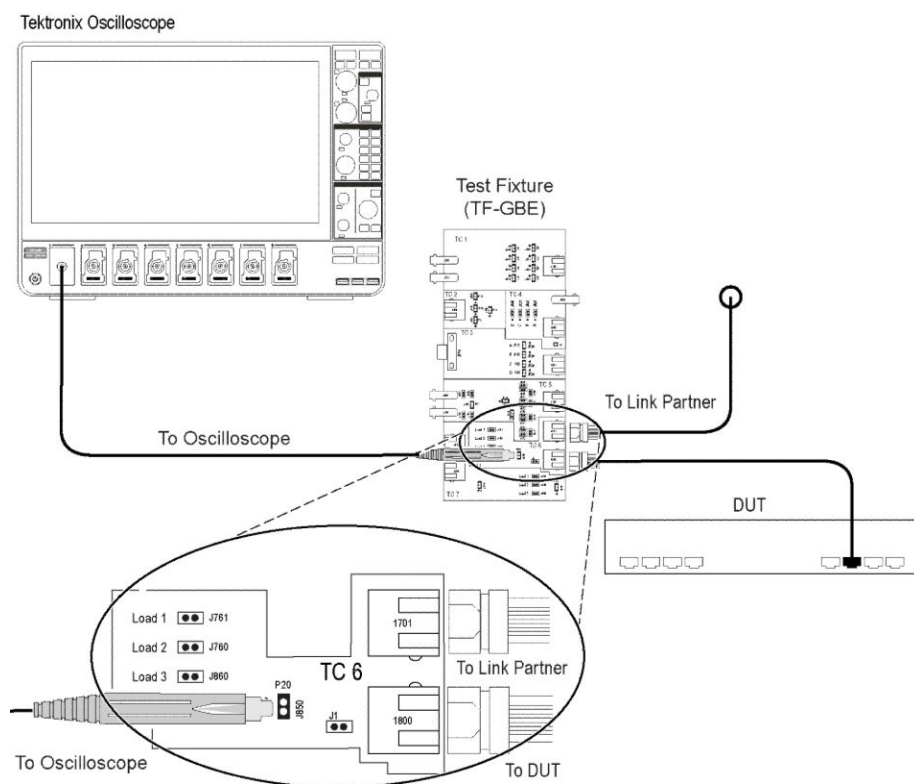
Figure 49: 10BASE-T TP_IDL Load Without TPM, Jitter, Link Pulse Load Without TPM, Harmonic, and Link Pulse Timing Without TPM , and Differential Voltage
