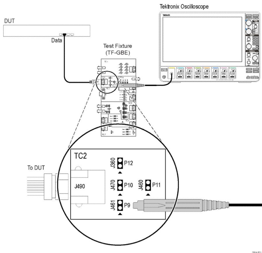
Figure 45: 100BASE-T connection diagram for all tests except Return Loss
