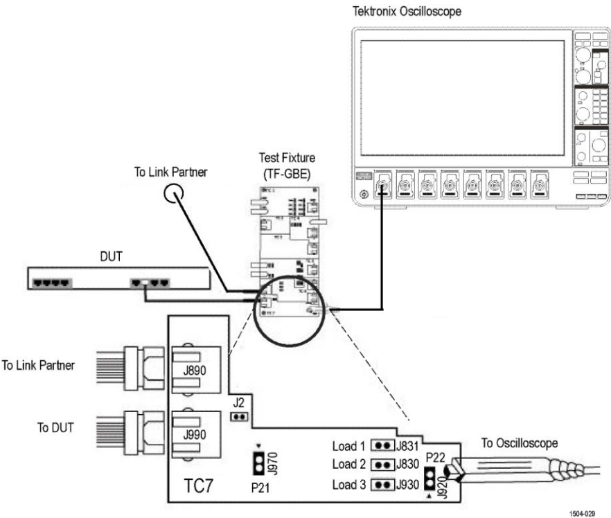
Figure 48: 10BASE-T MAU, Jitter, TP_IDL Load With TPM, Link Pulse Timing With TPM, and Link Pulse Load With TPM
