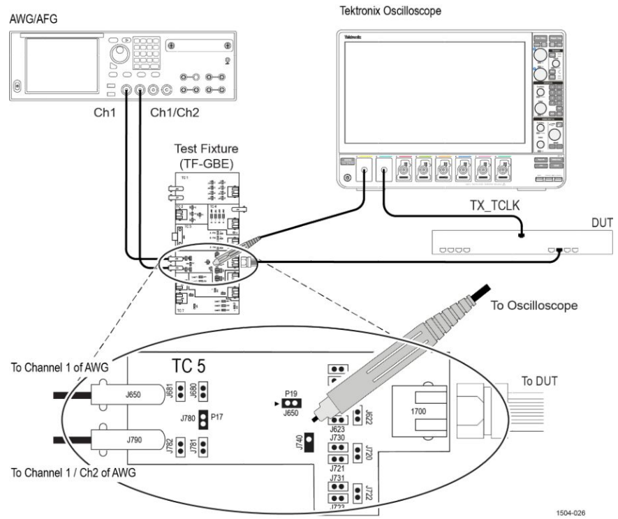
Figure 31: Distortion with Disturber with Clock
