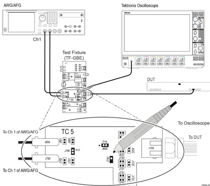
Figure 30: 1000BASE-T Template, Peak Volt, and Droop (With Disturber)
