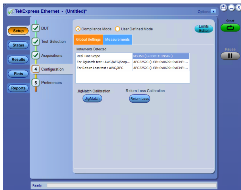
Figure 5: Configuration Panel to select Signal Source and to perform Return Loss Calibration
