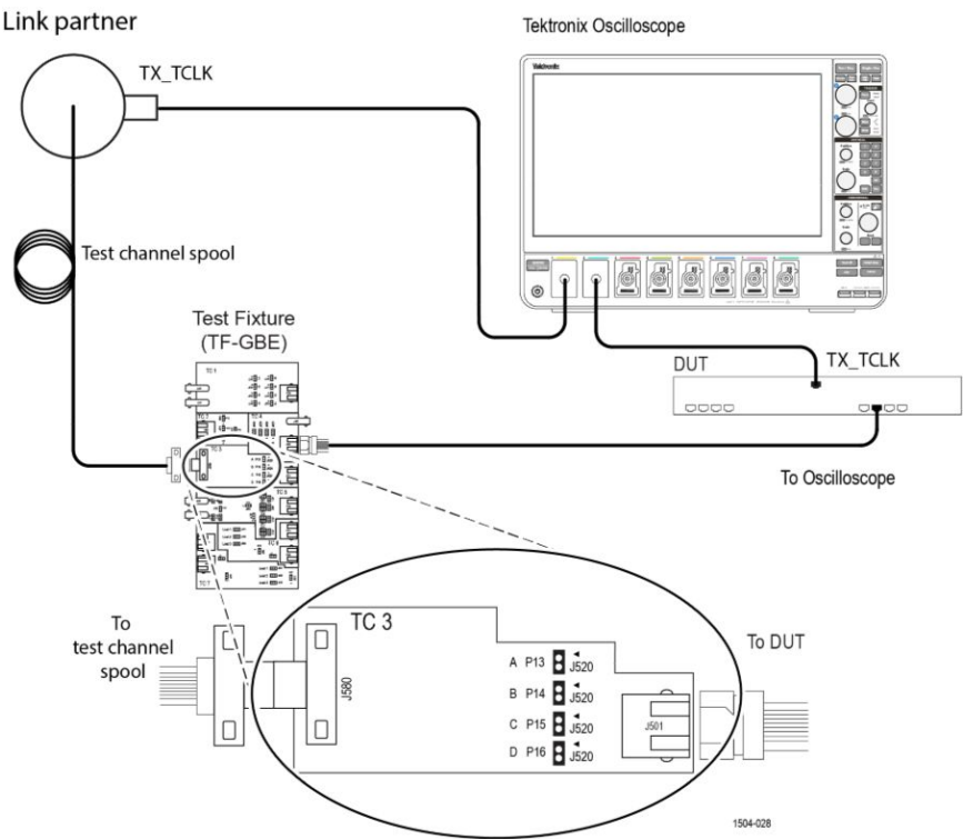
Figure 40: Slave Filtered with Clock - Connection 2
