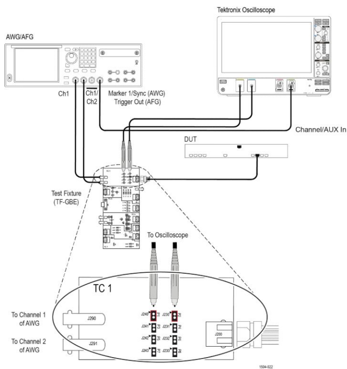
Figure 50: 10BASE-T Transmitter Return Loss
