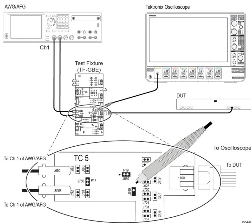
Figure 22: Connection diagram to measure linearities of the Test Fixture using JigMatch
