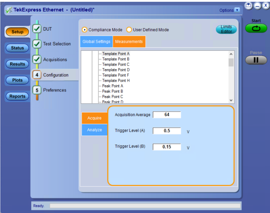
Figure 3: Configuration tab: Measurements Settings
