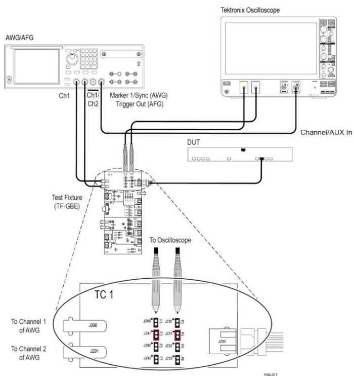
Figure 51: 10BASE-T Receiver Return Loss
