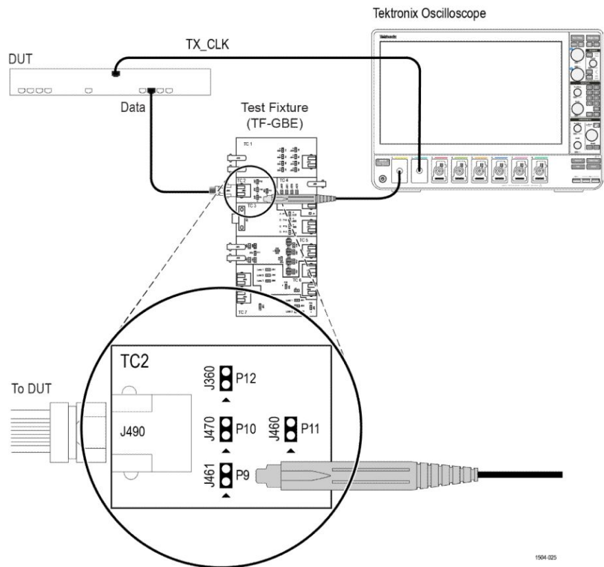
Figure 39: Slave Filtered with Clock - Connection 1
