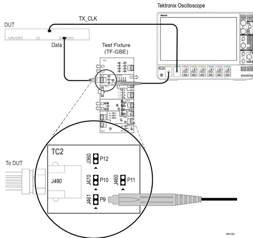
Figure 33: Distortion without Disturber with Clock
