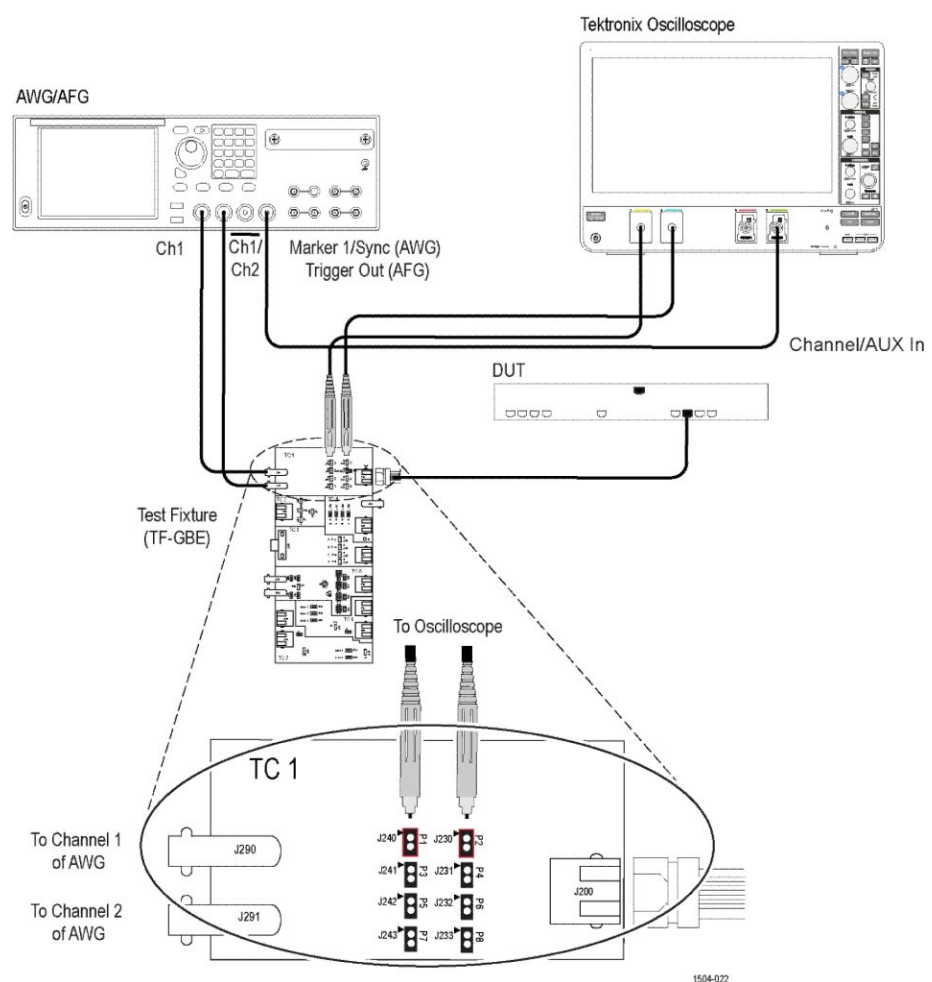
Figure 43: 1000BASE-T Transmitter Return Loss
