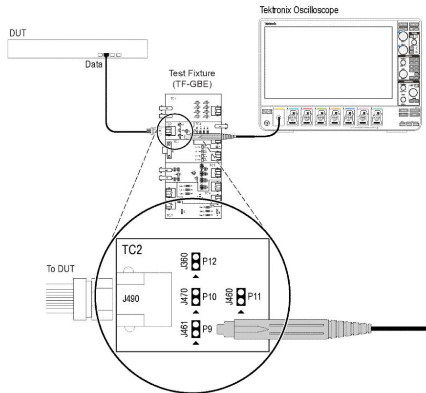
Figure 29: 1000BASE-T Template, Peak Volt, and Droop (Without Disturber)
