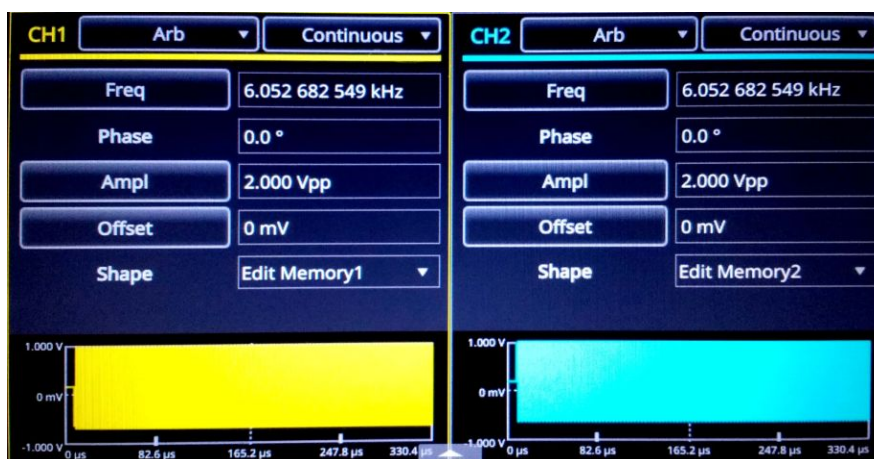
Figure 16: AFG with Return Loss waveforms loaded
