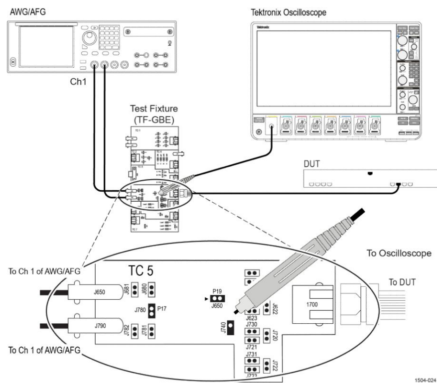
Figure 32: Distortion with Disturber without Clock
