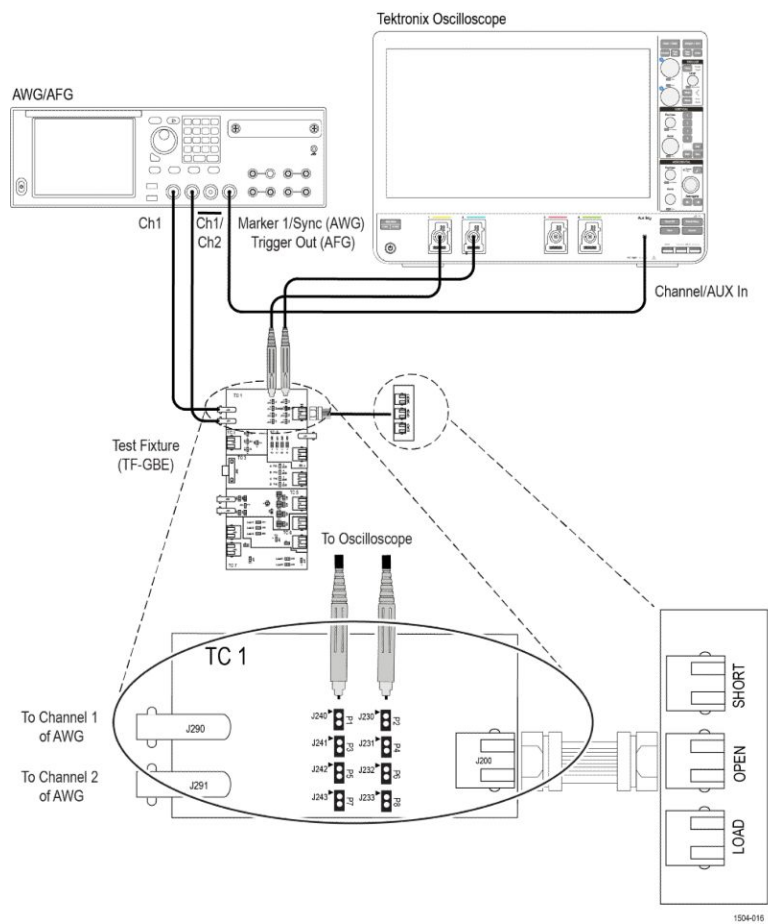
Figure 10: Connection diagram for OPEN Calibration
