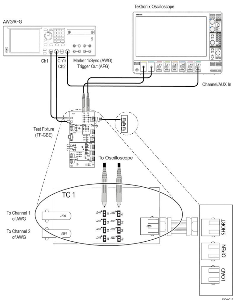
Figure 4: Connection diagram for SHORT Calibration
