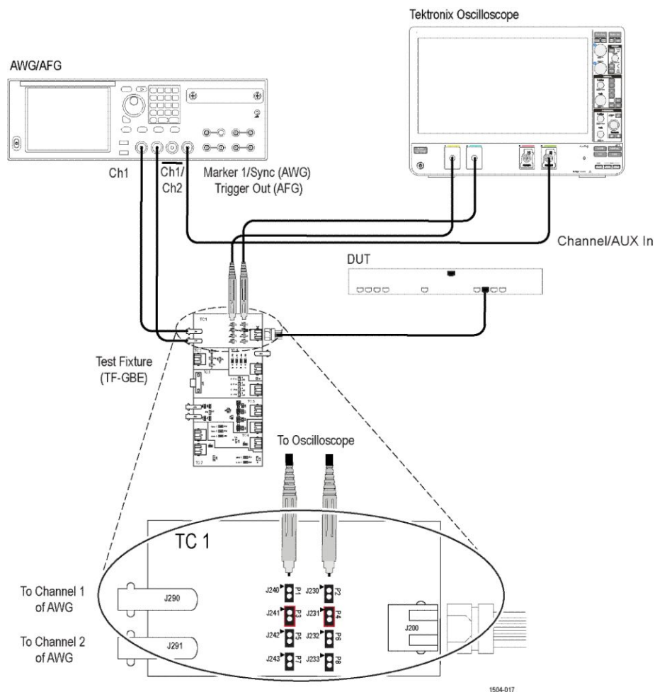
Figure 44: 1000BASE-T Receiver Return Loss
