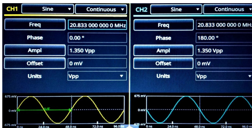
Figure 28: AFG with Test Mode 4 waveform loaded
