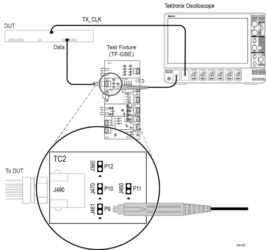
Figure 38: Master Unfiltered with Clock
