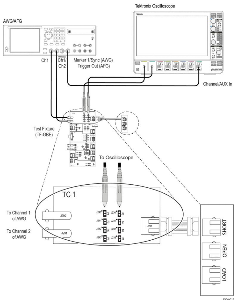
Figure 8: Connection diagram for SHORT Calibration
