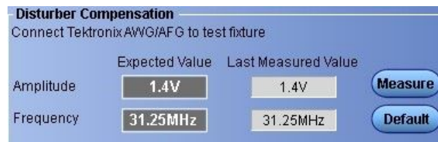
Figure 19: Disturber Compensation in JigMatch
