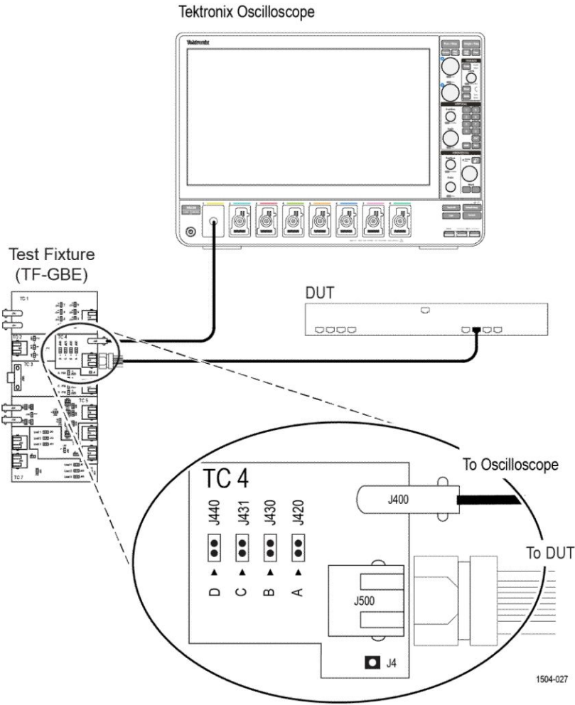
Figure 42: 1000BASE-T CM Voltage
