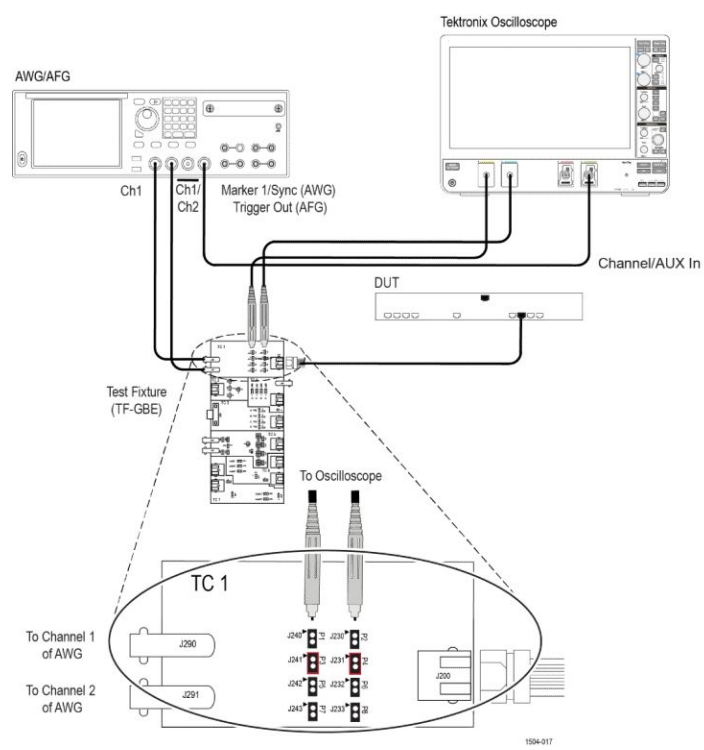
Figure 47: 100BASE-T Receiver Return Loss
